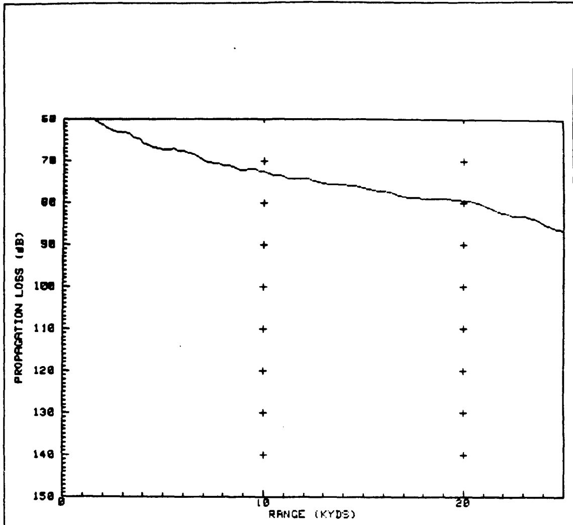
Range Independent (RI) Plot for Event 10115, Run 1, 25'R. The RI prediction was not able to accurately reproduce propagation losses predicted in the measured data. The RI prediction (no bottom bounce) was not comparable to MAPS.
