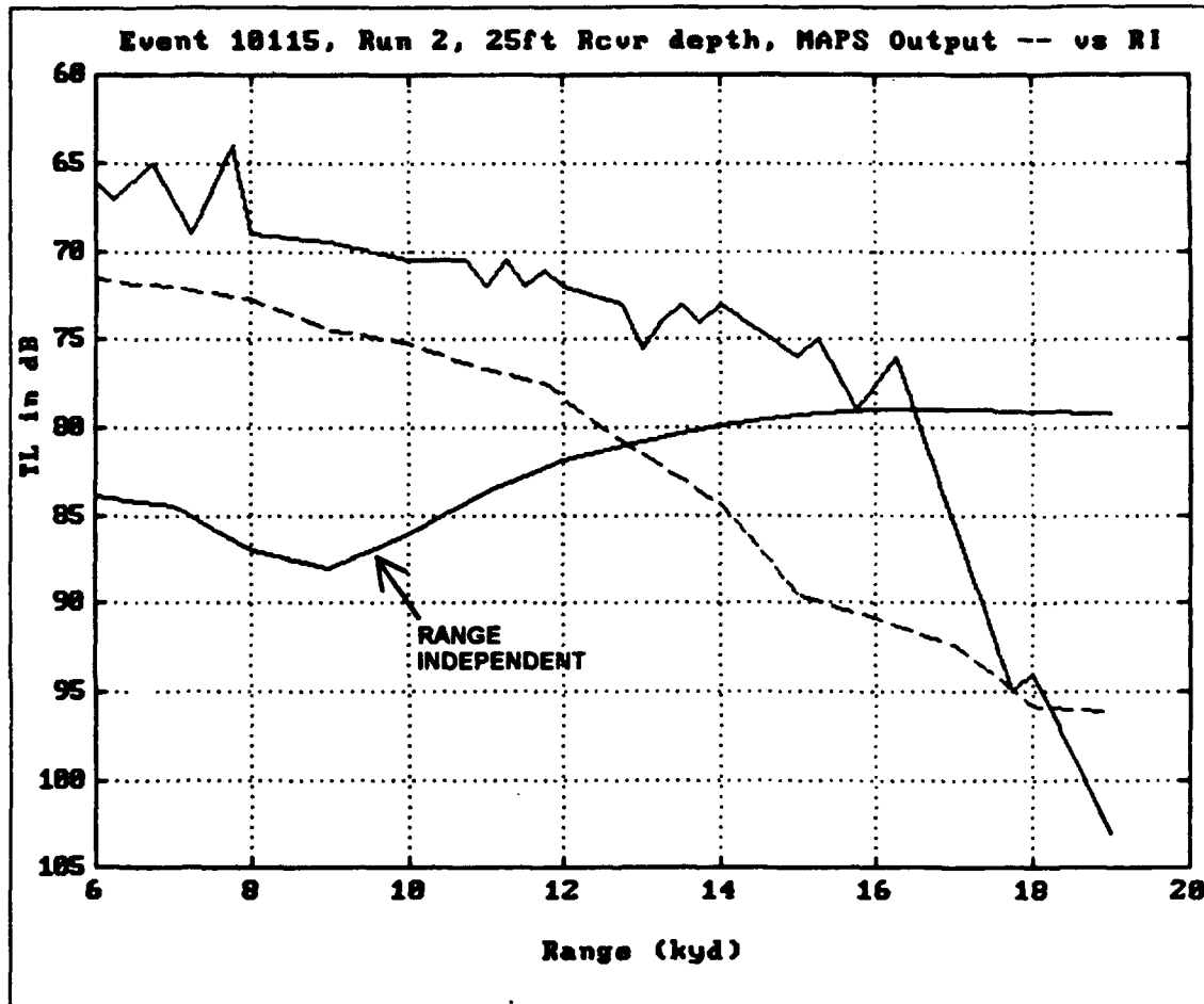
Figure 28. Comparison for Event 10115, Run 2, 25'R
