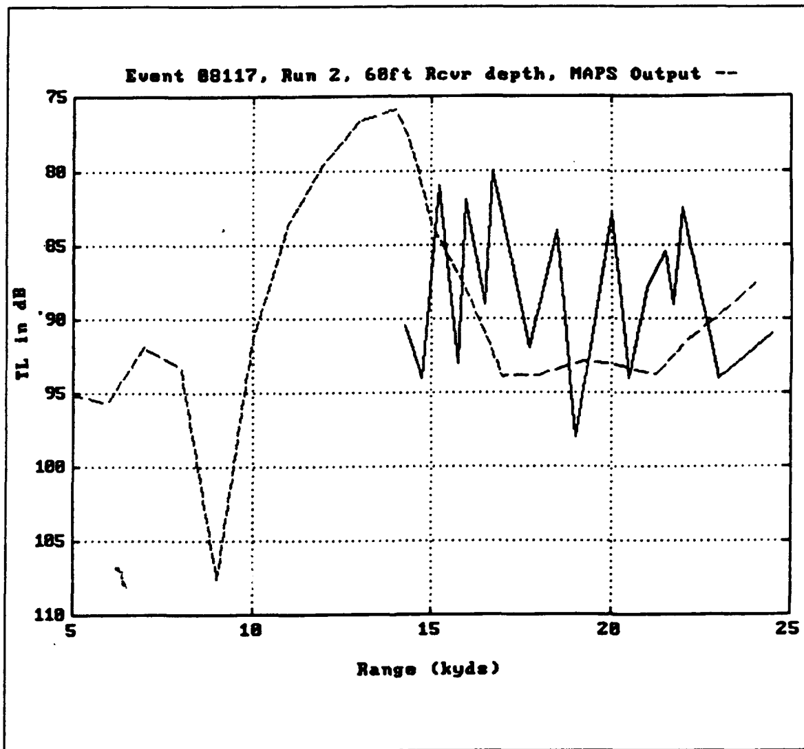
Figure 21. Comparison for Event 08117, Run 2, 60'R
