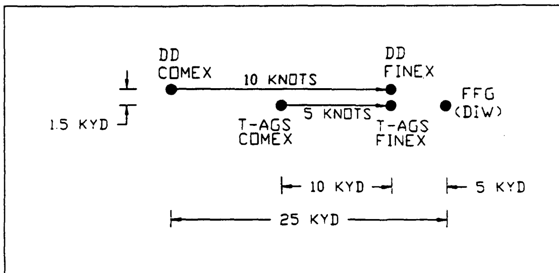
Figure 16. 3 Ship Geometry
