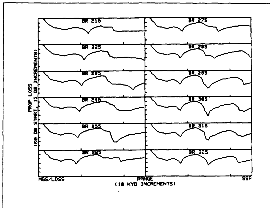
Figure 11. Twelve Beam Propagation Loss
