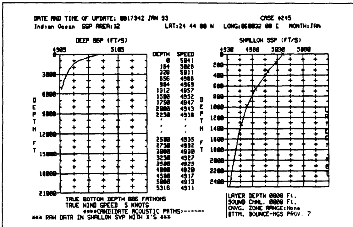
Figure 10. XBT Presentation
