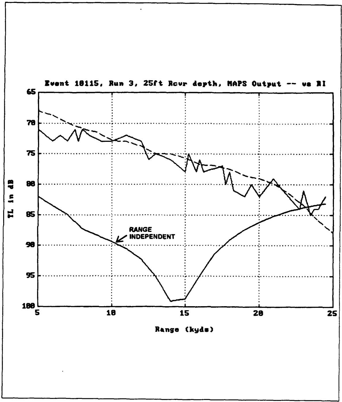
Figure 31. Comparison for Event 10115, Run 3, 25'R
