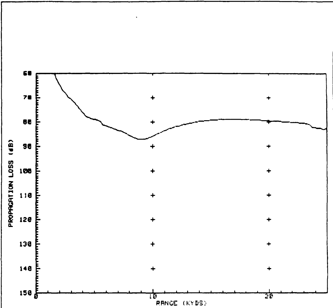
Range Independent (RI) Plot for Event 10115, Run 2, 60'R. The RI prediction does not reproduce the 17 kyd loss of sound energy. The RI prediction was 20 dB lower loss than MAPS prediction.
