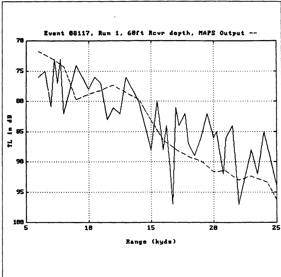
Figure 19. Comparison for Event 08117, Run 1, 60'R formed surface duct with a layer depth of 300 ft. MAPS produces an accurate reproduction of the measured data to the 17 kyd point. At the 17 kyd point MAPS is showing approximately 5 dB more propagation loss that was experienced in the experiment.
