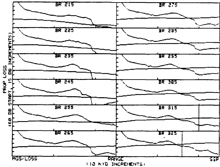
Event 08117, Run 2, 60'R with MGS province 7 used.
