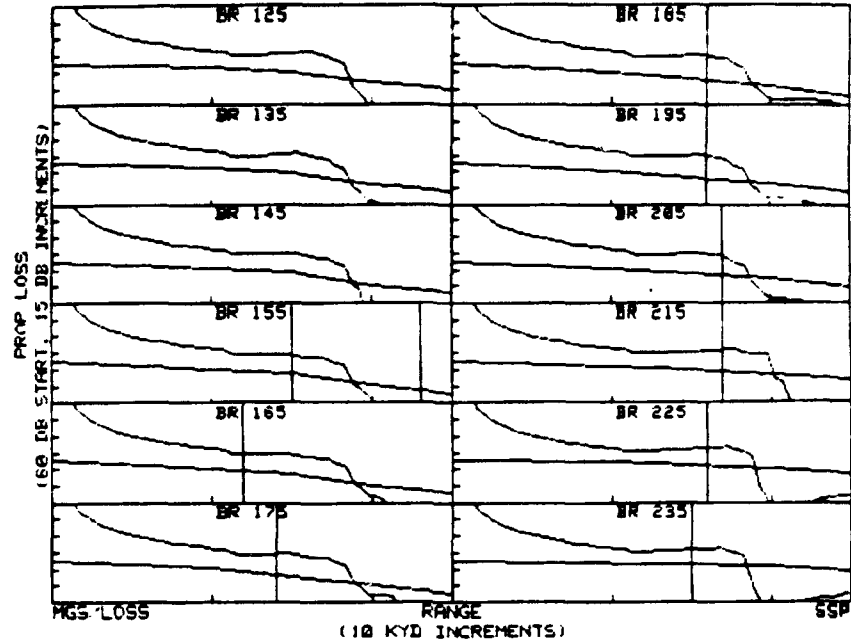
Event 08117, Run 1, 60'R with MGS province 7 used.
