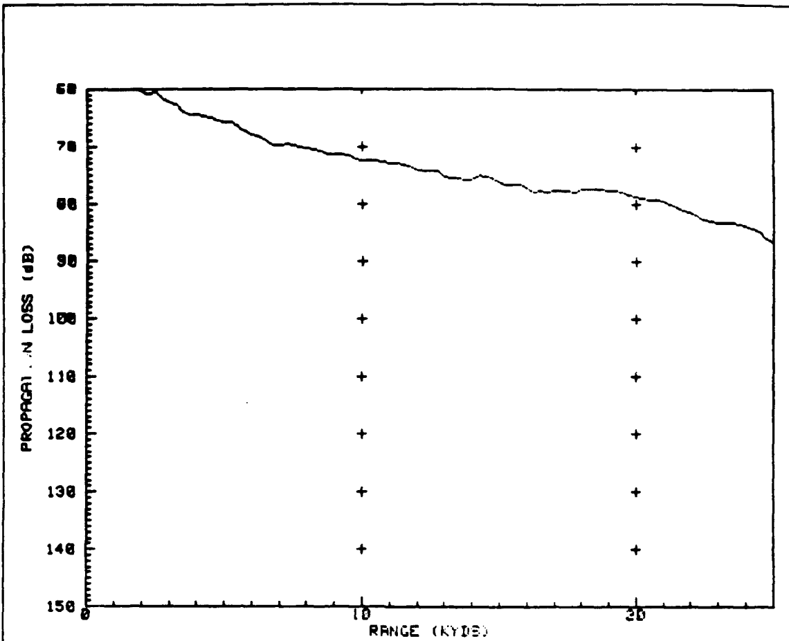
Range Independent (RI) Plot for Event 08117, Run 2, 25'R. The RI prediction was 3 to 5 dB lower loss than the measured data. The RI prediction and MAPS were almost identical.
