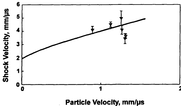
Figure 30: Hugoniot measurements for Lexan from impact experiments using a Lexan flyer with a thin facing material ( 35\text{ }\mu\text{m} thick aluminium foil). The solid line is from published data [6].
