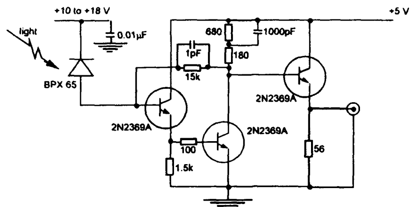
Figure 13: Photodetector circuit No.2.
