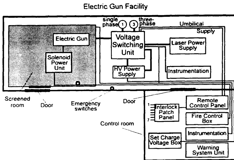
Figure 3: The electric gun facility and control room.
