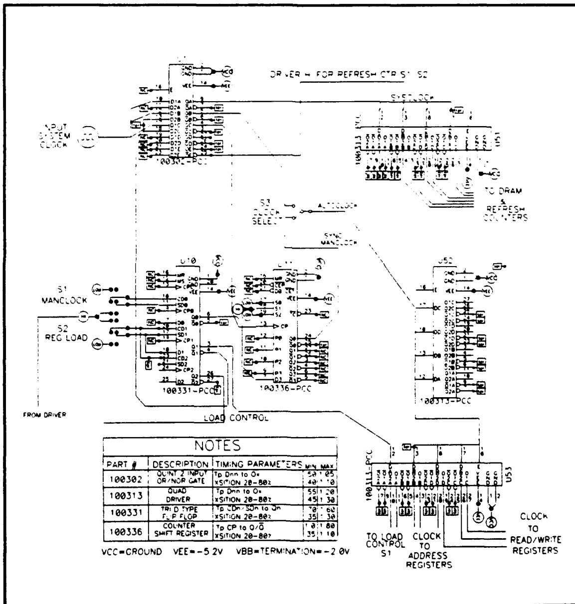
Figure 2-8 Manual Clock and Drivers
