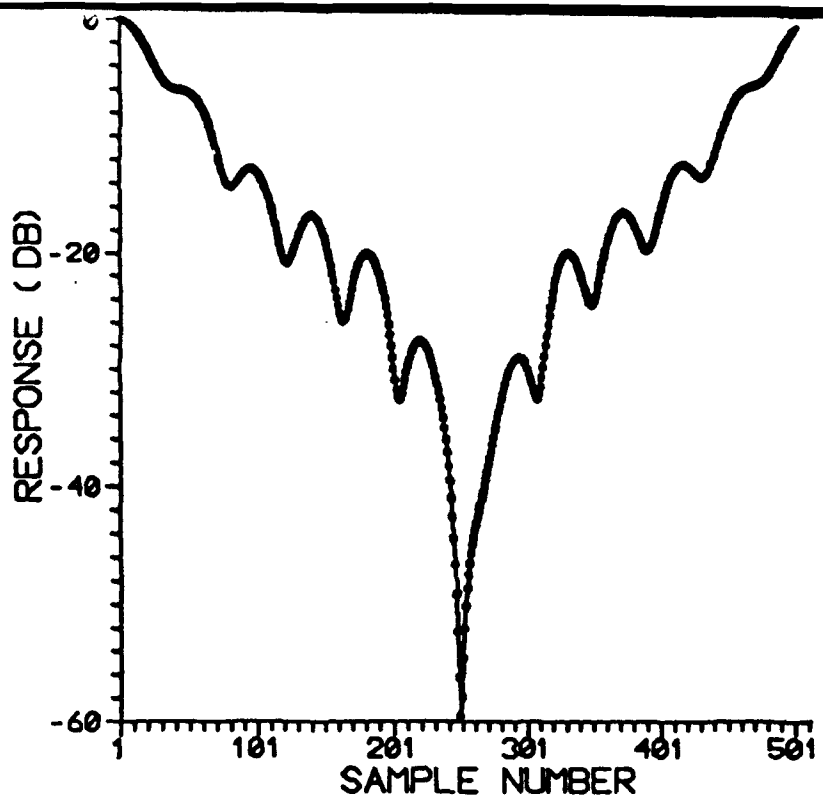
Fig. 18 The spectrum of reconstructed signal (obtained from Figs. 13 and 14)
