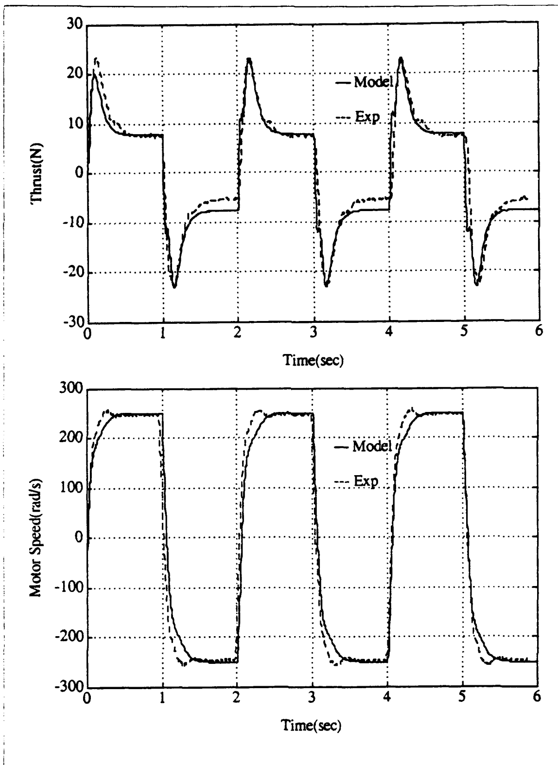
Figure 3.2 Square Wave, 2 Sec Period, Motor Voltage \pm 20.4 v
