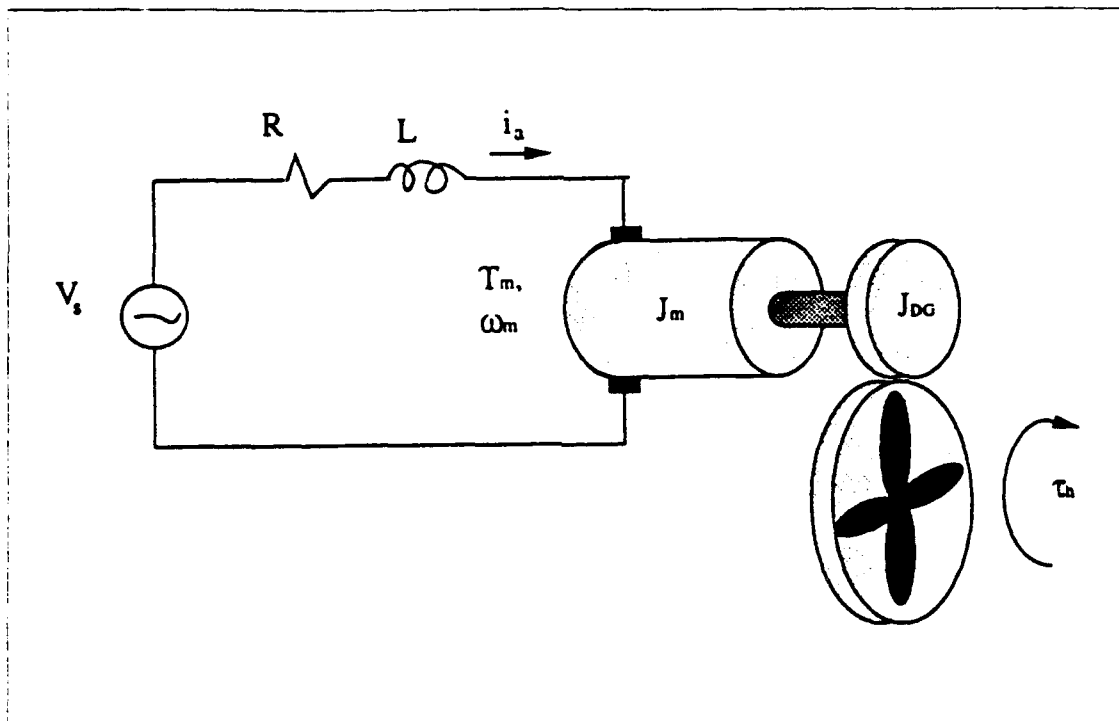
Figure 2.2 Electric/Mechanical Schematic
