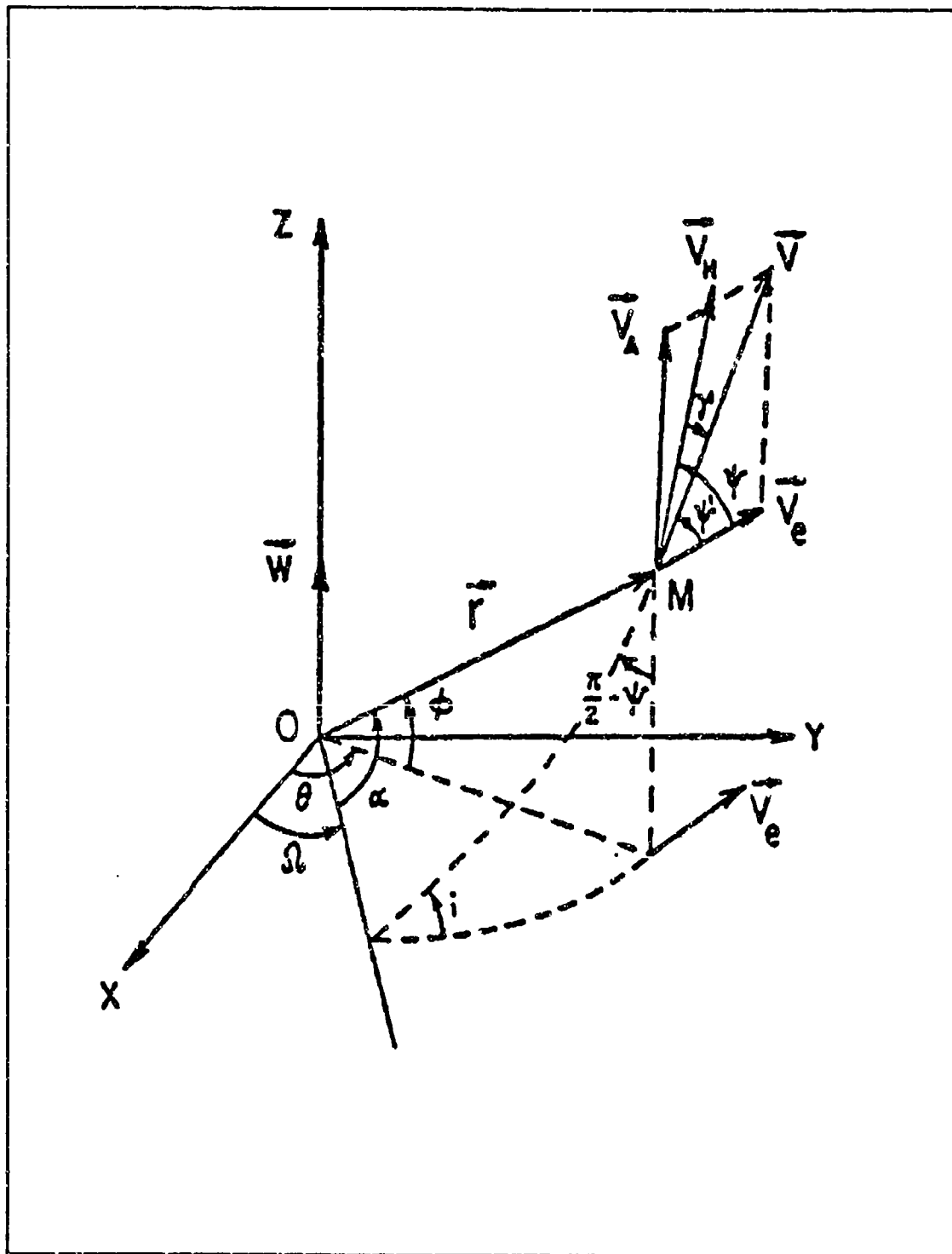
Figure 20: Coordinate System And Nomenclature [Ref. 41]
