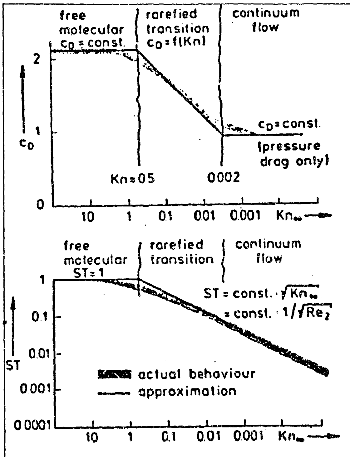
Figure 31: Aerodynamic Coefficients In The Flow Regimes [Ref. 76]
