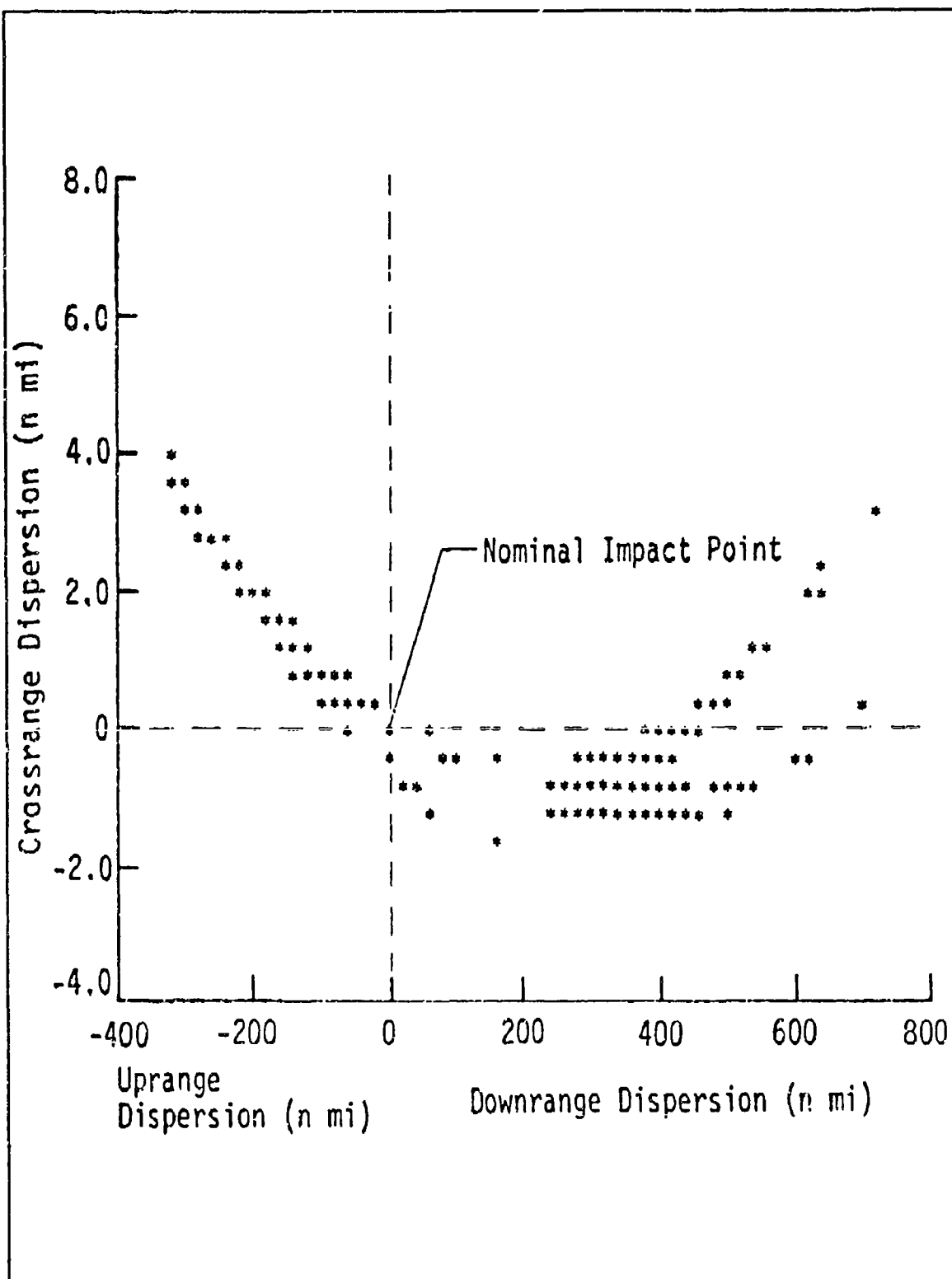
Figure 65: Down Range And Crossrange Dispersions [Ref. 45]
