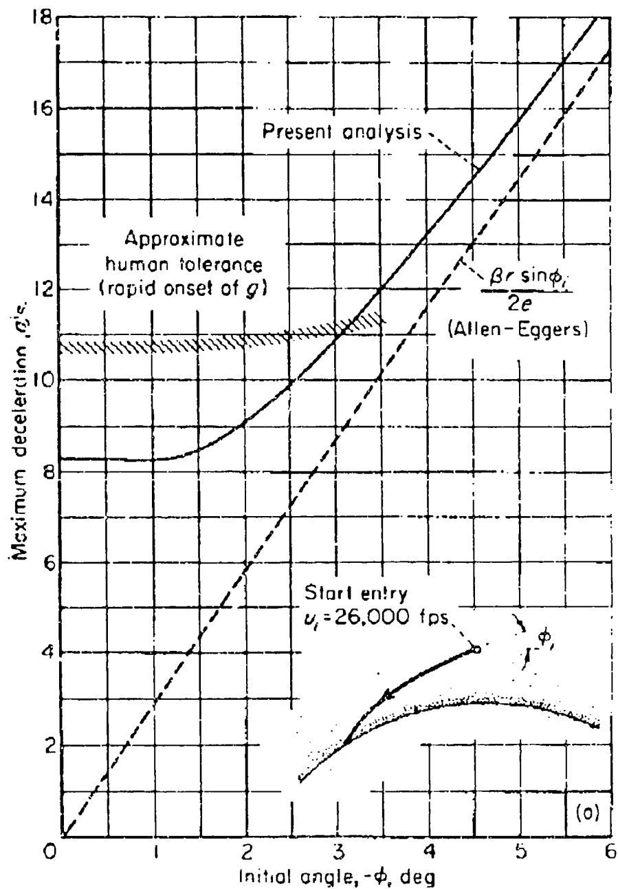
Figure 13: Maximum Deceleration vs Initial Flight Path Angle [Ref. 14]
