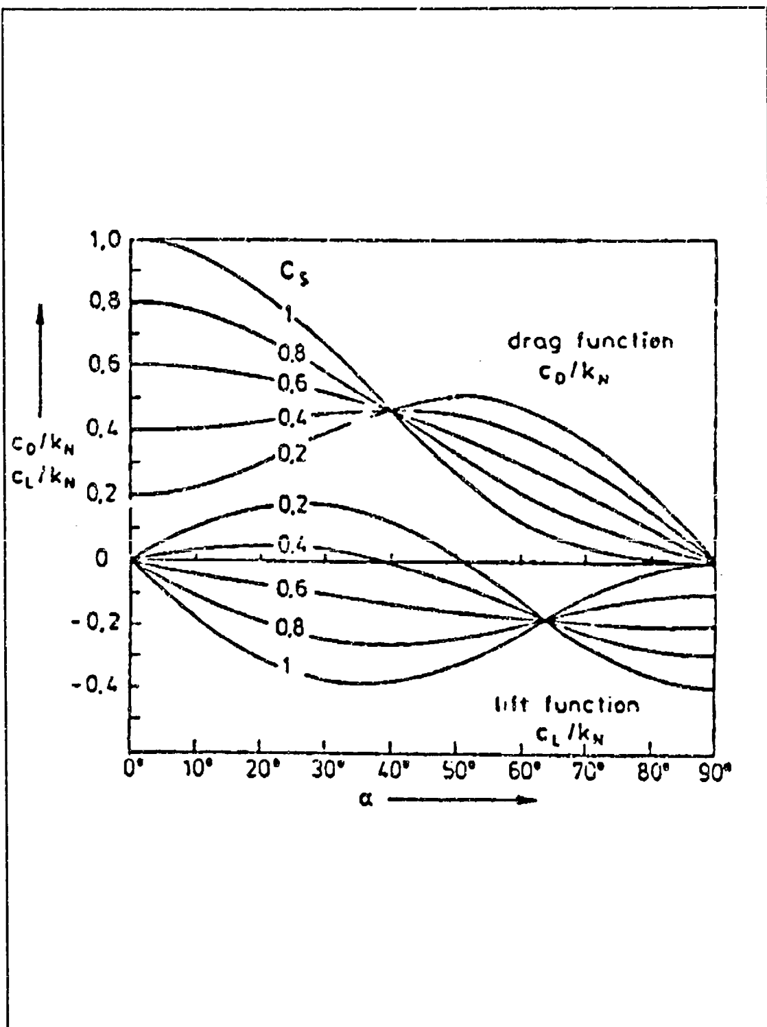
Figure 34: Newtonian Lift And Drag Functions [Ref. 76]
