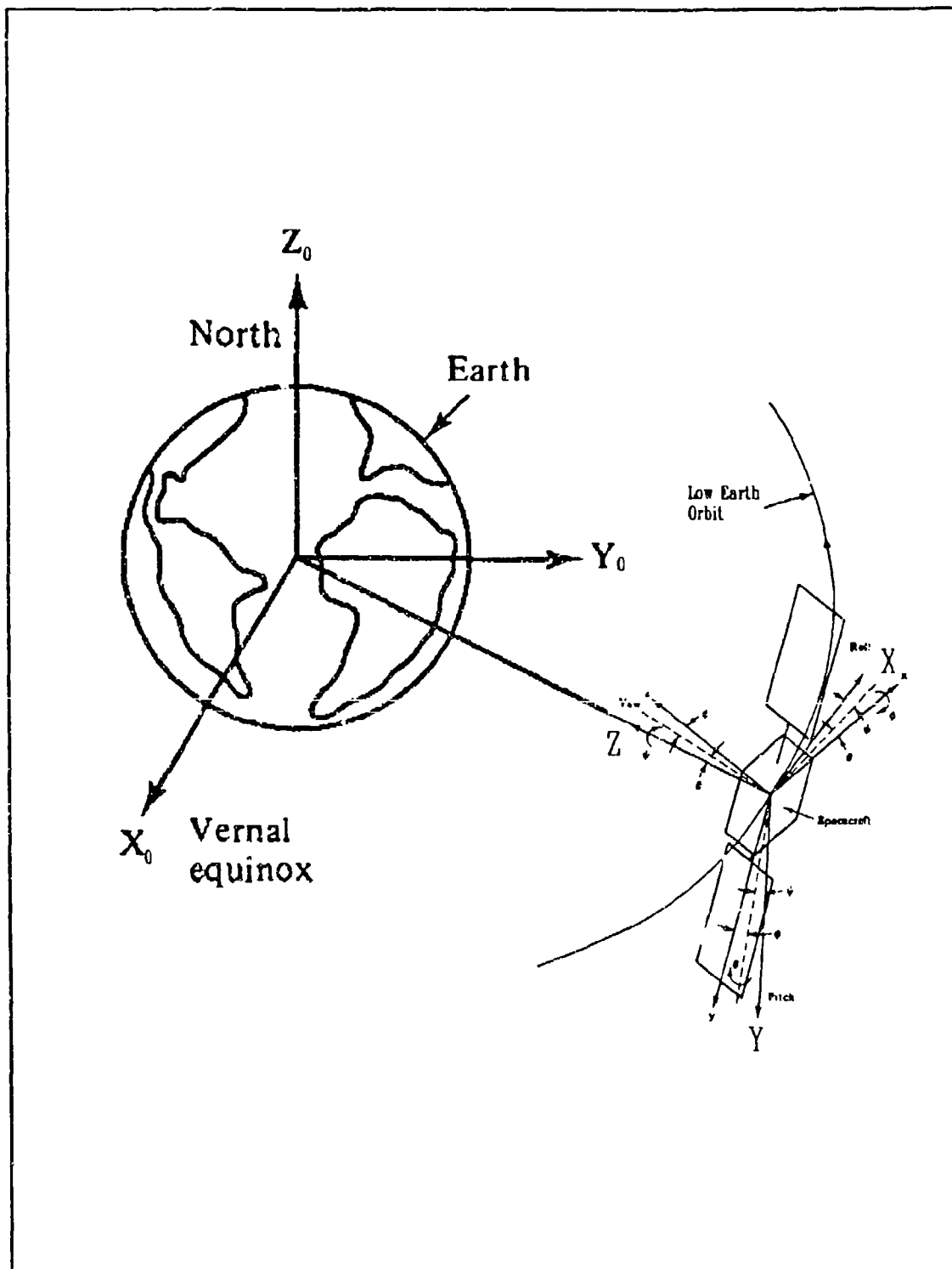
Figure 25: Attitude Dynamics Coordinate System [Ref. 57]
