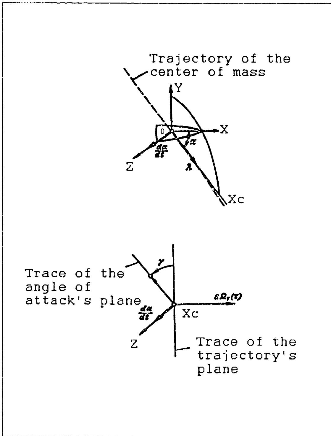
Figure 27: Reentry Body Coordinate System [Ref. 56]
