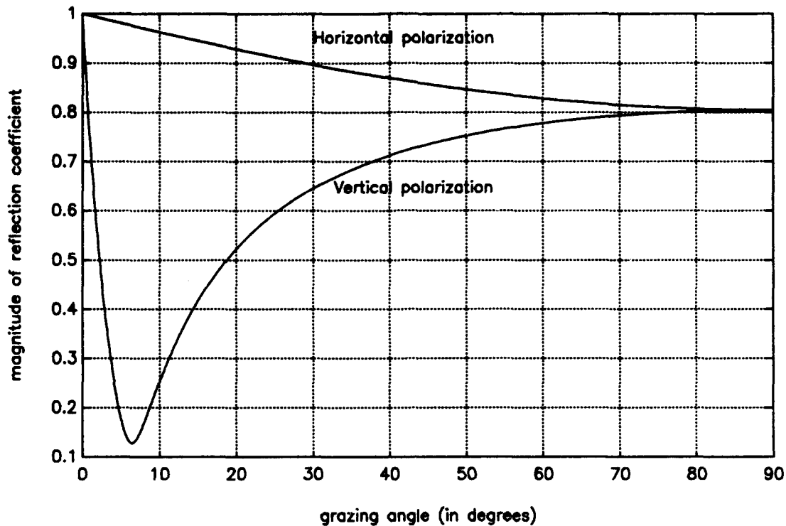
Figure 2.2 The Magnitude of the Reflection Coefficients for \epsilon' = 69 , \epsilon'' = 39 .
