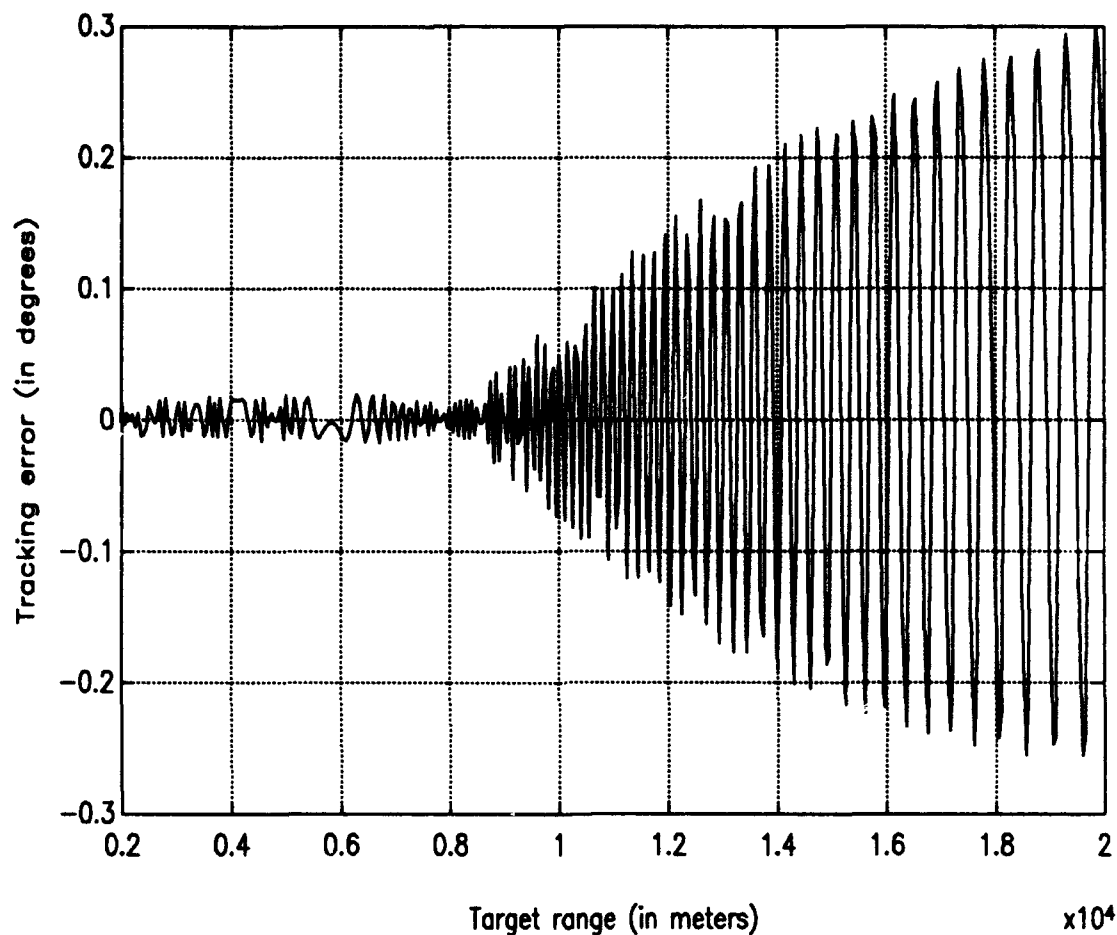
Figure 4.3 Tracking Error Calculated for f=9 GHz, h_2=150 m, h_1=15 m, \rho=0.9 , N=90 , d=0.5\lambda . Low Sidelobe Beams.
