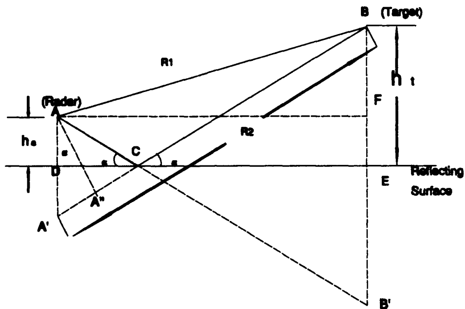
Figure 2.4 Geometry of Earth's Specular Reflection Model.
