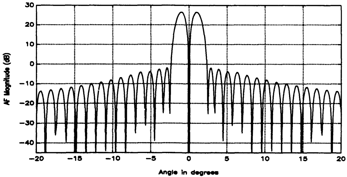
Figure 3.6 Bayliss difference pattern for an array 90 elements, d=0.5\lambda and \bar{n}=5 .
