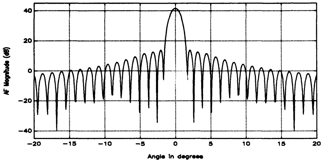
Figure 3.5 Taylor Sum Pattern of a 90 Element Array, d=0.5\lambda and \bar{n}=5 .
