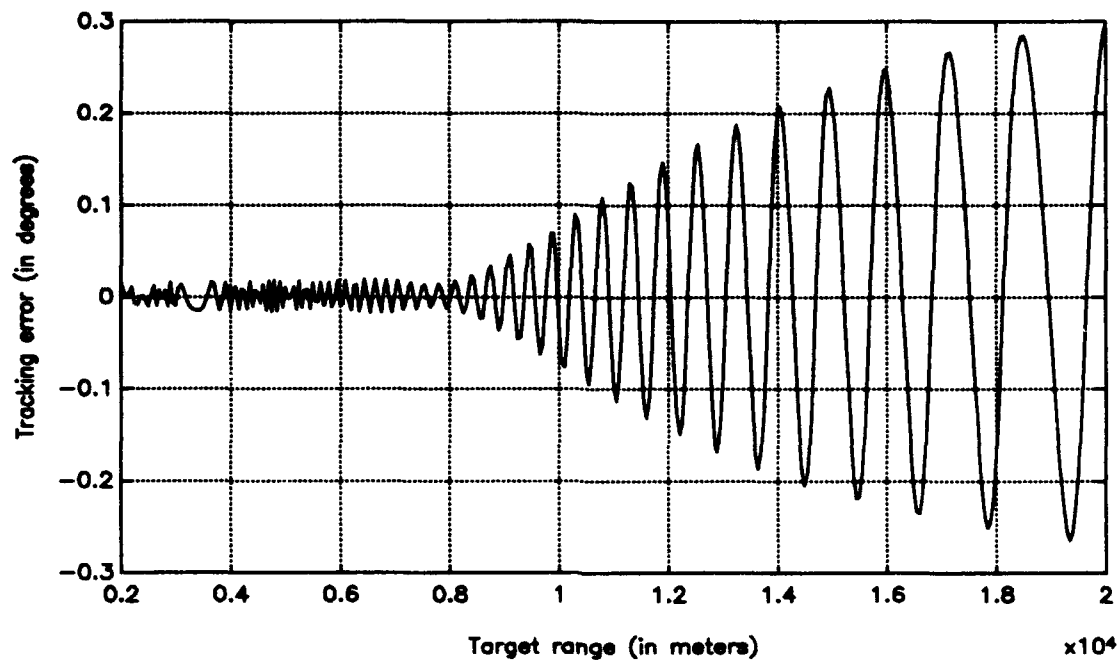
Figure 4.4 Tracking Error Calculated for f=3 GHz, h_2=150 m, h_1=15 m, \rho=0.9 , N=90 , d=0.5\lambda . Low Sidelobe Beams.
