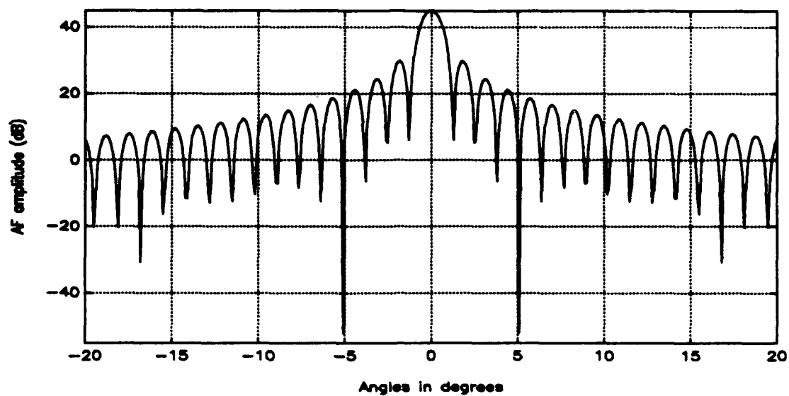
Figure 3.3 Uniform Distribution Sum Pattern for a 90 Element Array with d=0.5\lambda .
