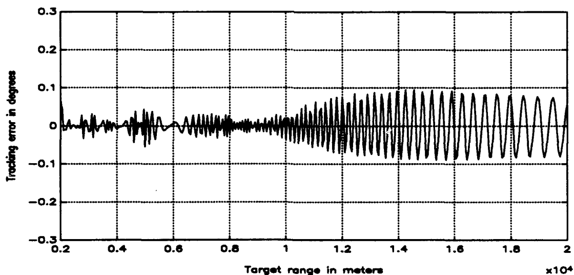
Figure 5.5 Reduced Tracking Error Using Difference Beam Phase Toggling for Uniform Antenna Coefficients. Same Parameters as in Figure 4.3.
