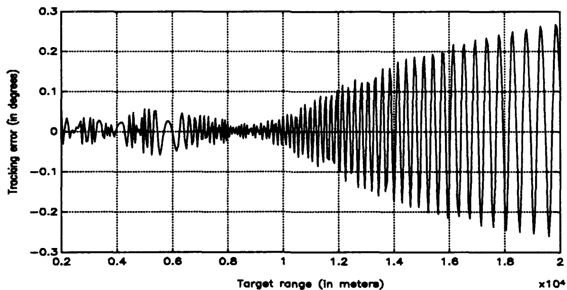
Figure 4.5 Tracking Error Calculated for f=9 GHz, h_2=150 m, h_1=15 m, \rho=0.9 , N=90 , d=0.5\lambda . Uniform Amplitude Beams.
