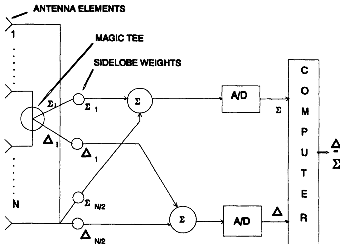
Figure 4.1 Monopulse Processor Simulation Model.
