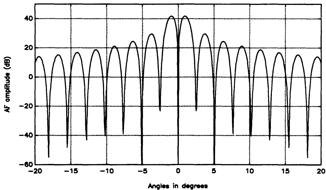
Figure 3.4 Uniform Distribution Difference Pattern for a 90 Element Array with d=0.5\lambda .
