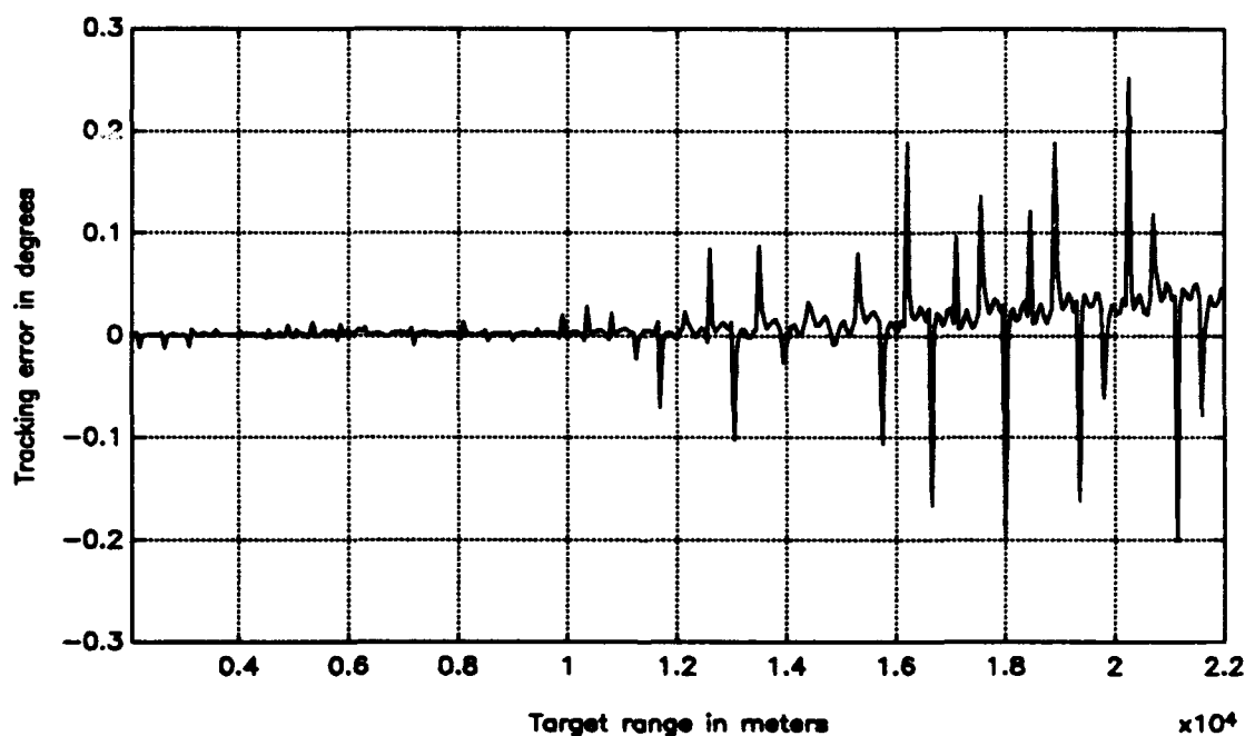
Figure 5.1 Reduced Tracking Error Using Uniform Coefficients. Frequency Agility with 20 Frequencies in 10 MHz Increments and Averaging of Error Method is Used. Same Parameters as in Figure 4.3.
