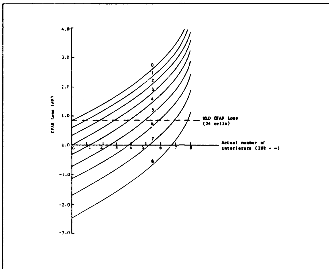
Figure 47. CFAR Loss for CMLD
