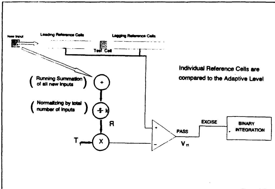
Figure 56. Excision Logic
