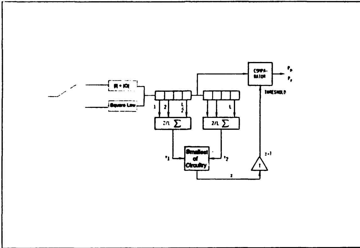
Figure 15. SO CFAR Schematic
