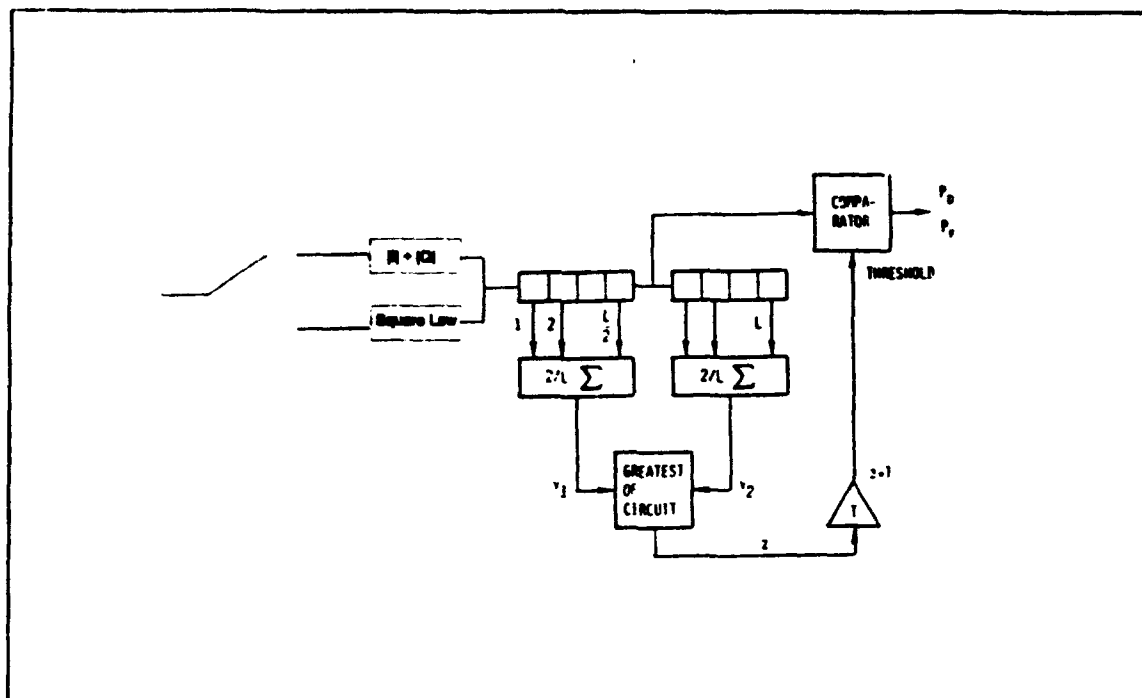
Figure 12. GO CFAR Schematic
