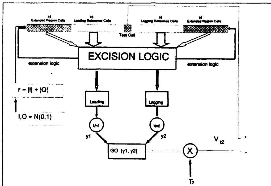
Figure 55. EXGO Schematic
