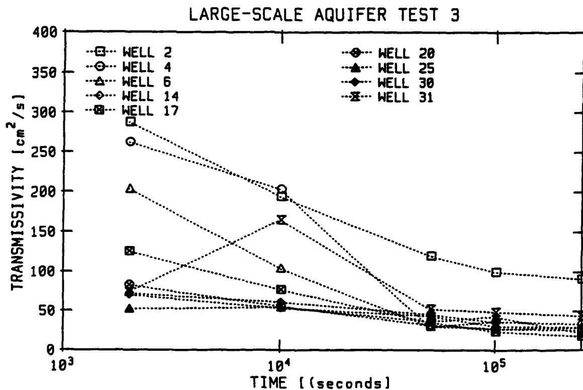
Figure 37. Transmissivities as a Function of Time for Large-Scale Aquifer Tests 1 and 3.
