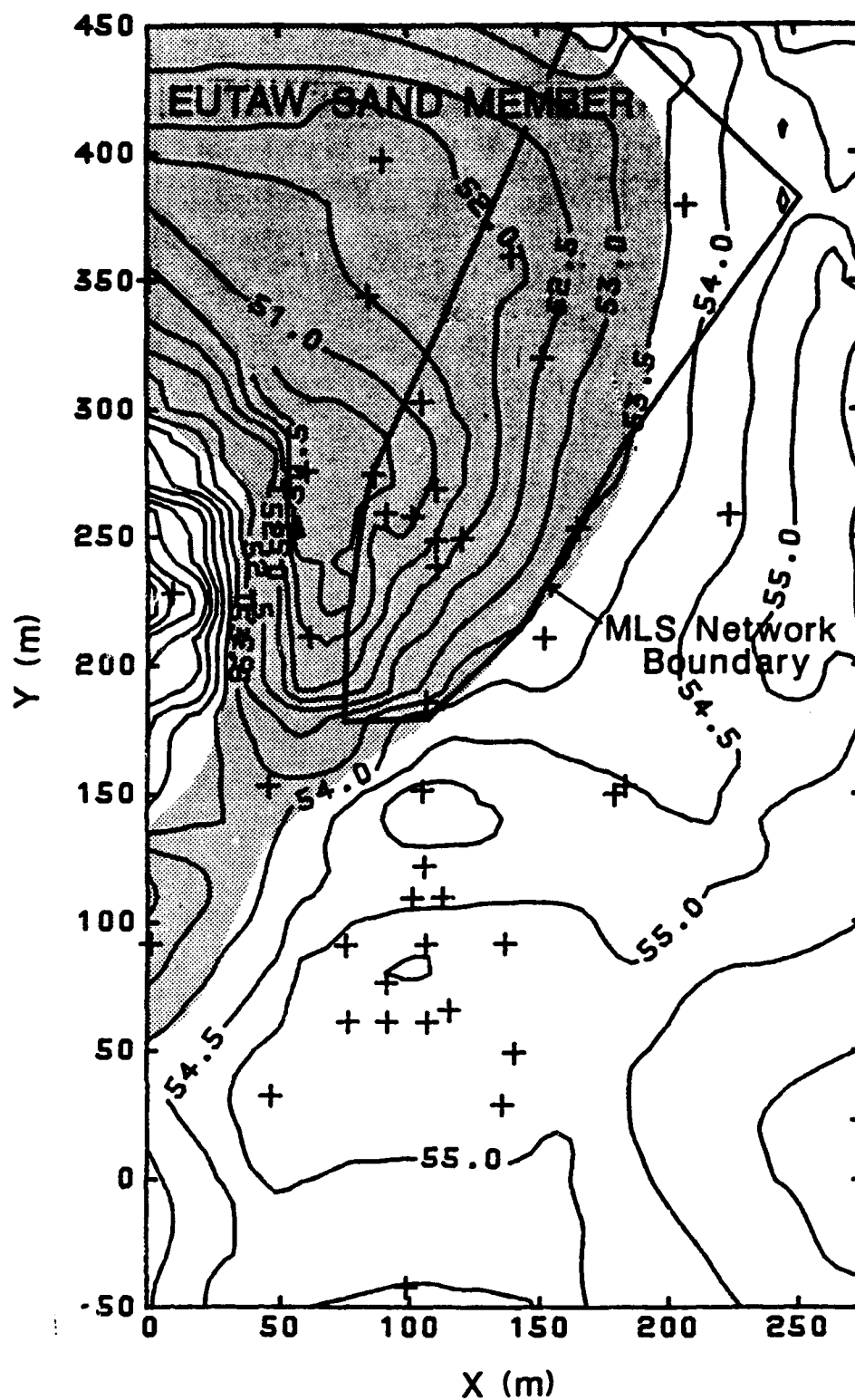
Figure 27. Elevation of Top of Eutaw Formation (Contours in Meters MSL -- after Boggs, et al., 1990).
