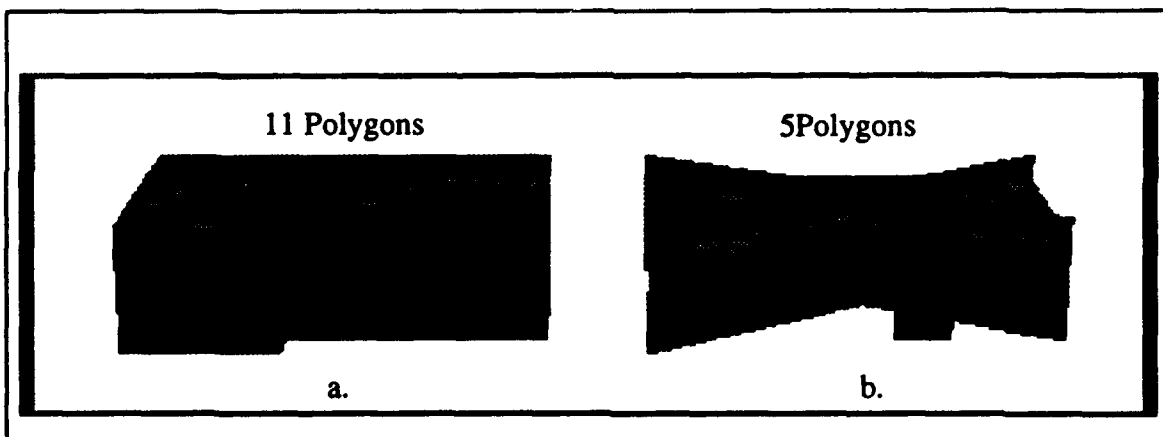
Figure 5 Replacement LODs
