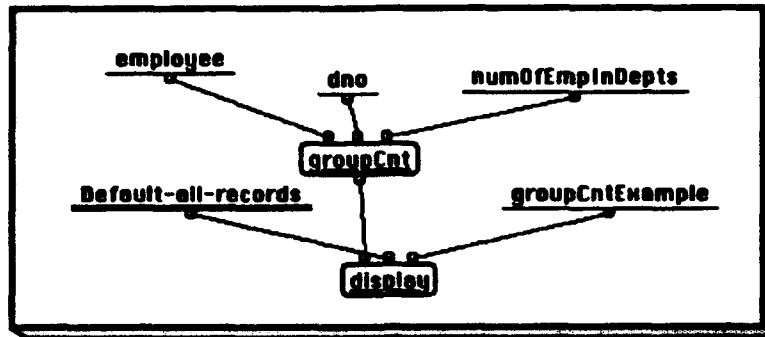
Query 3.9 List the number of employees in each department of the company.
