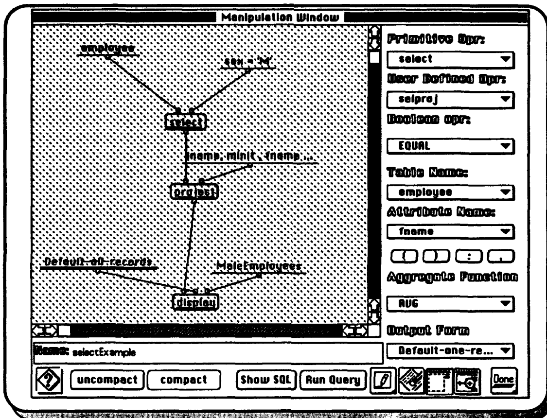
Figure 4.5 Compacted query shaded with a pattern to indicate that no modification is allowed other than traversing into the user-defined operators.
