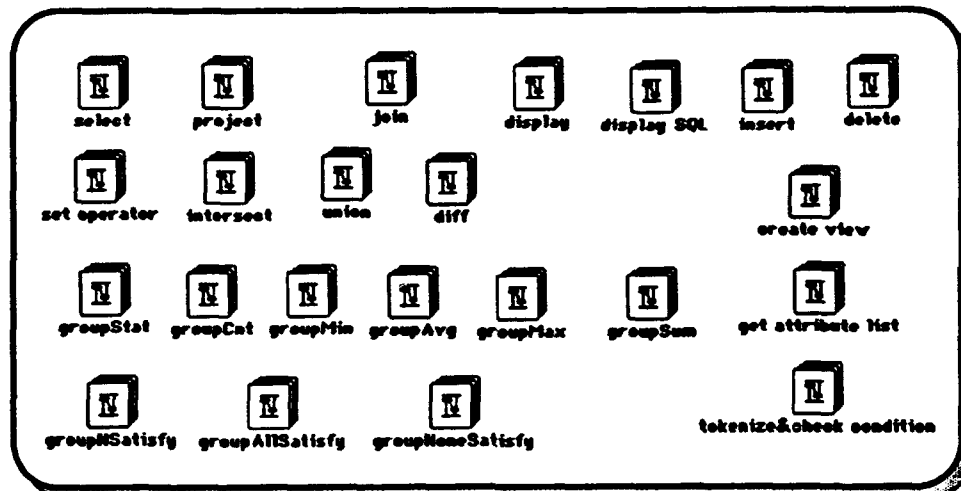
Figure 5.6 The necessary methods of class Oracle Relation where all primitive operators are implemented for the Oracle RDBMS.
