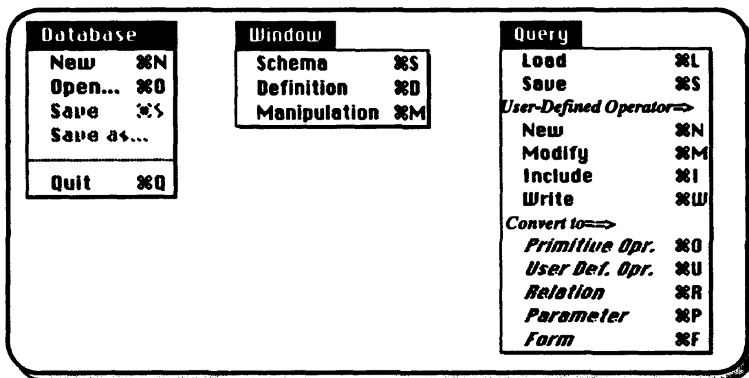
Figure 4.1 Pull-down menus for Amadeus.
