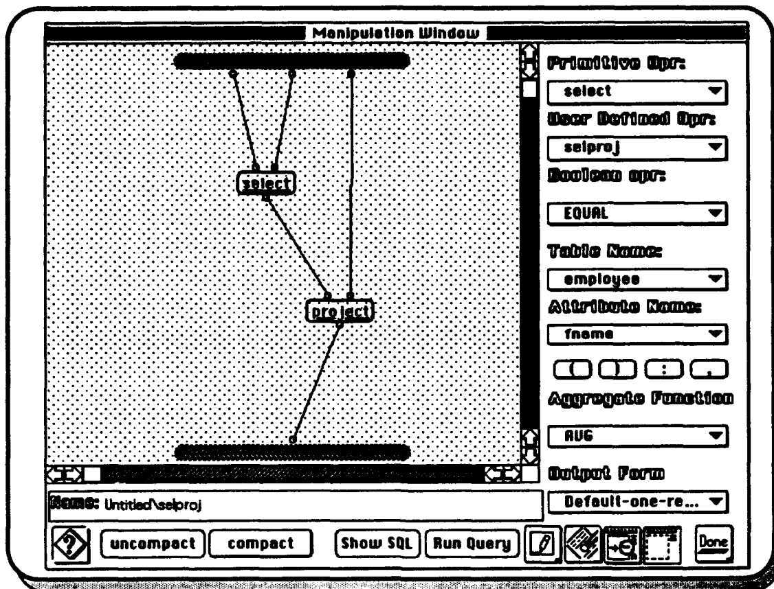
Figure 4.4 Creation of a user-defined operator in the manipulation window.
