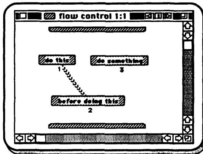
Figure B. 5 Synchro Link to control the execution order of the methods in Prograph.
