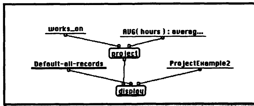
Query 3.4 Give the average number of hours worked on all projects in the company.
