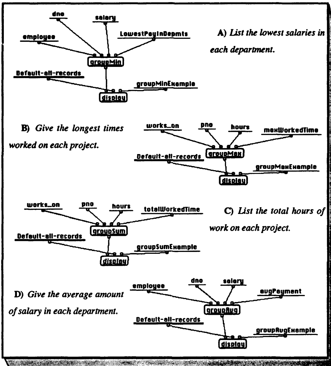
Query 3.11 Group aggregate functions' examples.
