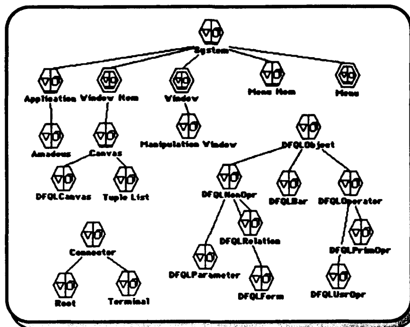
Figure 5.2 The OO design of the graphical editor in Prograph (other classes are not shown).
