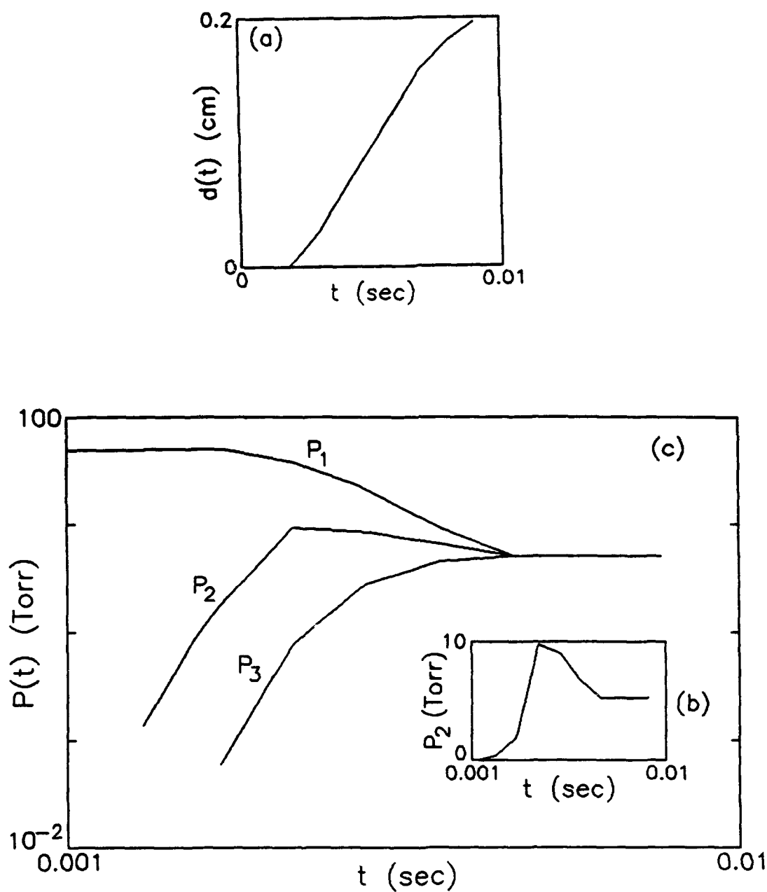
Figure 8. Gap Spacing and Pressure Histories in the Present UI Flow Systems
