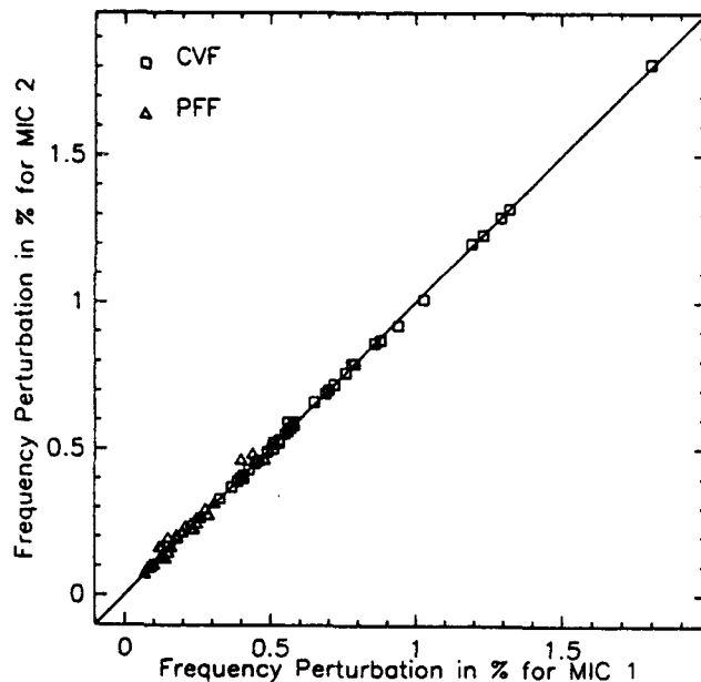
Figure 3 (top). Scatter plot of microphone 1 (the 410) versus microphone 2 (the 451) for amplitude perturbation analysis (CVA and PFA) using ten male subjects and ten female subjects at two F_0 s. Figure 4 (bottom). Scatter plot similar to Figure 3 for frequency perturbation measures.
