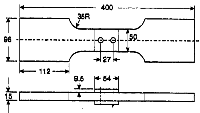
(a) low-load-transfer joint specimen
