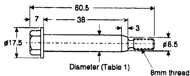
(c) Fastener
