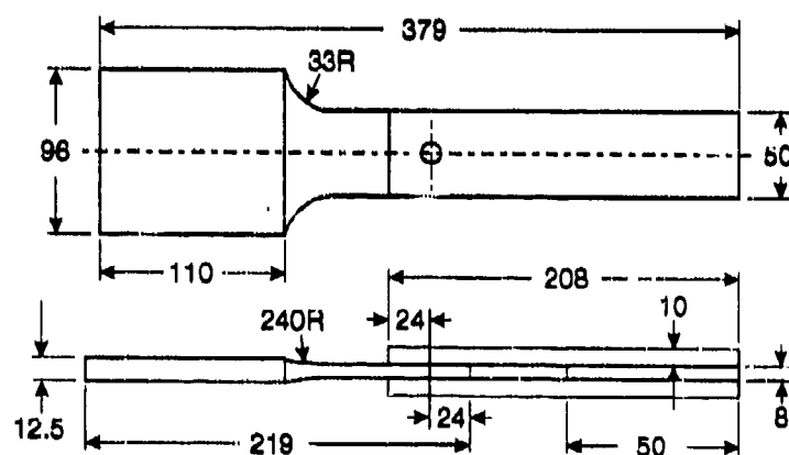
(b) 100% - load-transfer joint specimen
