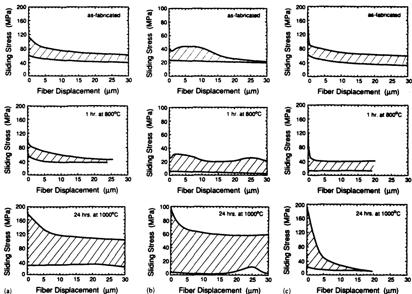
Fig. 5. Range of results for push-out tests, comparing the behavior of as-hot isostatically pressed and heat treated specimens. (a) carbon black, (b) colloidal carbon, and (c) carbon + alumina debond coating. In all cases the carbon is eliminated during the oxidative heat treatment.
