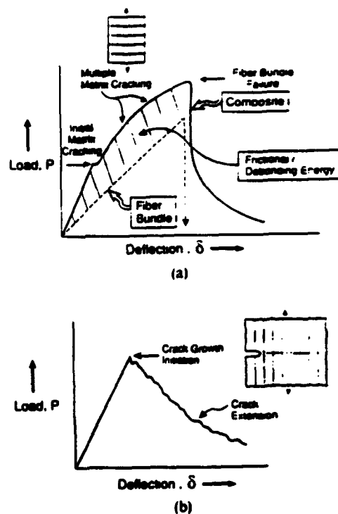
Fig. 2. Load/deflection curves and fracture behavior of unidirectional ceramic matrix composites: (a) Class I materials; (b) Class II materials. The cross-hatched area represents the energy per unit volume that goes into multiple matrix cracking, interface debonding and frictional sliding; the latter is typically the major contribution.
