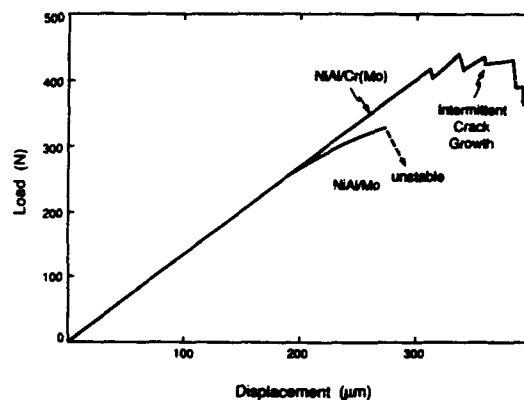
Fig. 6. Load/displacement curves measured for the two materials.
