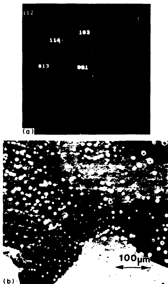
Fig. 8. (a) Channeling patterns obtained on a gold surface revealing the (001) orientation. (b) A view of the sub-grains in the gold obtained in the SEM.
