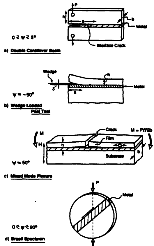
Fig. 2. Sandwich test specimens suitable for interface fracture energy measurements.
