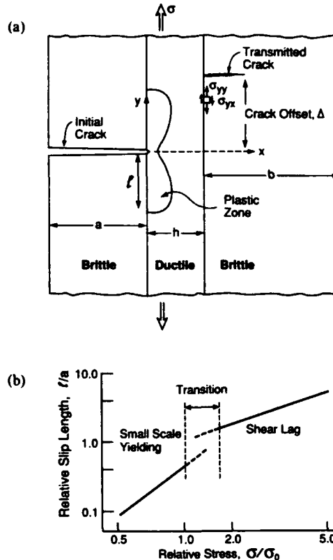
Fig. 6. (a) A schematic showing the plastic zone width, \ell . (b) Schematic of trends in plastic zone size. At small stresses, the results are conveniently normalized using small-scale yielding \ell/a \sim (\sigma/\sigma_0)^2 , while at larger stresses, a shear lag scaling is used, \ell/a \sim (\sigma/\sigma_0) .
