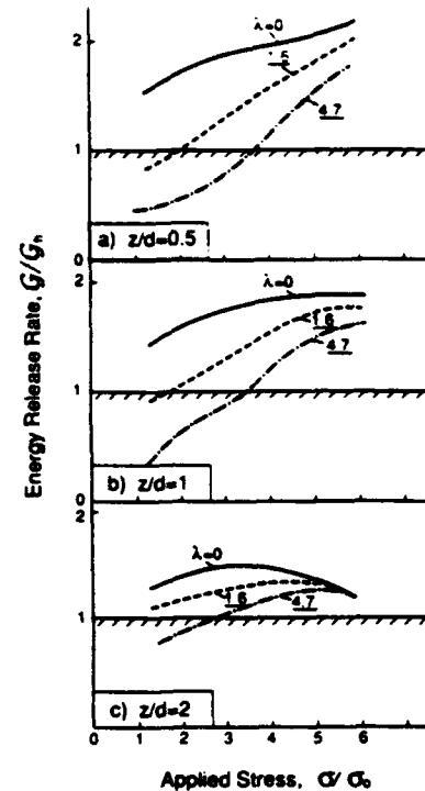
Fig. 10. Effect of stress and expansion misfit on the energy release rate for long cracks ( a/h = 0.2 ), (a) z/d = 0.5 , (b) z/d = 1.0 , (c) z/d = 2.0 .
