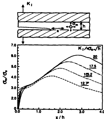
Fig. 6. Variations in the hydrostatic stress ahead of the crack for a range of metal layer thicknesses.
