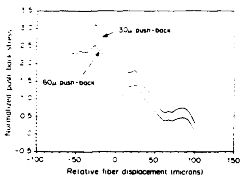
Fig. 13. Push-back reseating load drop is modelled by implementing a wear process during fiber sliding.
