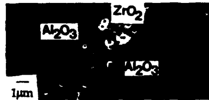
Fig. 7. SEM micrograph of \text{ZrO}_2 interfaces on \text{Al}_2\text{O}_3 (a) porous interlayer that fractures through the layer with \Gamma_R = 4 \text{ Jm}^{-2} (b) dense interlayers that fracture at the interface with \Gamma_R \approx 20 \text{ Jm}^{-2} .
