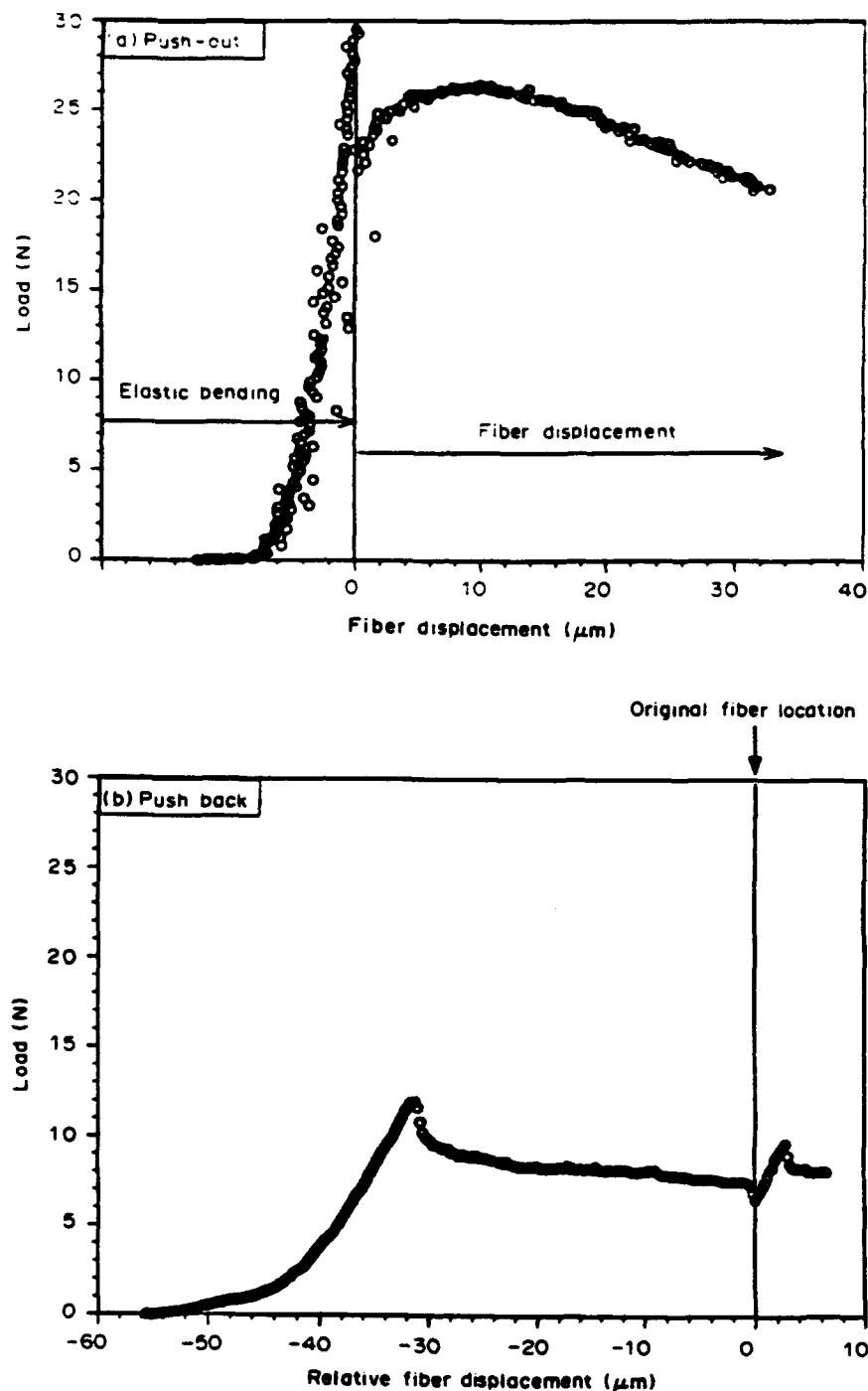
Fig. 1. Fiber push-out (a) and push-back (b) in a Ti(15-3)-SCS-6 composite. During fiber push-out, there is a notable increase in the sliding stress associated with the first few microns of fiber sliding. Note the reseating load drop associated with fiber push-back ( h = 410 \mu\text{m} ).
