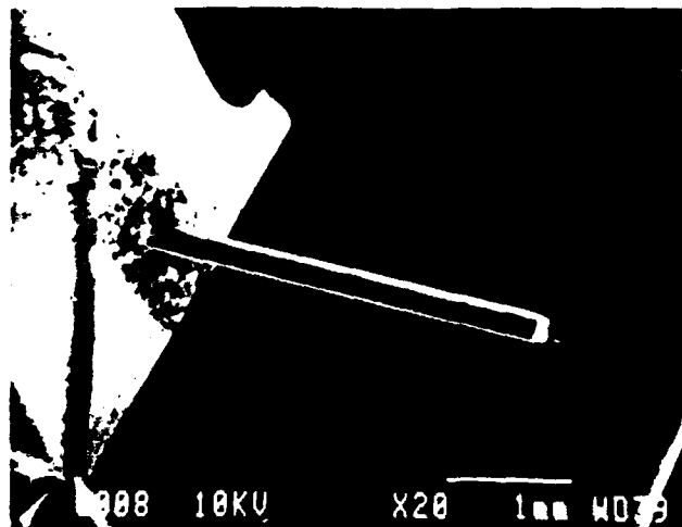
Fig. 12. Long fiber pull-out can result when thick (6 μm) Mo coatings are removed by oxidation.
