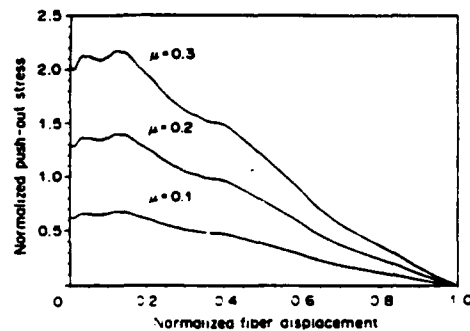
Fig. 9. An increase in the coefficient of friction, \mu , increases fiber sliding stress.
