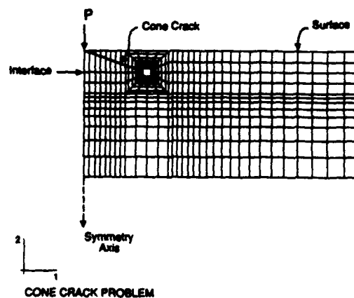
Fig. 7. The finite element mesh used to compute the energy release rate G and the phase angle of loading, \Psi .
