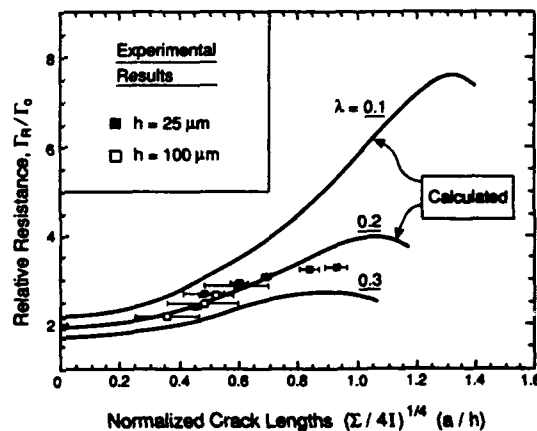
Fig. 13. Resistance curves predicted for interface cracks with bridging tractions [18]. Experimental data points from Fig. 3 are also shown: I is the moment of inertia of the beam and \Sigma is given by equation (7).
