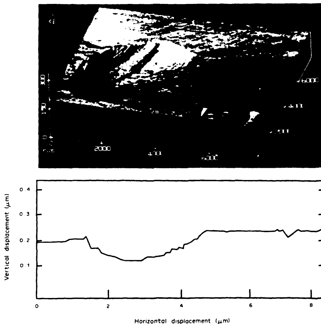
Fig. 4. A void on the fracture surface between Pt and \text{Al}_2\text{O}_3 and the AFM trace that can be used to obtain the dihedral angle.
