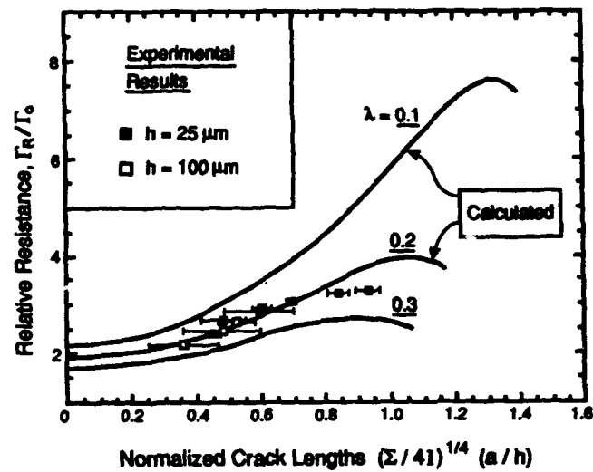
Fig. 8. b) A comparison of the measured resistance curve for Au/Al 2 O 3 with calculations based on a ligament model.
