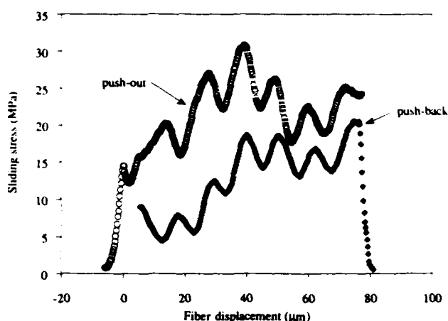
Fig. 4. Fiber roughness appears as a sinusoidal modulation in the push-out curve. Note the approximately 10 \mu\text{m} wavelength characteristic of the sapphire fiber surface topography.
