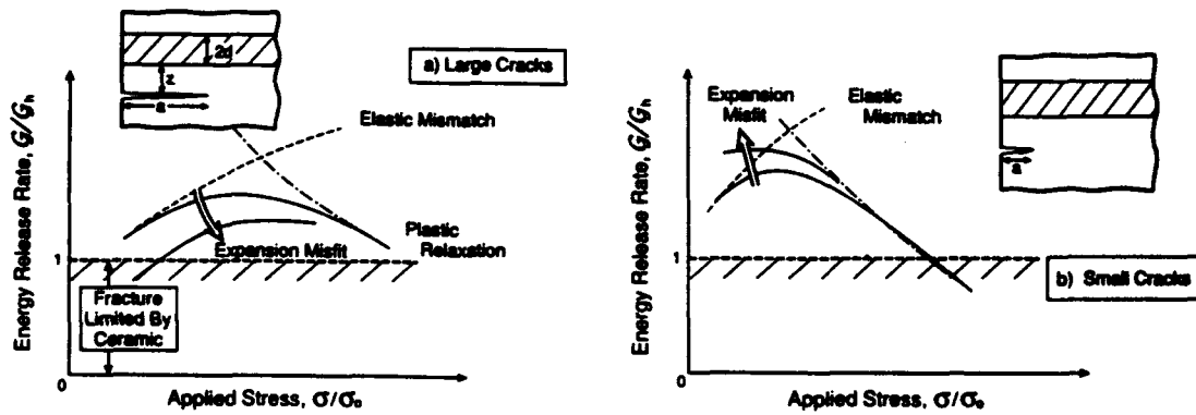
Fig. 7. A schematic indicating trends in the energy release rate with applied stress (a) large cracks (b) small cracks, a/h \lesssim 0.1 .
