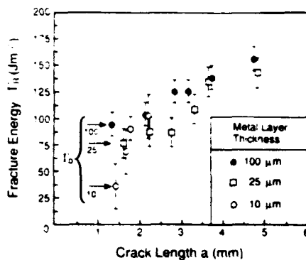
Fig. 10. Interface fracture resistances for the \text{Al}_2\text{O}_3 -Au interface.
