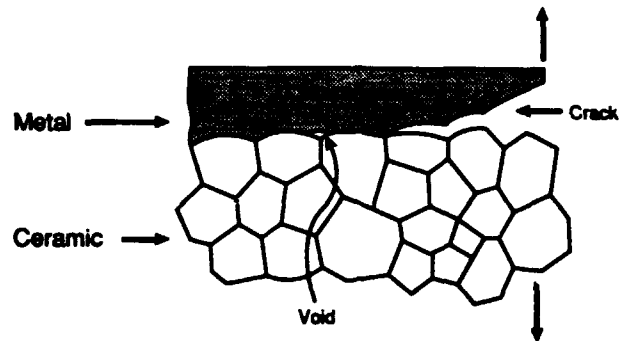
Fig. 1. a) A schematic of interface fracture by void growth.
