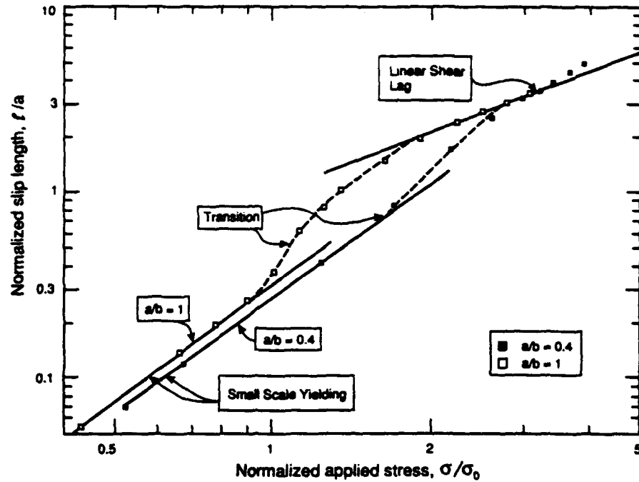
Fig. 10. Calculated trends in non-dimensional slip length l/a with relative applied stress. Also shown are the analytical small-scale yielding and shear lag predictions.
