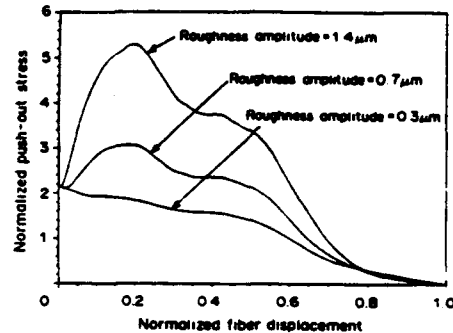
Fig. 8. An increase in roughness amplitude has a pronounced effect on fiber sliding.
