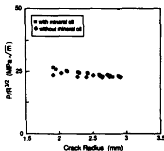
Fig. 4. Trends in cone crack radius R with load P obtained for glass, plotted in accordance with the parameter P/R^{3/2} suggested by equation (1).
