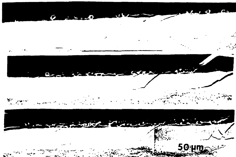
Fig. 7. Interface fracture path, for the thicker layer (120 h bond). Tunnel cracks form a damage zone ahead of the interface crack.
