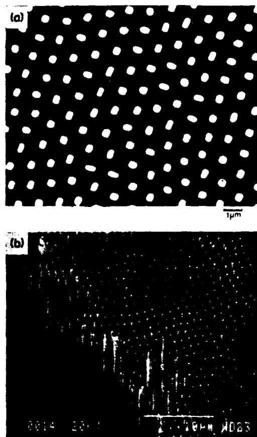
Fig. 2. Cross section of the NiAl/Mo system examined in the scanning electron microscope, (a) general view, (b) aligned rods.
