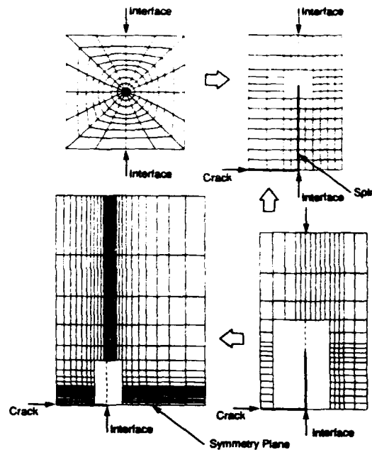
Fig. 8. Finite element mesh used to evaluate effects of slip and splitting.
