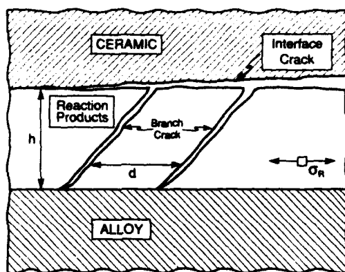
Fig. 9. Schematic of cracking mechanisms.
