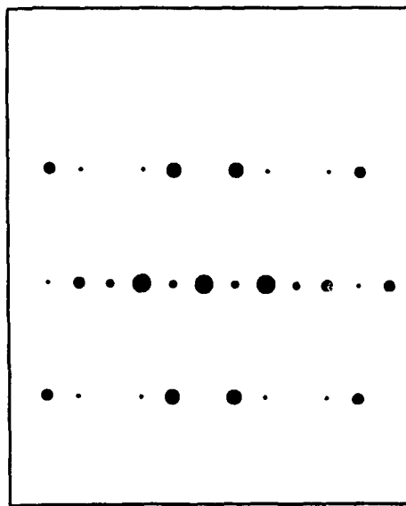
Calculated \bar{1}2\bar{1}2 zone
