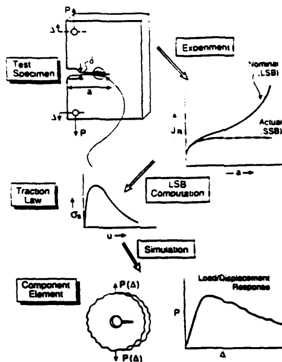
Fig. 7. Procedure for measuring the crack surface tractions and relating to the load/deflection properties of composite structures.
