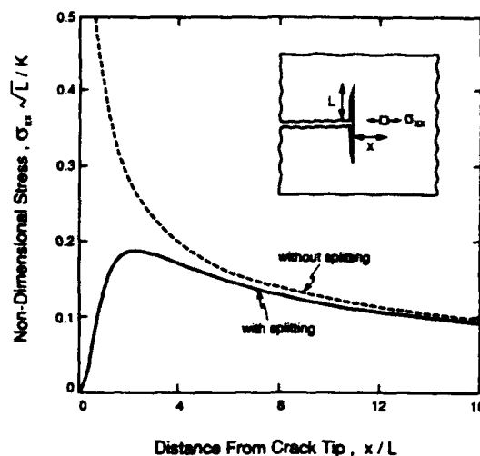
Fig. 10. The in-plane, \sigma_{xx} stress ahead of a crack with a split.
