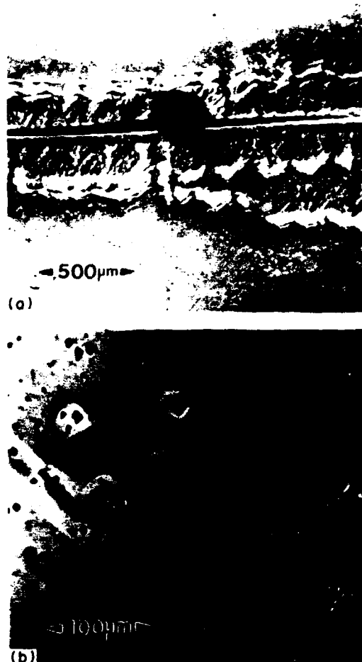
Fig. 2. (a) A precracked specimen viewed through the sapphire layer revealing the symmetrical cracks at the interface (specimen unloaded). (b) Also visible at higher magnification is the faceted nature of the apparent (closure) crack front and the residual opening around voids.
