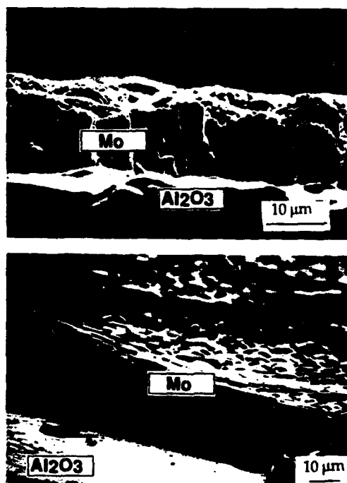
Fig. 2. Coating microstructures revealed by scanning electron microscopy (A) after physical deposition (Mo coating); (B) after diffusion bonding (Mo coating).
