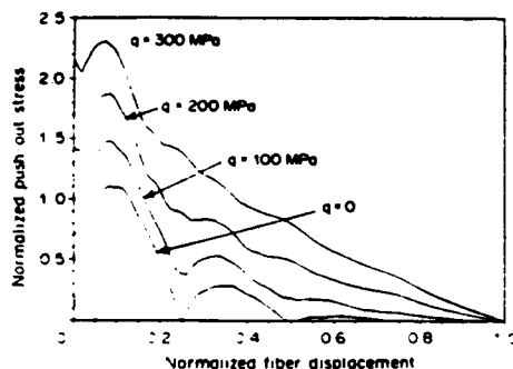
Fig. 11. A change in the thermal misfit at identical roughness changes both the character and magnitude of the sliding stress; q is the thermal expansion misfit stress, q = E\epsilon_t .
