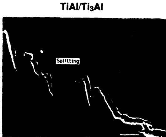
Fig. 6. A crack within a layered, colony structure exhibited by the system, TiAl/Ti 3 Al.
