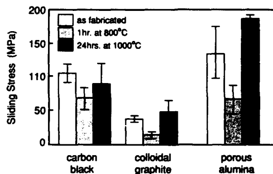
Fig. 6. Comparison of the peak sliding stress for each coating and each heat treatment condition as calculated from the tests illustrated in Fig. 5. Means and standard deviations are derived from a minimum of five push-outs for each coating and heat treatment.
