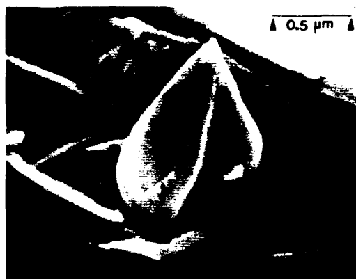
Fig. 9. Higher-resolution SEM views of the fracture surface of the NiAl/Mo indicating characteristic crack trapping "trails" in the NiAl.
