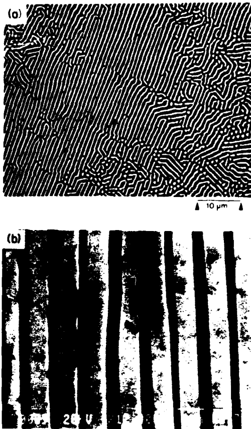
Fig. 3. Cross section of the NiAl/Cr(Mo) system examined in the SEM, (a) overview, (b) layers.
