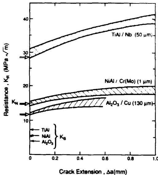
Fig. 3. Resistance curves for three layered materials, (a) \text{Al}_2\text{O}_3/\text{Cu} with h_m \approx 130 \mu\text{m} , (b) \text{NiAl}/\text{Cr}(\text{Mo}) with h_m \approx 1 \mu\text{m} , (c) \text{TiAl}/\text{Nb} with h_m \approx 50 \mu\text{m} .
