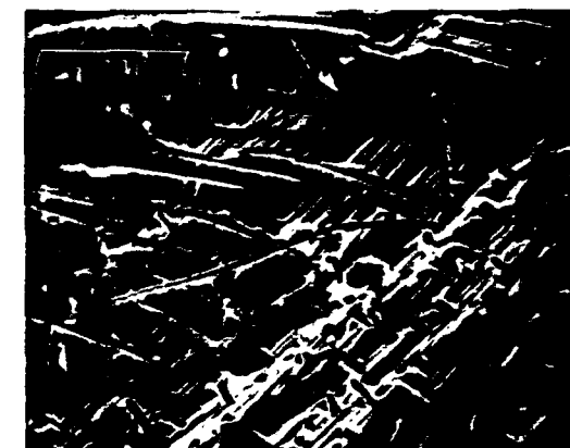
Fig. 8. SEM fractographs of the NiAl/Mo system showing plastic stretch of the Mo and interface debonding.
