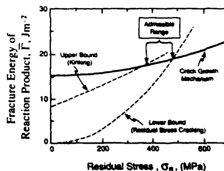
Fig. 11. Upper and lower bounds on the relationship between \bar{\Gamma} and \sigma_R established by crack kinking and tunnel cracking requirements. The allowable \sigma_R/\bar{\Gamma} line governed by the fracture mechanism is superimposed. The admissible values of \sigma_R and \bar{\Gamma} are identified.
