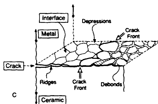
Fig. 21. Interface debonding mechanism in Pt-Al 2 O 3 interface. Decohesion of amorphous phase ridges (a) and (b). Progressive debonding of the intervening interface is schematically represented in (c).
