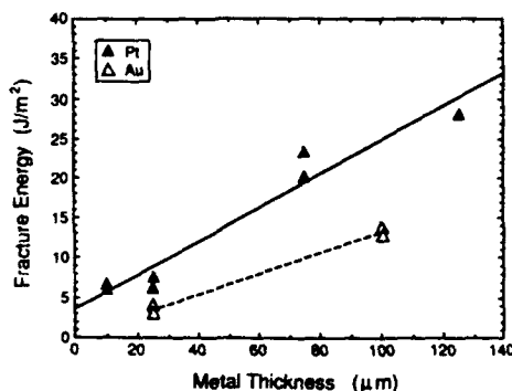
Fig. 7. Effects of Pt thickness on the mode I nominal interface fracture energy for Pt-polycrystalline \text{Al}_2\text{O}_3 . Results for Au- \text{Al}_2\text{O}_3 bonds are also shown.
