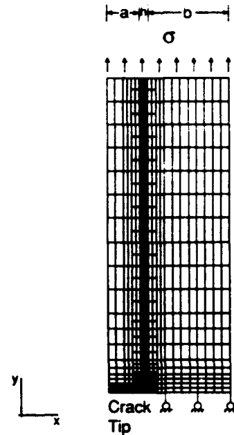
Fig. 8. Finite element mesh for three-layer system ( a/b = 2/5 , h/a = 1/4 ).
