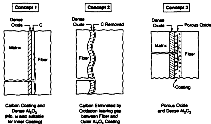
Fig. 1. Schematic representation of three double coating concepts for sapphire fibers in \gamma -TiAl matrix composites.
