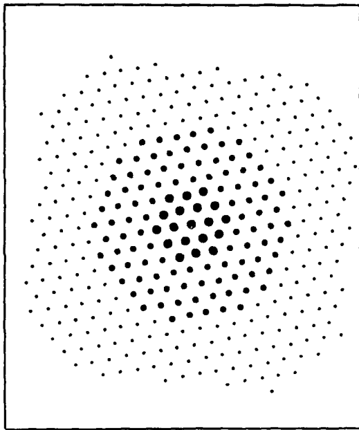
Calculated 1\bar{1}\bar{1} zone
