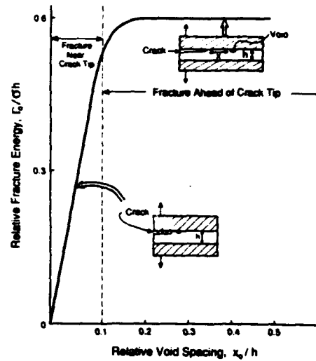
Fig. 7. Trends in interface fracture energy with metal layer thickness when fracture occurs by a ductile mechanism.
