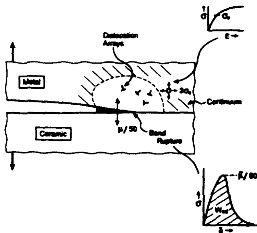
Fig. 15. A schematic of the features around an interface crack that fails by brittle debonding.
