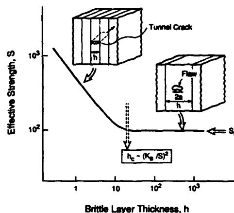
Fig. 11. A schematic of the trend in strength with brittle layer thickness.
