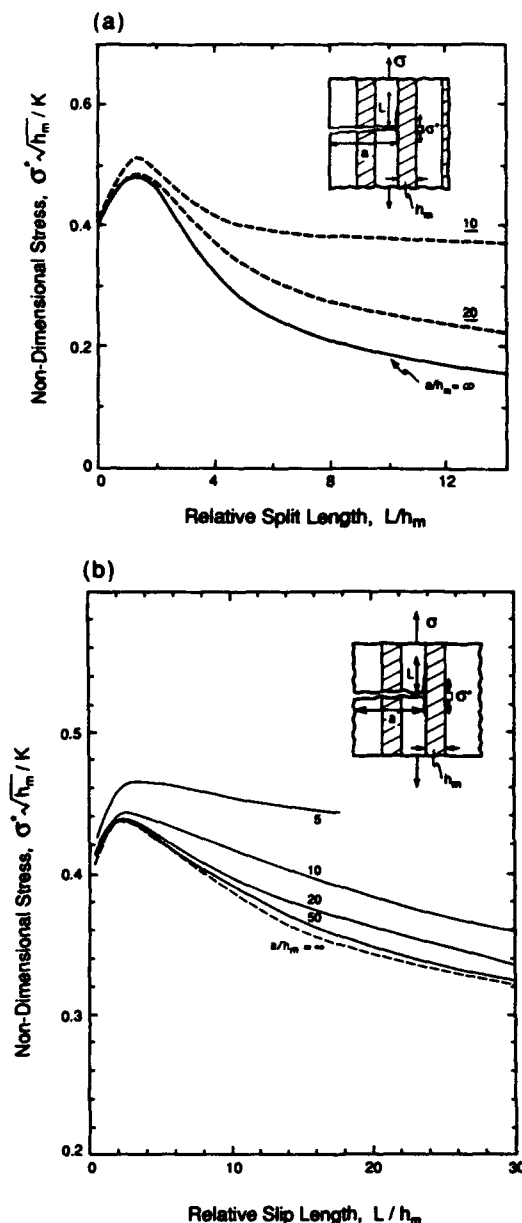
Fig. 9. Effect of crack size on the stress ahead of a crack subject to (a) splitting or (b) slip.
