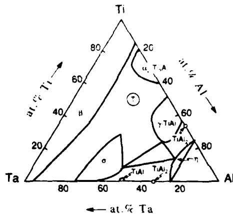
Fig. 1. Ti-Ta-Al ternary phase diagram.
