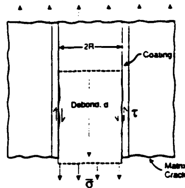
Fig. 1. A typical 'interface' in a brittle matrix composite: (a) schematic illustration showing a debond crack formed following matrix cracking; (b) the LAS/Nicalon system, with debonding within the carbon layer caused by thermal expansion misfit.
