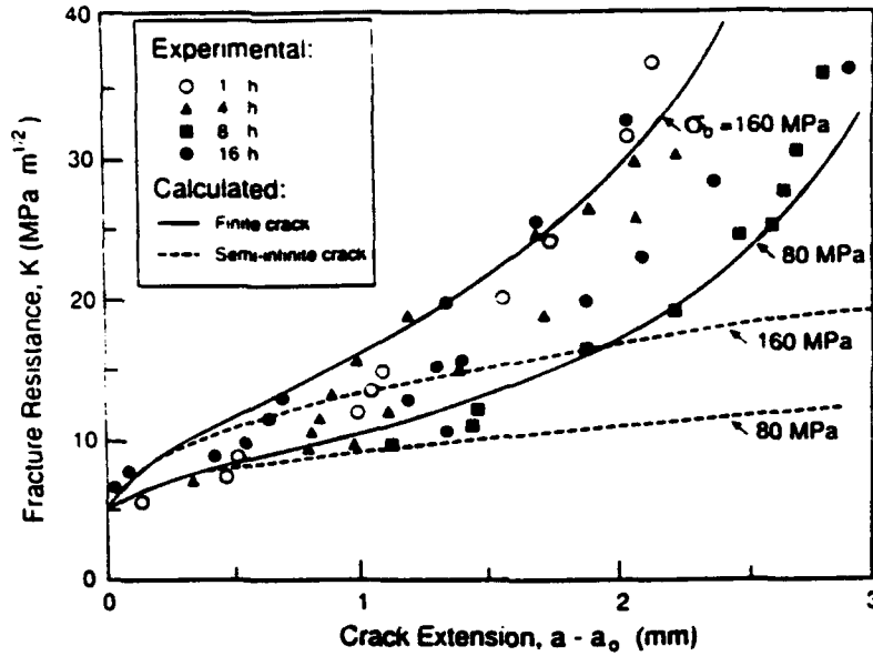
Fig. 6. Mode I fracture resistance curves for a LAS/Nicalon composite following heat treatment at 800°C for times indicated in the legend. Also shown are the simulated curves.
