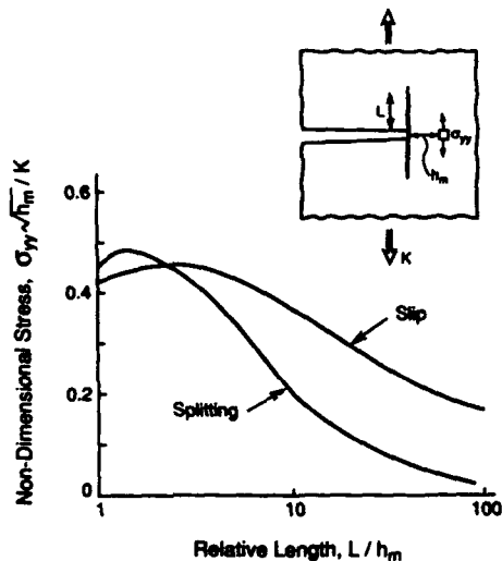
Fig. 13. Effects of slip and splitting on the \sigma_{yy} stress ahead of a semi-infinite crack in a layered material [20].
