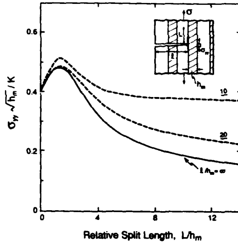
Fig. 14. Effects of splitting on the stress ahead of a finite crack in a layered material [21].
