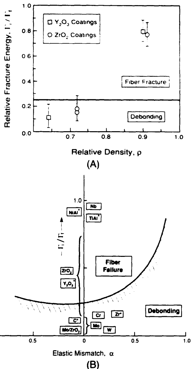
Fig. 8. (A) The relative density of oxide coatings plotted as a function of \Gamma_i/\Gamma_f clarifies the role of coating porosity in the debonding process. (B) A summary of the interfacial fracture energy measurements for various coatings on sapphire is presented on a "debond map." Coatings which fall within the fiber debonding regime of the map have some potential for sapphire fibers. However, coatings denoted by \star were found to chemically react with sapphire; these were precluded from further consideration.
