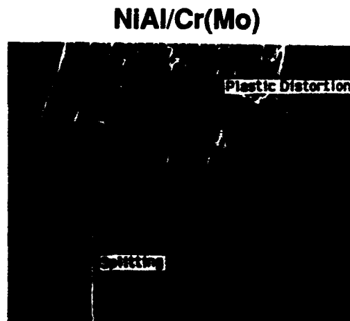
Fig. 5. The fracture surface for a \text{NiAl}/\text{Cr}(\text{Mo}) layered material indicating splitting, as well as plastic distortion.
