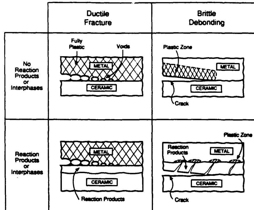
Fig. 1. A schematic indicating the various fracture mechanisms that occur in metal-ceramic interfaces.
