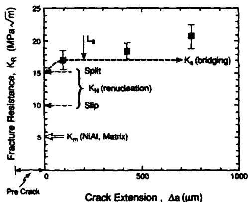
Fig. 12. Predictions of initiation toughness for weakly bonded layered systems with and without splitting and comparison with results for \text{NiAl}/\text{Cr}(\text{Mo}) .
