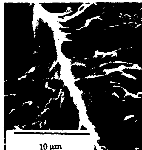
Fig. 2. A scanning electron fractograph of a diffusion-bonded \text{Al}_2\text{O}_3/\text{Al} material indicating plastic stretch of the Al to a ridge.
