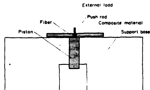
Fig. 1. Schematic diagram of the fiber push-through apparatus.
