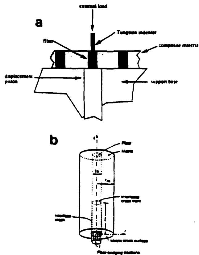
Fig. 9. Schematics of test specimens used to evaluate the mechanical properties of interfaces: (a) fiber push-through; (b) fiber pull-out.
