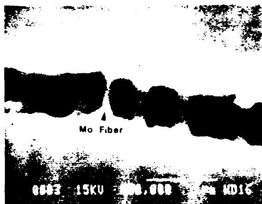
Fig. 7. SEM views of a crack extending in the NiAl/Mo system, indicating the plastic stretch of the Mo that occurs as the crack extends through the material.
