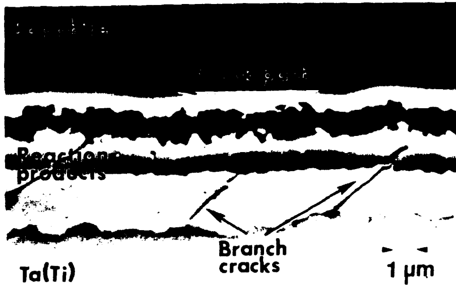
Fig. 5. Continued. (b) Crack trajectory when testing to obtain the fracture energy: note the periodic branch cracks in the reaction product layer and the roughness of the interface.
