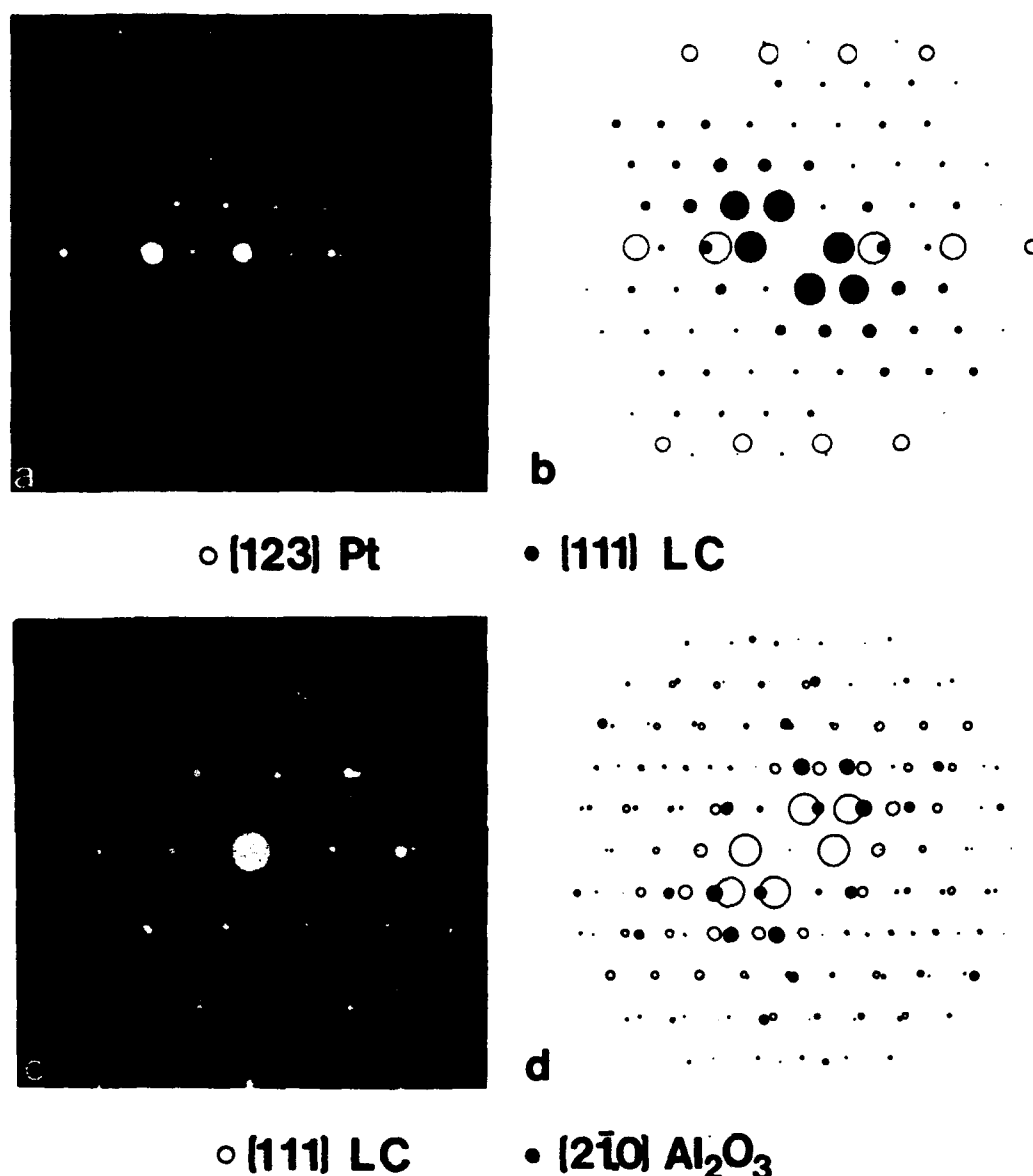
Fig. 14. (a, c) Experimental and (b, d) computed zone axis patterns for respectively the Pt-crystalite and the crystalite-sapphire interfaces.
