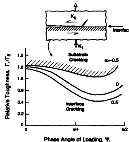
Fig. 3. A diagram indicating the region in which cracks deviate from the interface, using fracture energy/phase angle space.
