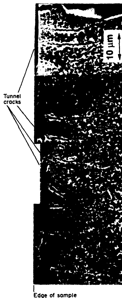
Fig. 6. Plan view of the reaction product layer subsequent to the removal of the sapphire, showing tunnel cracks in the reaction products (thin layer, 1.2 h bond).
