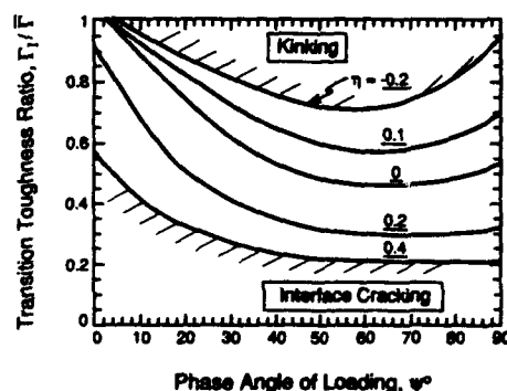
Fig. 10. Predicted kinking diagram when residual stresses exist: \eta is defined in equation (2). Kinking occurs when \Gamma_1/\bar{\Gamma} lies above the curve.
