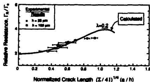
Fig. 14. Simulated resistance curves based on large-scale bridging by metal ligaments: experimental results are superposed.
