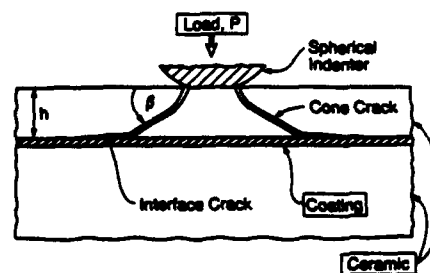
Fig. 1. A schematic of the test geometry and the cracking patterns associated with the elastic indentation technique.
