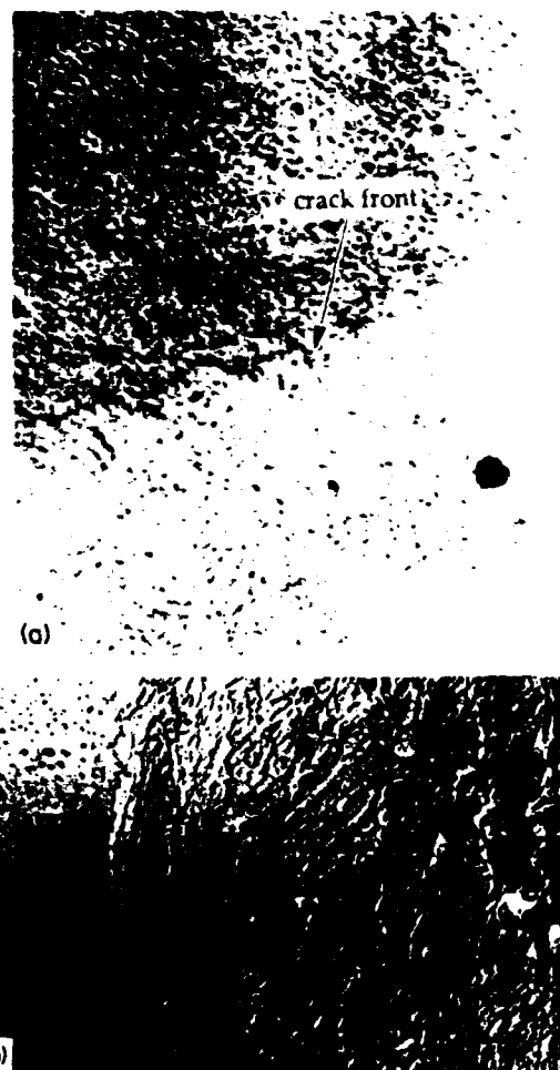
Fig. 9. Fracture surfaces observed in situ in the optical microscope for cracks extending at the Au/ \text{Al}_2\text{O}_3 interface: (a) moist air (RH 100%); (b) dry air indicating plastic distortion.
