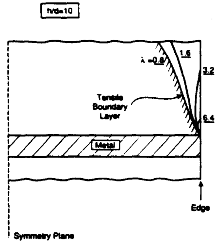
Fig. 4. The \sigma_{yy} tensile boundary layer caused by the residual field and the effect of the expansion misfit coefficient, \lambda = \Delta\alpha\Delta T/\epsilon_0 .
