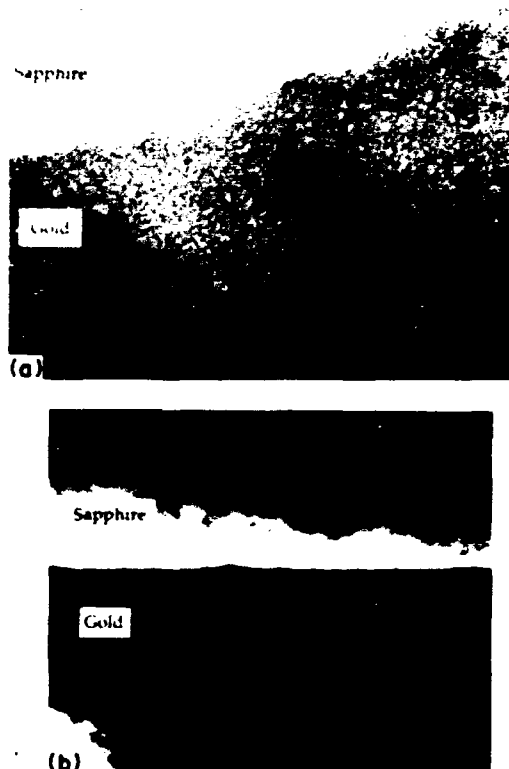
Fig. 11. (a) An atomic resolution image of the interface. (b) A conventional TEM view revealing interface non-planarity.
