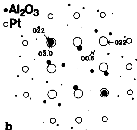
Fig. 13. (a) Experimental and (b) computed zone axis patterns for the [2\bar{T}.0] \parallel [100]_{\text{P}} orientation relation. Note that the Pt crystal is slightly misaligned in the experimental pattern.
