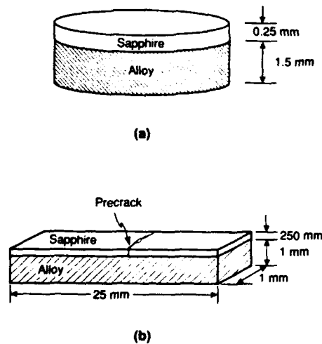
Fig. 2. (a) Schematic of geometry used for diffusion bonding. (b) Test specimen geometry for measuring mixed-mode interface fracture resistance.
