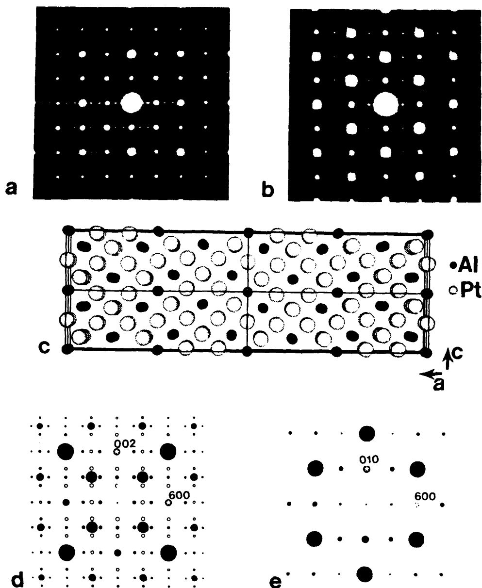
Fig. 11. (a) [010] and (b) [001] experimental diffraction patterns for the Pt_2Al intermetallic (orthorhombic, Pmma ); (c) structure drawing projected along the [010] axis. (d) and (e) computed zone axis patterns corresponding to (a) resp. (b). Open and filled circles in (d) refer to two orientation variants.
