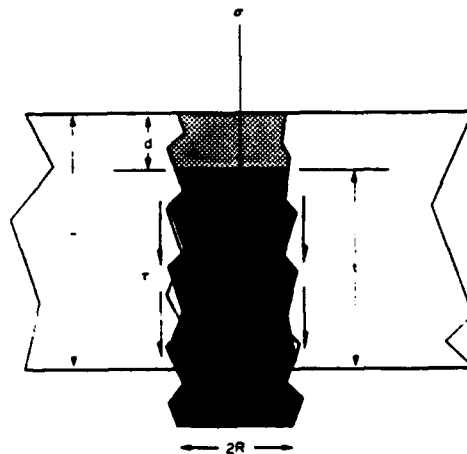
Fig. 3. Schematic of fiber sliding and the associated geometry.
