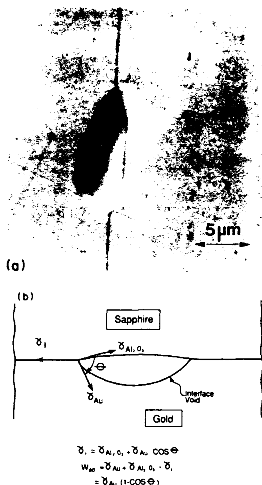
Fig. 10. (a) An electron damage line across an interface void, tilted to determine the void profile. (b) Schematic of the approach used to estimate the work of adhesion W_{\text{ad}} .
