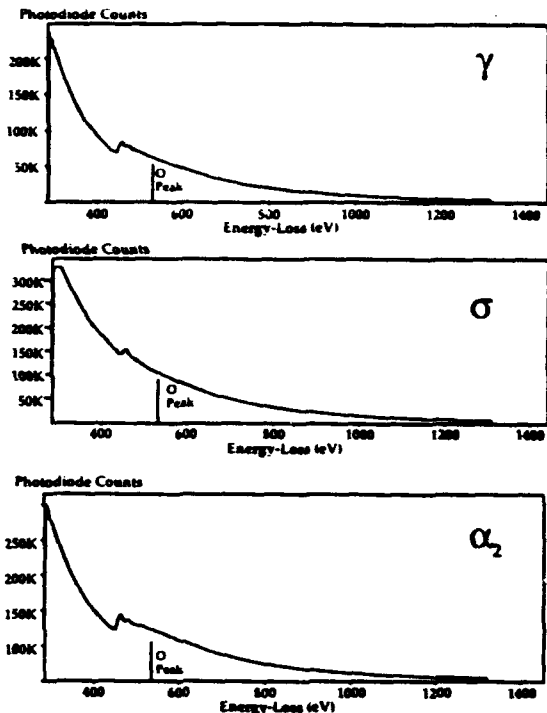
Fig. 2. PEELS spectra for the metal and reaction product layers revealing the absence of oxygen within detectable limits .
