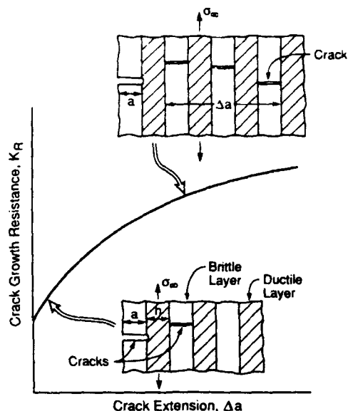
Fig. 1. A schematic of crack growth in a layered material with associated resistance curve.
