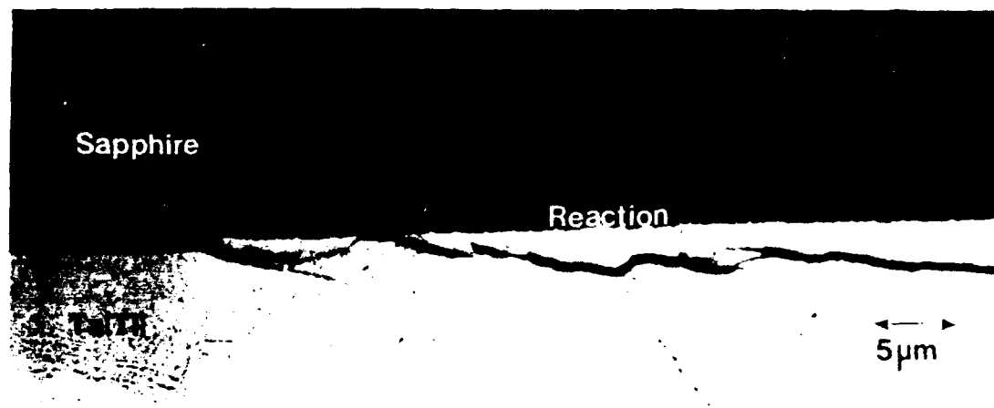
Fig. 7. Crack in the reaction product layer for a system with negative misfit ( \epsilon_1 \approx 5 \times 10^{-4} ).
