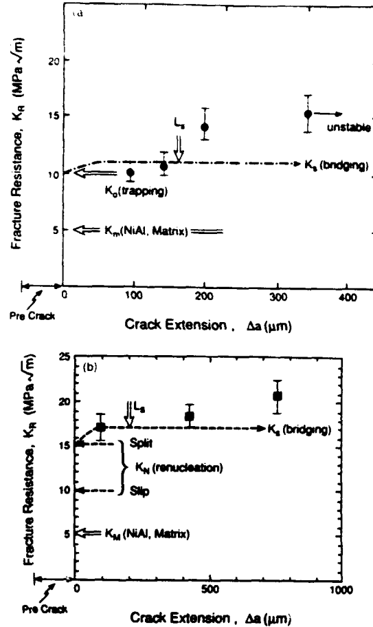
Fig. 5. Resistance curve results, (a) NiAl/Mo, (b) NiAl/Cr(Mo). Also shown are predicted values of the initiation toughness and subsequent propagation resistance.
