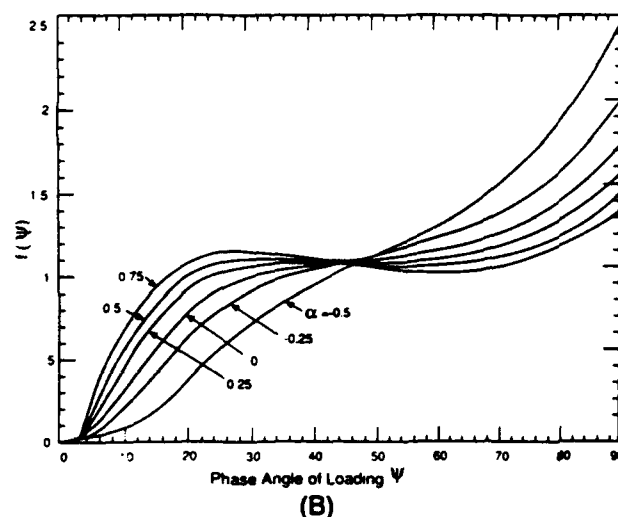
Fig. 7. (A) Energy release rate ratio versus \psi \equiv \tan^{-1}(K_2/K_1) for \eta = 0 . (B) Coefficient of lowest order contribution of \eta to energy release rate ratio in Eq. (24). In both cases, \beta = 0 .
