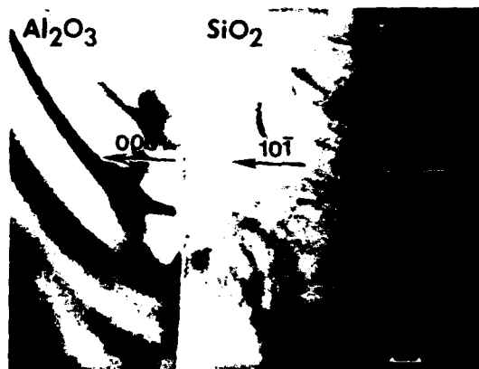
Fig. 19. TEM cross section of Pt-Al 2 O 3 bond with SiO 2 (cristobalite) interphase.
