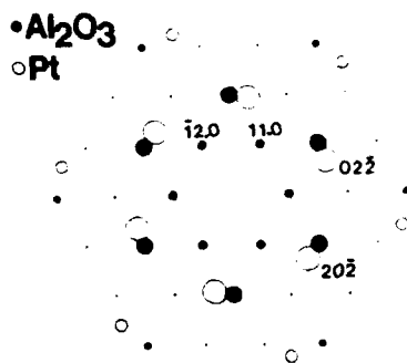
Fig. 9. Computed zone axis pattern for a [00.1]_S = [111]_{Pt} zone axis in the same orientation relation as in the previous figure.
