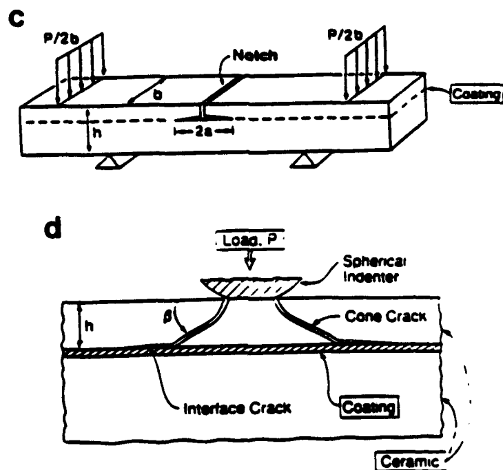
Fig. 9—contd. (c) mixed-mode flexure; (d) interfacial cone crack.
