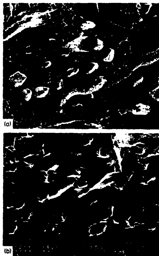
Fig. 8. Incidence of ductile debonding between Al alloy-reinforced \text{Al}_2\text{O}_3 : (a) extensive debonding in materials with a 2 \mu\text{m} grain size, (b) absence of debonding in a material with 20 \mu\text{m} grain size.
