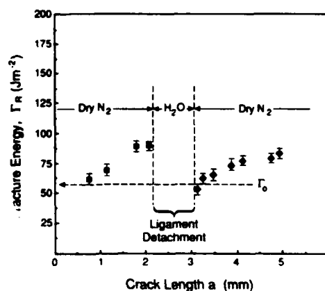
Fig. 13. The effect of removing the ligaments by stress corrosion on the resistance curve. Note that after the ligaments have been removed, the original resistance curve is duplicated.
