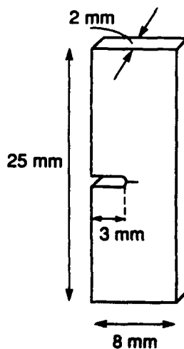
Fig. 4. The specimen geometry used for fracture resistance testing.
