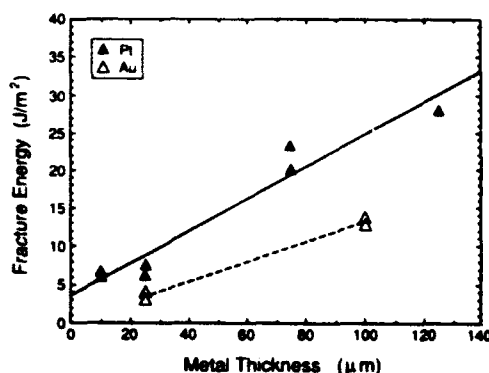
Fig. 17. Trends in \Gamma_i with metal layer thickness for interface between Au or Pt and commercial grade \text{Al}_2\text{O}_3 .
