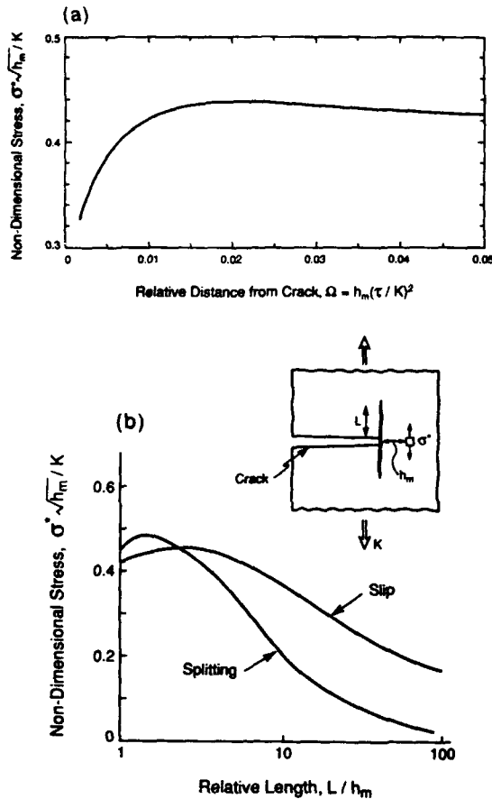
Fig. 7. Asymptotic solutions for the effects of slip and splitting on the stress, \sigma^* . (a) The normal stress ahead of the crack as a function of relative distance from the crack with a slip. (b) The normal stress ahead of the crack as a function of the relative slip or splitting length.
