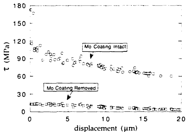
Fig. 13. Fiber push-out curves reveal that the interfacial sliding resistance was decreased to an acceptable level by removing the submicrometer thick (0.7 μm) Mo coating from the interface.
