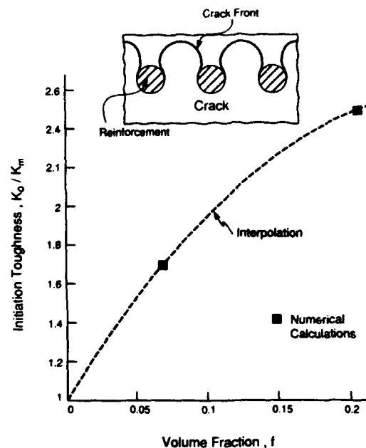
Fig. 12. Predictions of the influence of crack trapping on the initiation fracture toughness [15–18].
