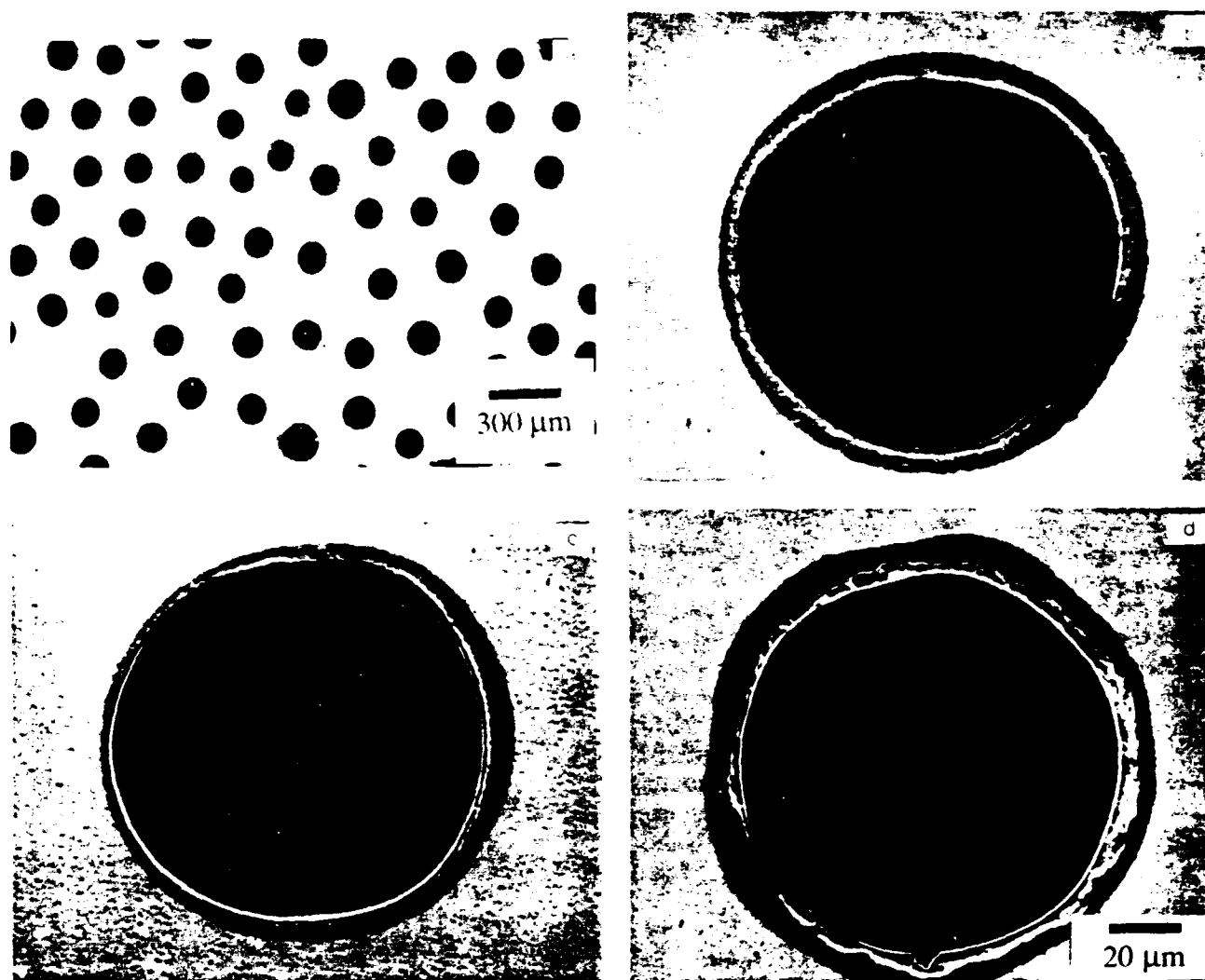
Fig. 2. Representative cross sections of double coated sapphire fibers: a. general view of a composite with 20-30 vol.% of double coated fibers; b. carbon black dense alumina; c. colloidal carbon dense alumina, and d. C + 10%Al 2 O 3 precursor to porous alumina followed by dense alumina.
