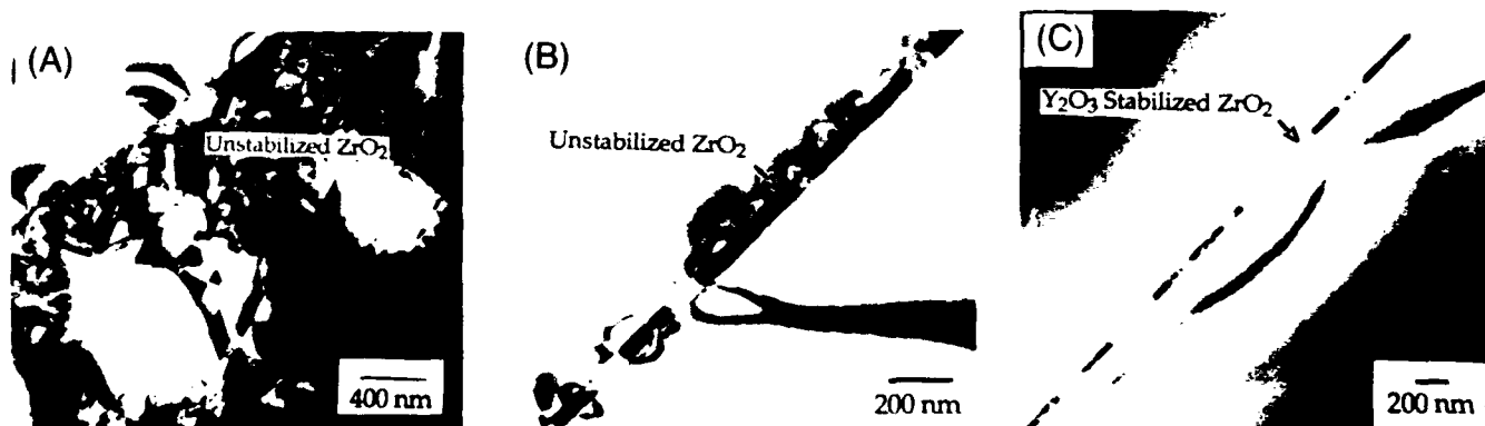
Fig. 3. (A) Extensive bend contours in the sapphire when unstabilized ZrO 2 sputtered coatings were used. It is believed that the contours result from strain in the fiber due to the t - \rightarrow m -ZrO 2 phase transformation. (B) The bend contours in the sapphire decrease with coating thickness for the unstabilized sol-gel ZrO 2 coating. (C) The extent of bend contours was further reduced when thin stabilized sol-gel ZrO 2 coatings were used. The remaining stresses are believed to result from CTE mismatch across the well-bonded interface.
