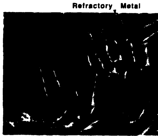
Fig. 11. A high-resolution view of a fracture surface showing plastic stretch of the refractory metal to a ridge.
