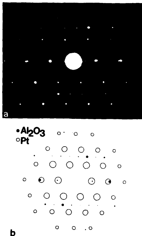
Fig. 8. (a) Experimental [101]_{\text{Pt}}-[45.0]_{\text{S}} zone axis pattern and (b) computation of this geometry for a [00.1]_{\text{S}}//[111]_{\text{Pt}} , (210)_{\text{S}}/(1121)_{\text{Pt}} orientation relation.
