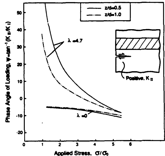
Fig. 11. Effects of stress and expansion misfit on the phase angle of loading for a long crack near the interface ( a/h = 0.2 ).
