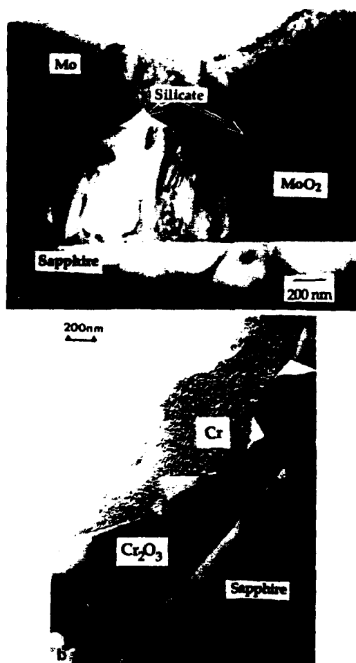
Fig. 25. Oxide interphase formation in \text{Al}_2\text{O}_3 refractory metal bonds: (a) \text{Mo}-\text{Al}_2\text{O}_3 with \text{MoO}_2 interphase, (b) \text{Cr}-\text{Al}_2\text{O}_3 with \text{Cr}_2\text{O}_3 interphase: the oxygen needed to form the oxide comes from solution in the refractory metal. Debonding occurs at the oxide-metal interface.
