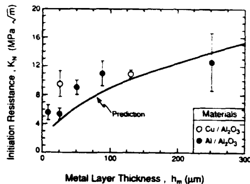
Fig. 4. Measurements of K_N as a function of metal layer thickness for the \text{Al}_2\text{O}_3/\text{Al} and \text{Al}_2\text{O}_3/\text{Cu} systems. The predictions are also shown.
