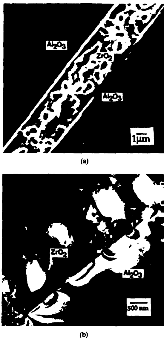
Fig. 11. (a) A porous \text{ZrO}_2 coating on \text{Al}_2\text{O}_3 ; debonding occurs within the coating. (b) A TEM view revealing residual stress in the \text{Al}_2\text{O}_3 .
