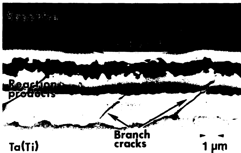
Fig. 5. A mixed-mode crack propagating along the sapphire/reaction product interface, 1/2 h bond. Note the appearance of periodic branch cracks.
