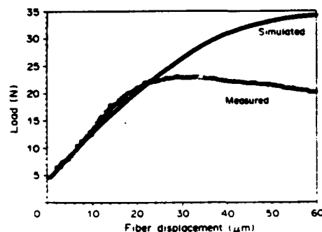
Fig. 12. Fatigue simulated by relaxing the misfit resembles experimental results.
