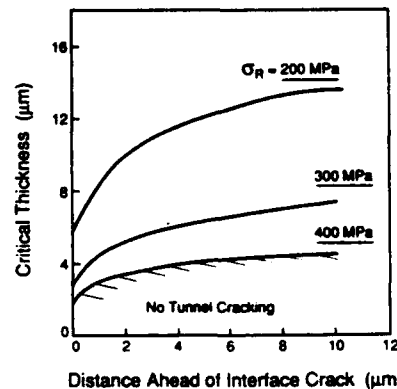
Fig. A1. Distance ahead of crack at which stress exceeds critical tunneling stress, as a function of layer thickness.
