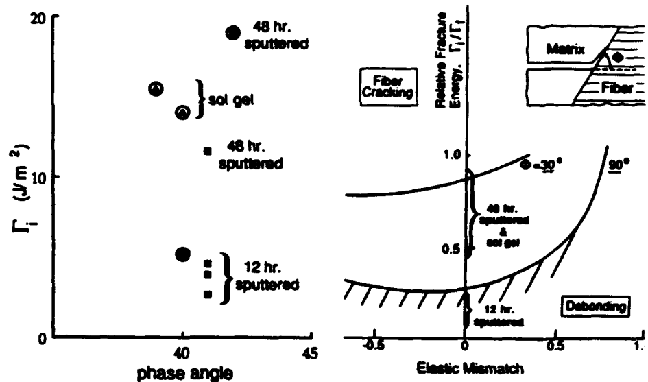
Figure 3. Results of mechanical tests on \text{ZrO}_2 coated interfaces. (Interfacial Cone Crack test results are circled)
