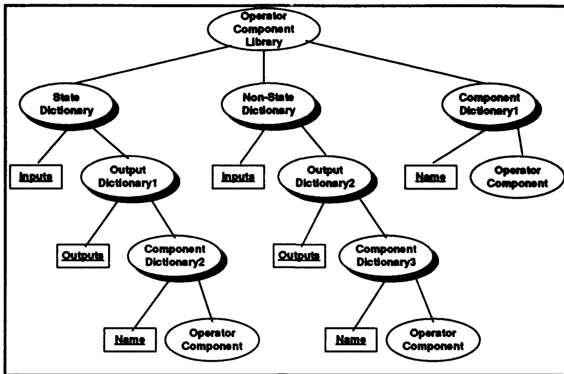
Figure 4 - Operator Component Library
