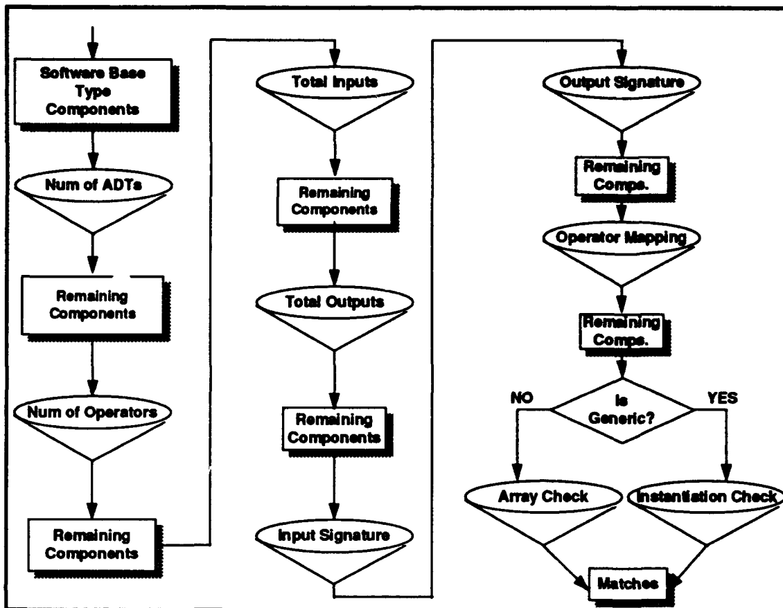
Figure 16 - Filter Process Flow for Types
