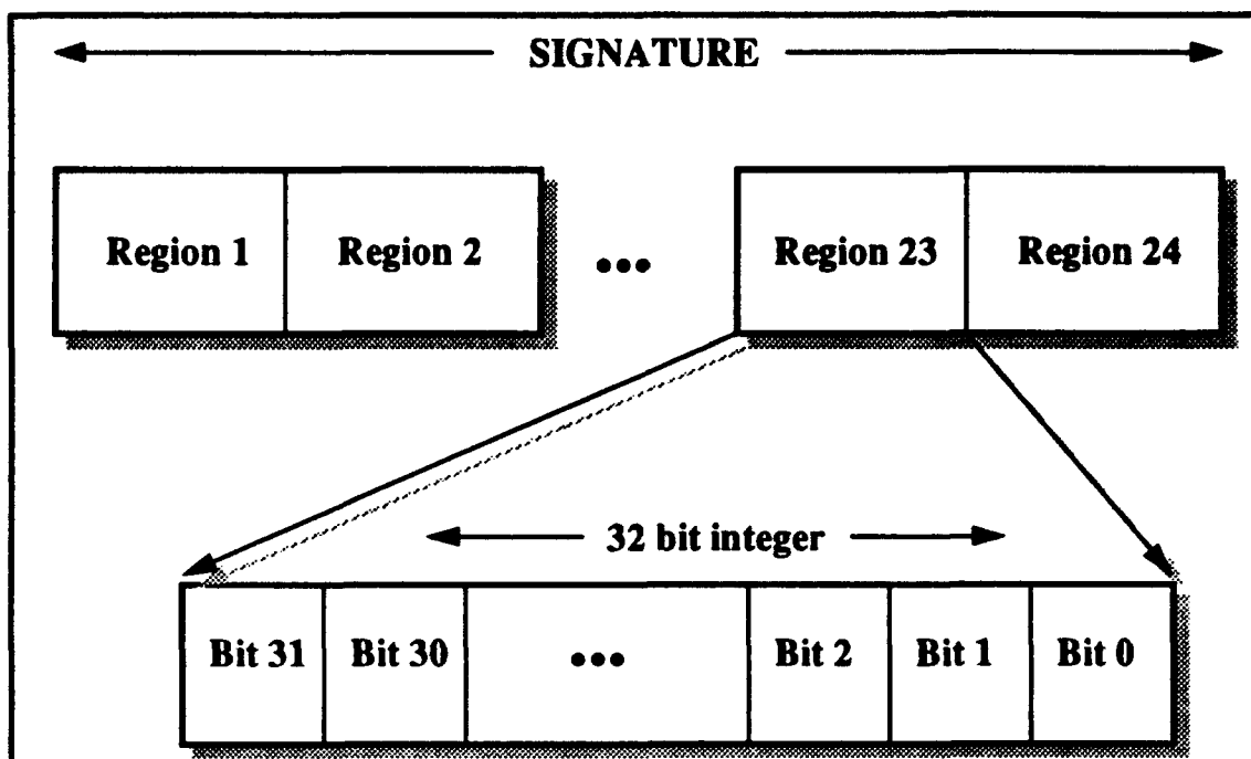
Figure 10 - Graphic Representation of a Signature
