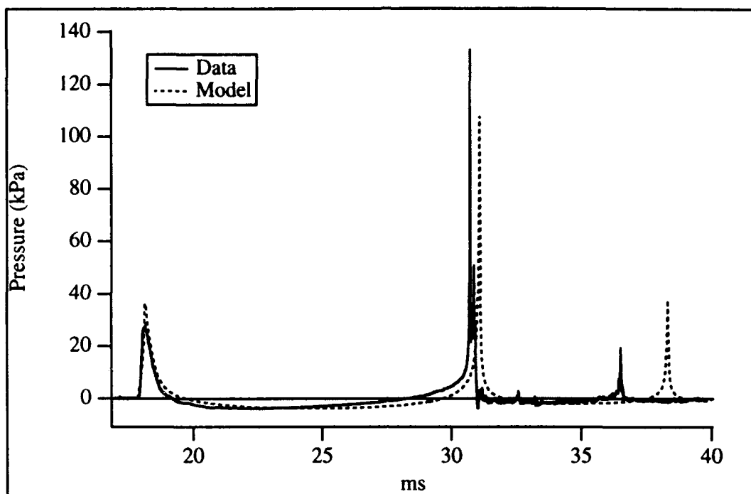
FIGURE 4.3 49 kJ ACOUSTIC SIGNATURE; DEPTH: 55 m
