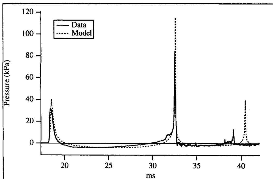
FIGURE 4.4 62.5 kJ ACOUSTIC SIGNATURE; DEPTH: 55 m
