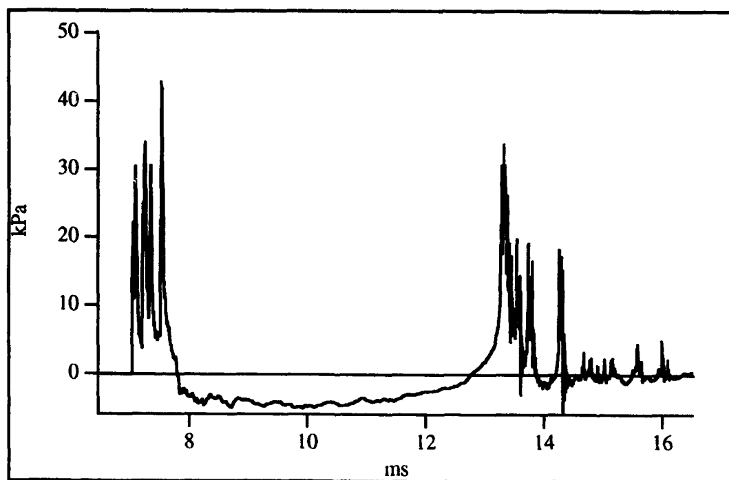
FIGURE 7.4 270 J MEASURED SIGNATURE, SEVEN ELEMENTS AT 0.48 m
