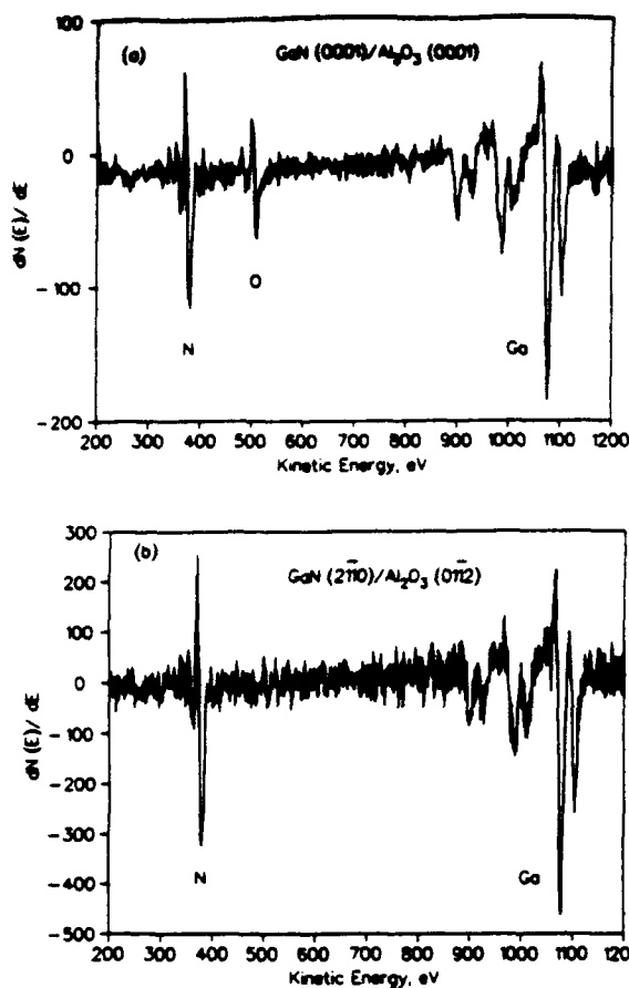
FIG. 2. Auger electron spectra of GaN thin films deposited on (a) (0001) Al 2 O 3 and (b) (0112) Al 2 O 3 substrates.
