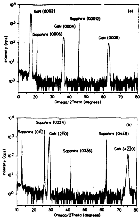
FIG. 3. X-ray diffraction spectra of GaN thin films deposited on (a) (0001) Al 2 O 3 and (b) (0112) Al 2 O 3 substrates.
