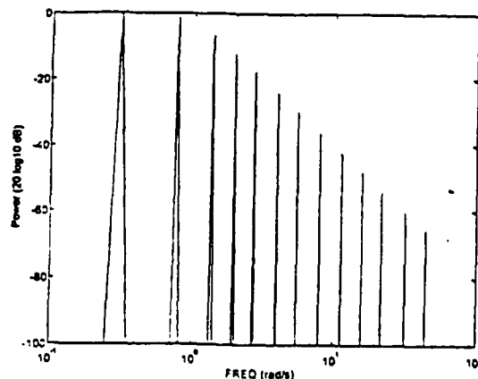
Figure C3: Power Spectral Density of Sum-of Sines Tracking Task
