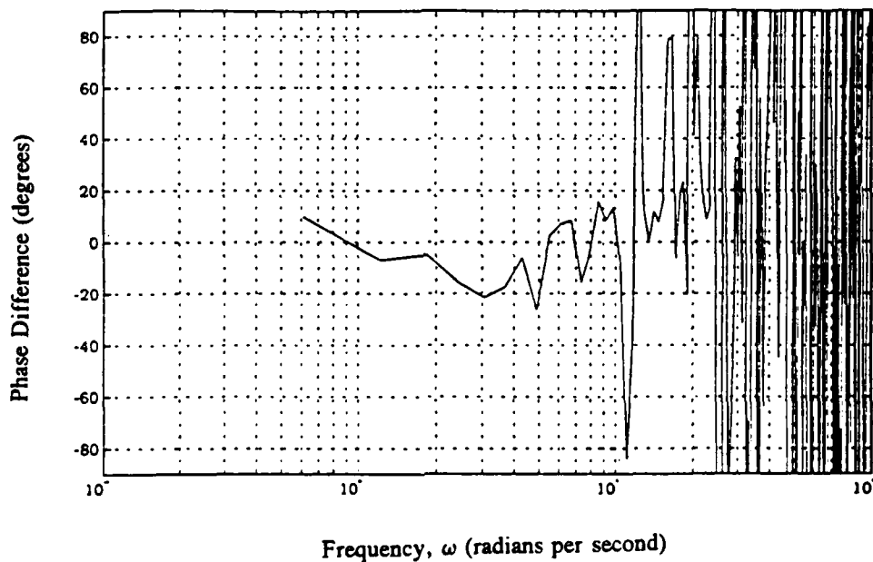
Figure K7: Frequency Response Comparison - Longitudinal Stick Deflection to Task Error (File F1XS_G_1)
