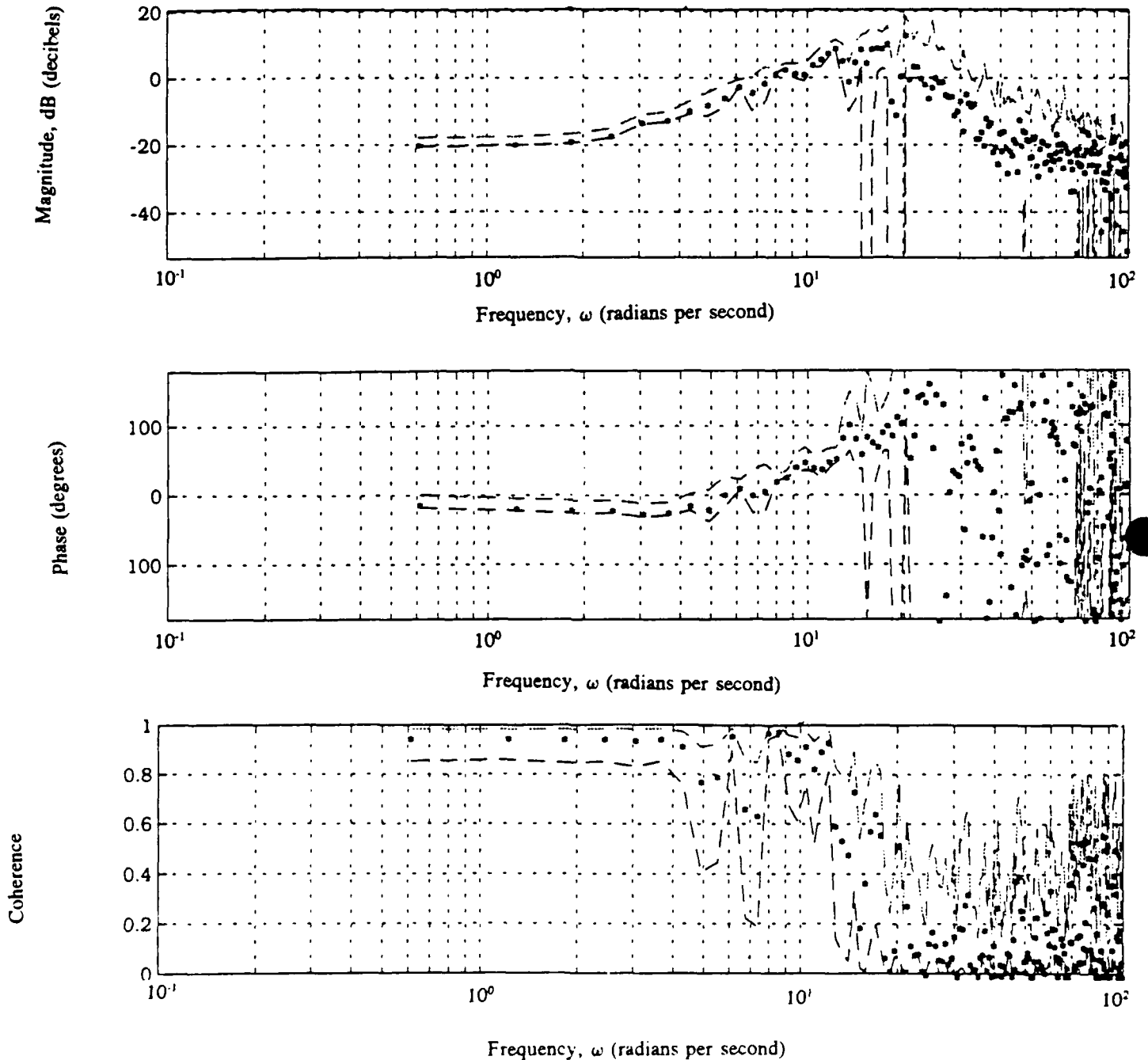
Figure N2: Frequency Response Analysis - Lateral Stick Deflection to Task Error (File F1AS_S_2)
