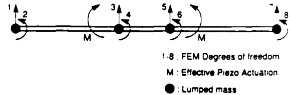
Figure 3. Equivalent FEM representation
