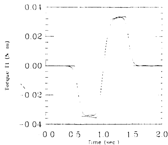
Figure 11. Joint 1 inverse dynamics (—) and rigid (. . . . .) torques
