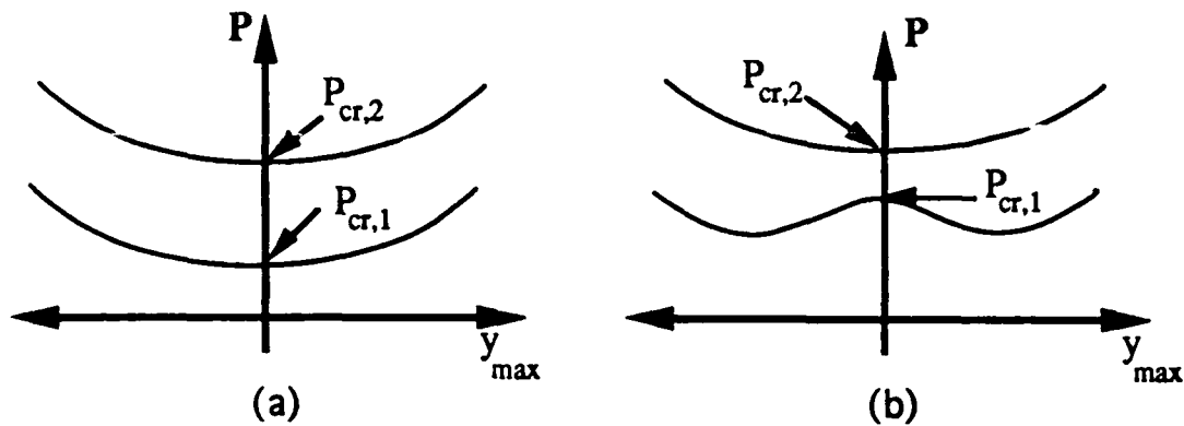
Fig. 3.1. Load deflection curve of a) uncontrolled beam and b) controlled beam.
