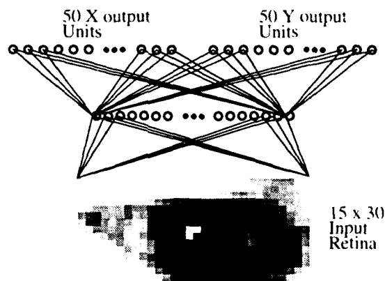
Figure 7. The ANN architecture used. A single, continuous, hidden layer is used. 15 x 30 input retina shown.
