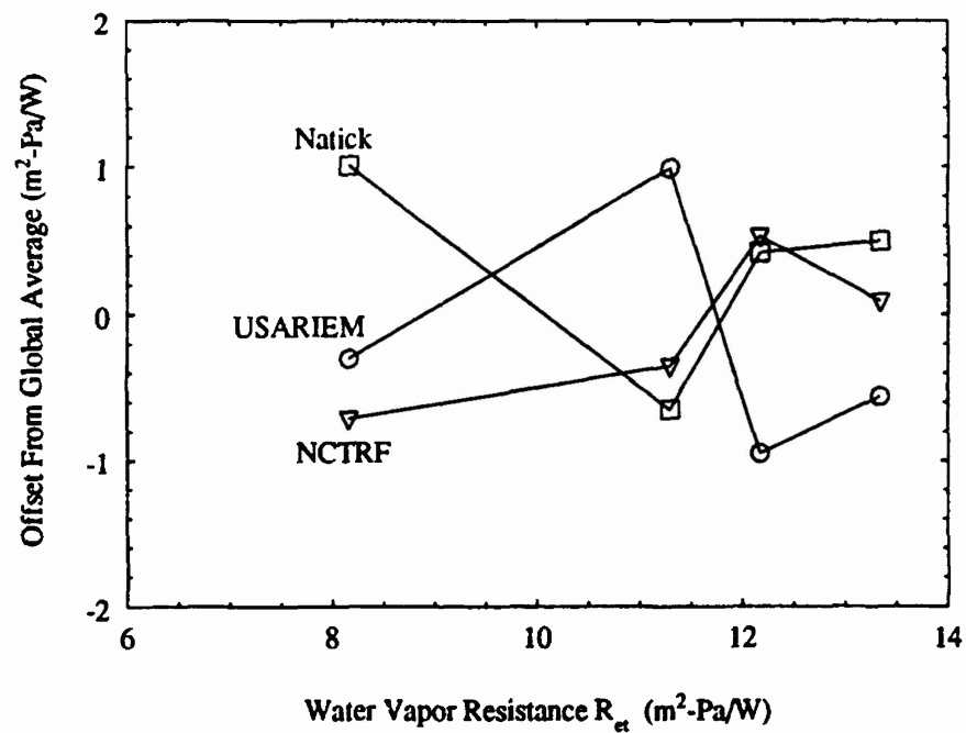
Figure 4. Individual Laboratory Offset From Global Average as Function of Sample Property Level for Water Vapor Resistance R_{vt} (Data from Appendix C).
