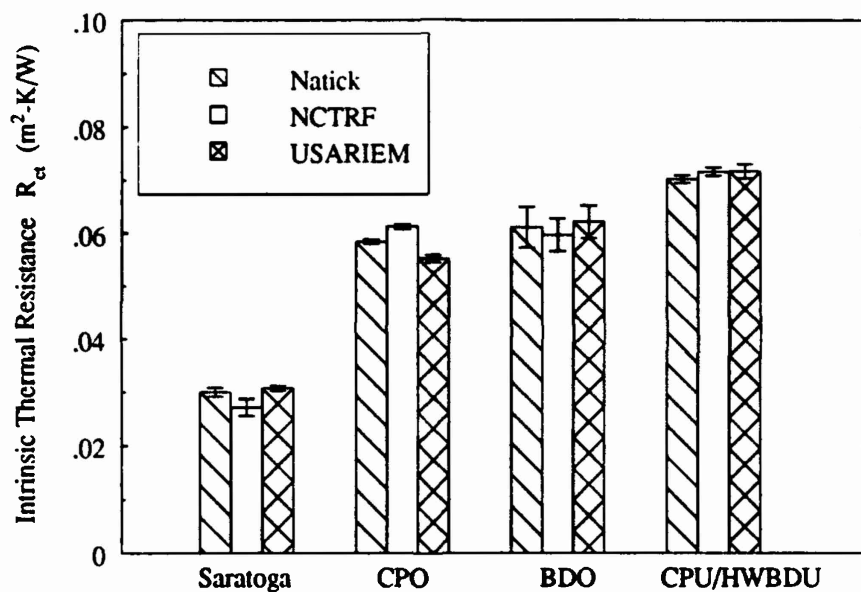
Figure 5. Thermal Resistance of Four Materials Corrected for Offset From Global Average.
