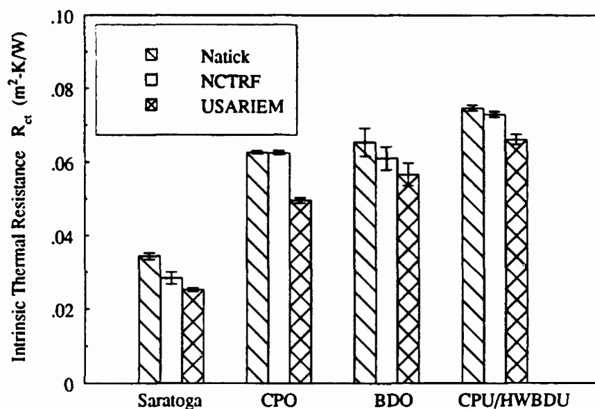
Figure 1. Thermal Resistance of Four Materials as Measured by Three Different Laboratories.
