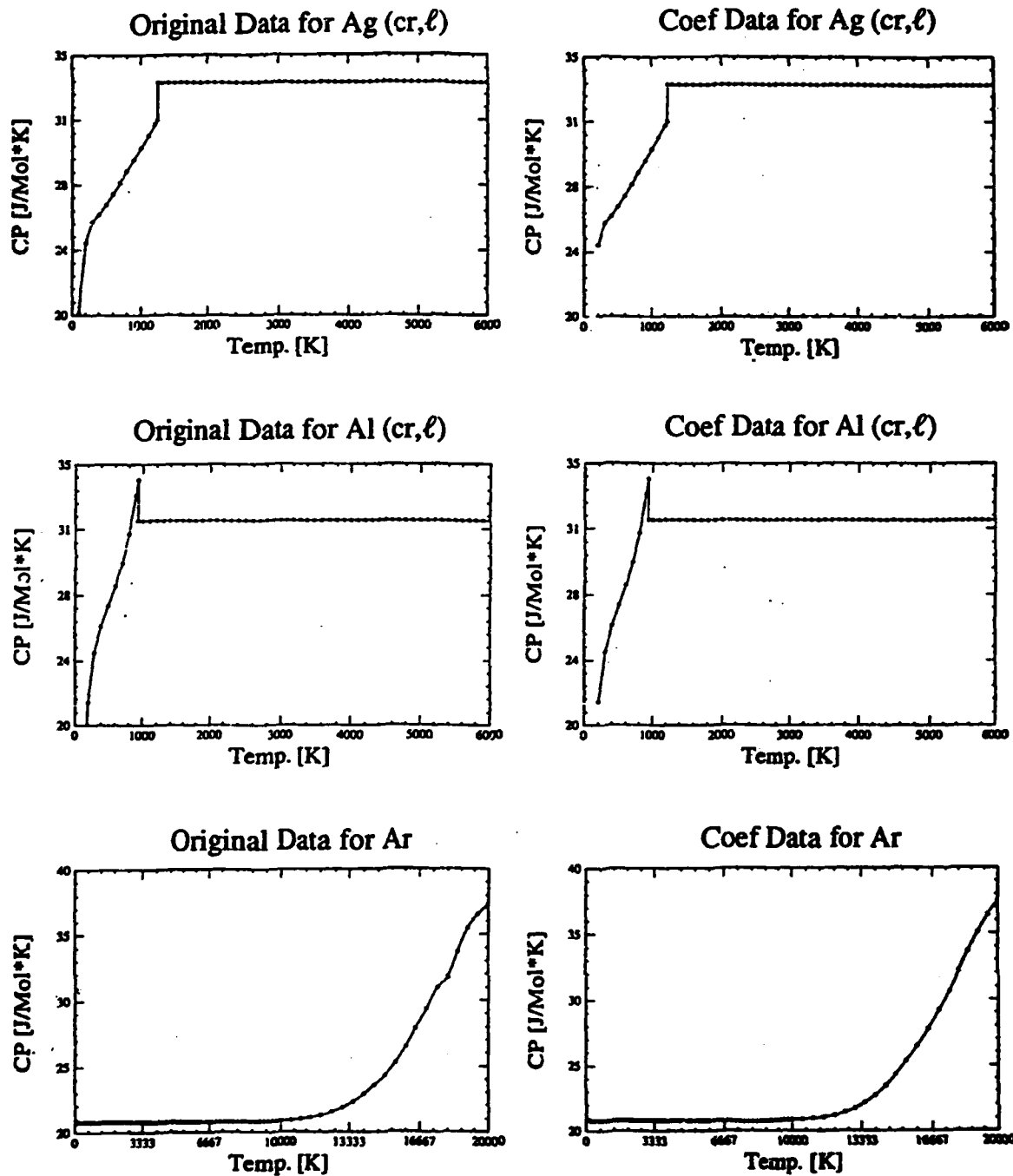
Figure 1.—Comparison of selected (labeled original) C_p values given in table III with values calculated from the 9-constant coefficients given in table VI.
