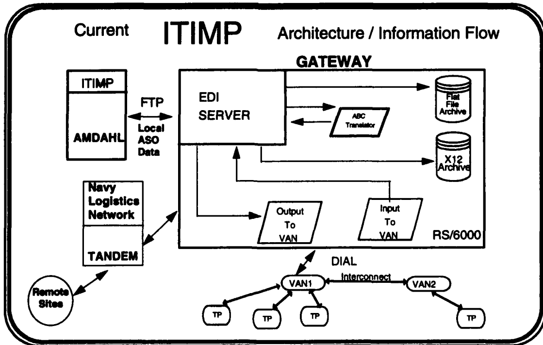
FIGURE 3A
