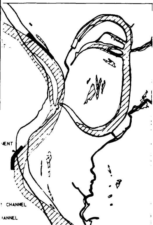
Lower Sunk Lake, Louisiana - Mississippi; the 1965 Lake Mary, Louisiana; and the 1965 Fort Adams, Mississippi - Louisiana topographic map of Louisiana: 1879/1880 Mississippi River Commission charts 59 and 60; 1930/1931 topographical quadrangle, showing historic bankline
