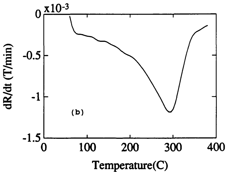
Figure 1b. Derivative of remanence versus time curve in Figure 1a.
