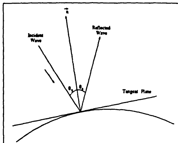
Figure 6: "Local" scattering geometry, [19].
