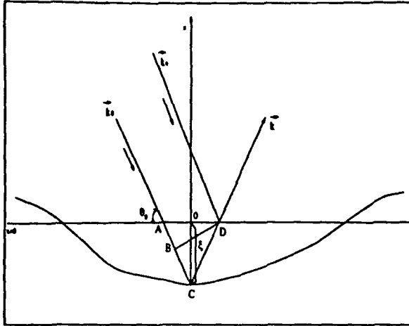
Figure 4: Derivation of the Rayleigh parameter [19].
