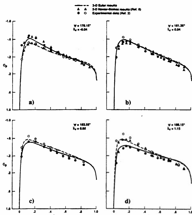
Fig. 8 Comparison of instantaneous surface pressures during parallel blade-vortex interaction for subsonic case ( M_{tip} = 0.6 , \mu = 0.2 , C_k \bar{\Gamma} = 0.133 , x_0 = 0.0 , z_0 = 0.4 , and r_B = 0.893 ).
