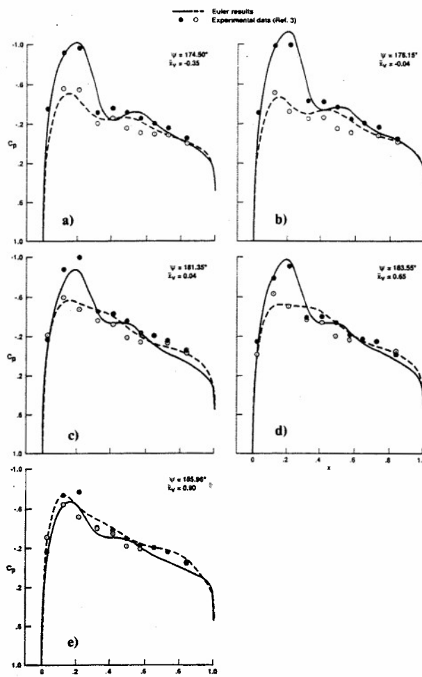
Fig. 9 Comparison of instantaneous surface pressures during parallel blade-vortex interaction for transonic case ( M_{tip} = 0.8 , \mu = 0.2 , C_k \bar{\Gamma} = 0.177 , x_0 = 0.0 , z_0 = 0.4 , and r_B = 0.893 ).
