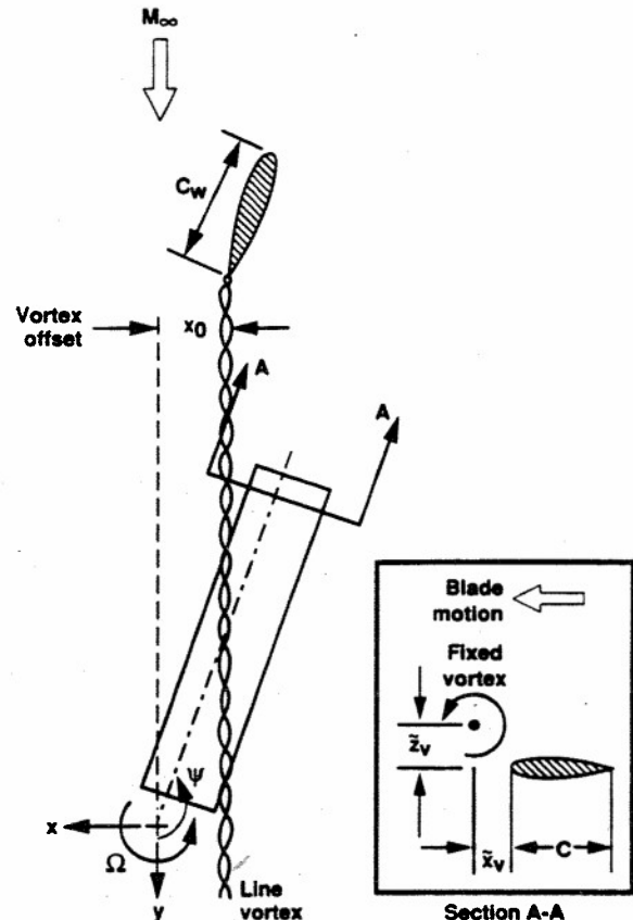
Fig. 2 Schematic of an advancing rotor blade passing a line vortex in a wind-tunnel experiment (Ref. 3).
