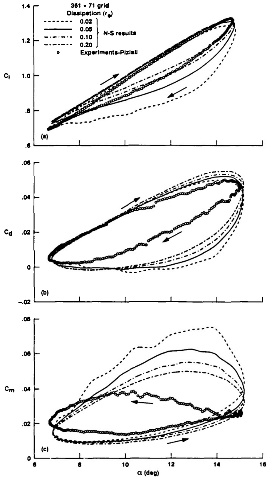
Fig. 41 Effect of numerical dissipation on the solution accuracy with J-K model for the experimental conditions of Fig. 40.
