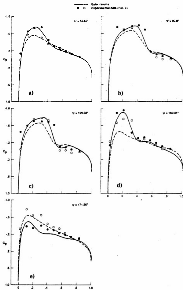
Fig. 10 Comparison of instantaneous surface pressures during oblique blade-vortex interaction for transonic case ( M_{dp} = 0.763 , \mu = 0.197 , C_k \bar{\Gamma} = 0.179 , x_o = -2.13 , z_o = 0.25 , and r_B = 0.946 ).
