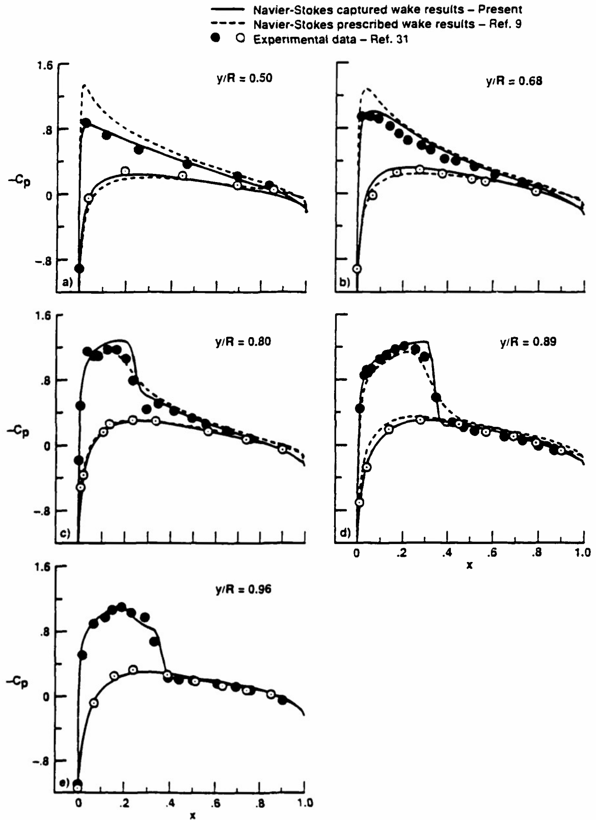
Fig. 3 Comparison of surface pressures for a lifting rotor in hover: M_{tip} = 0.877 , \theta_c = 8^\circ , and Re = 3.93 \times 10^6 .
