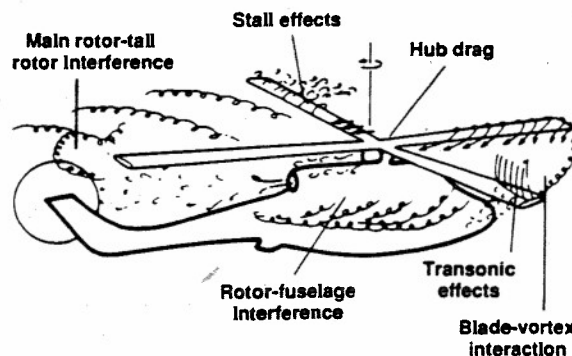
Fig. 1 Schematic of the complex flowfield of a helicopter in forward flight.
