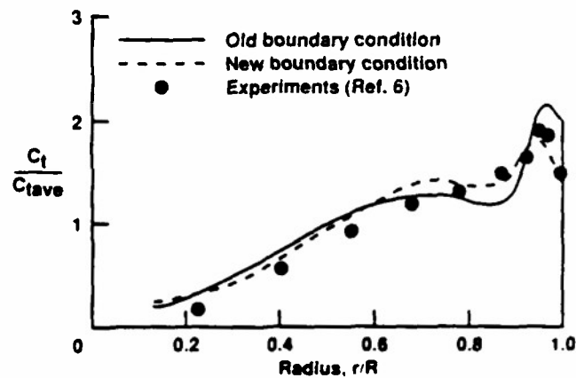
Fig. 30 Sectional thrust distributions for the UH-60A blade with old and new farfield boundary conditions compared with experimental data. M_{t,p} = 0.628 , \theta_r = 9^\circ , and Re = 2.75 \times 10^6 .
