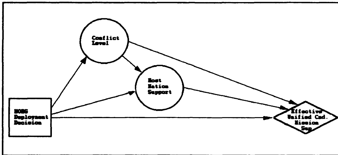
Figure 6 Conflict Level → HSN Influence Diagram.
