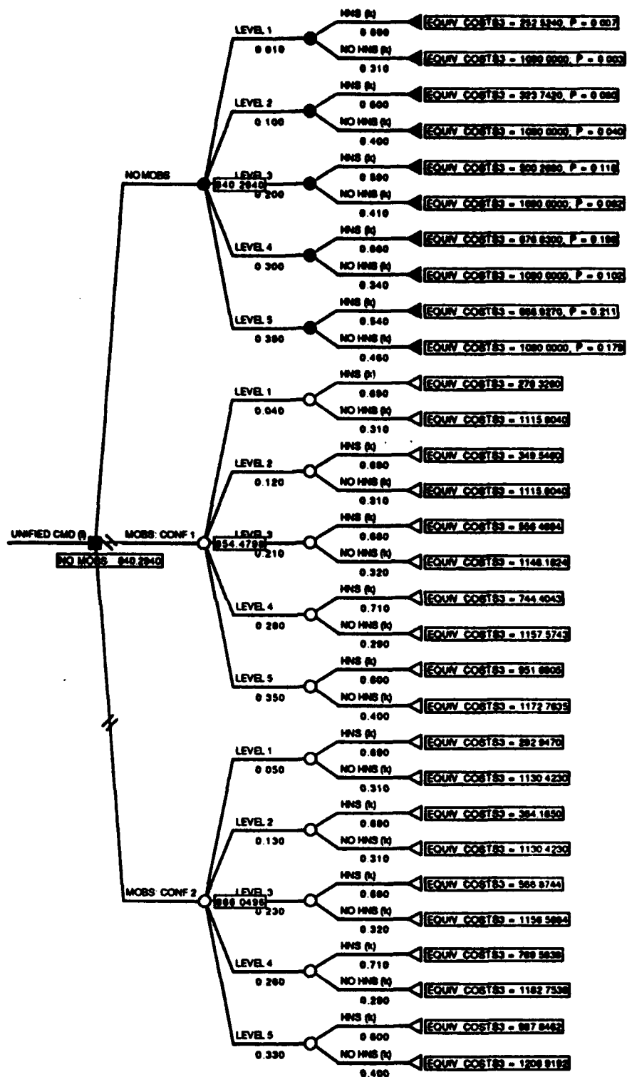
Figure 12 DATA Decision Tree After Rollback
