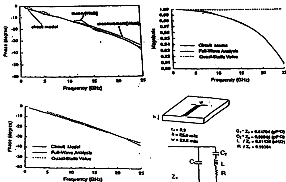
Figure 10 – 13: Equivalent circuit for open end discontinuity
