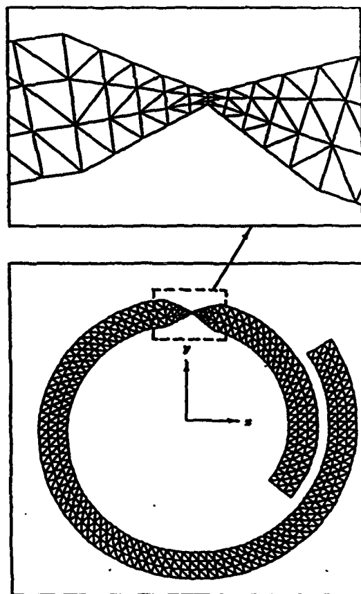
Figure 7: Grid for the monofilar spiral containing 989 interior edges.
