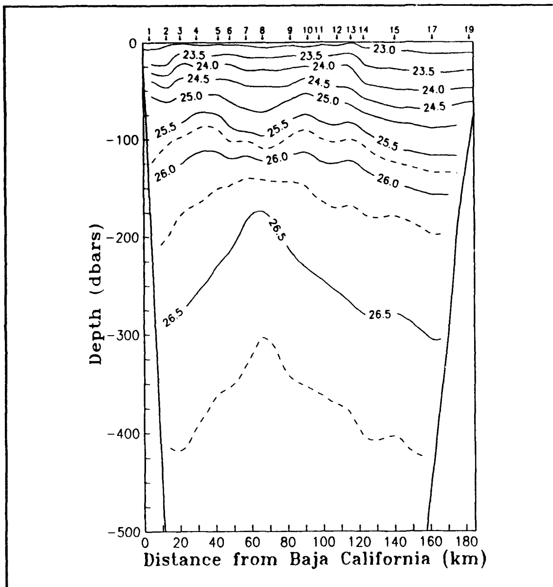
Figure 8(c). Density anomaly. Isopycnal spacing is 0.25 \text{ kg/m}^3 or as labeled.
