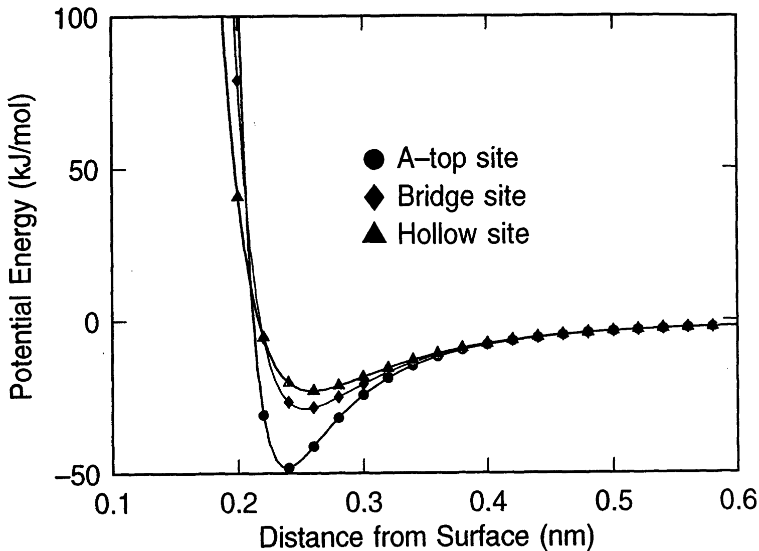
Fig. 1 Water-Pt(100) interaction
