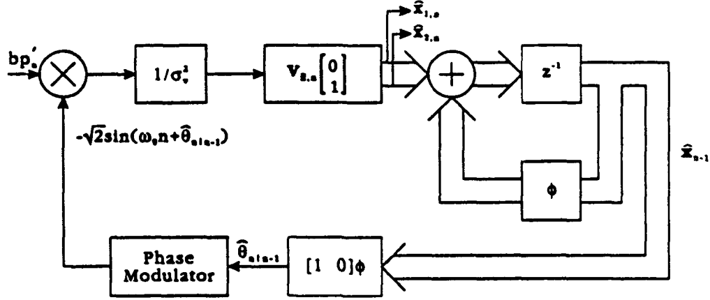
Figure 6: State space representation of the DPLL.
