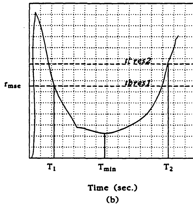
Figure 13: Illustration of the adaptive Kalman filter process.
