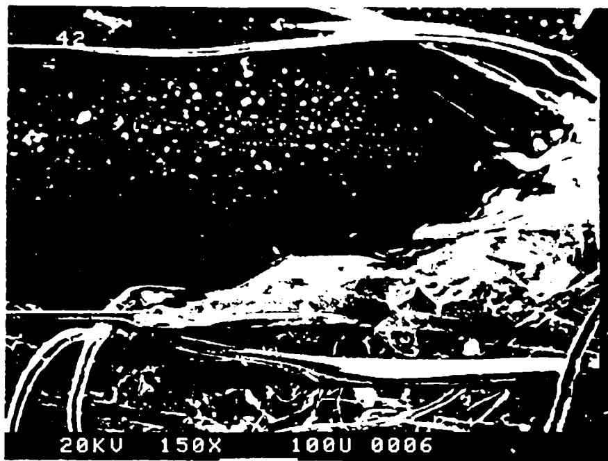
Figure 4.25. Electron Photomicrograph of Sample 42 Adherend After Room Temperature Wedge Test, Highlighting the Adhesive-Debonded Region Interface.
