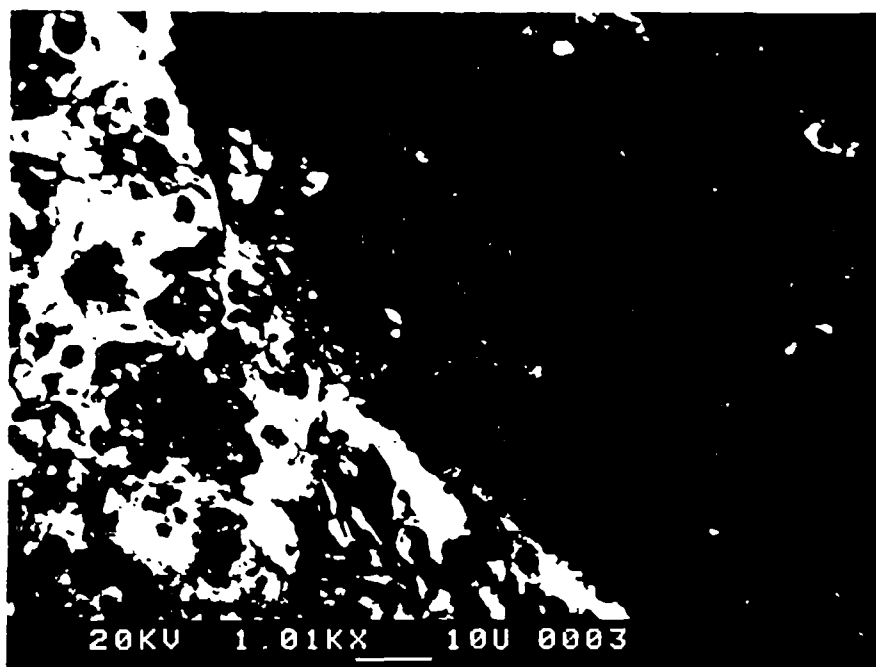
Figure 4.5 Electron Photomicrograph of Sample 14 Adherend After Room Temperature Wedge Test.
