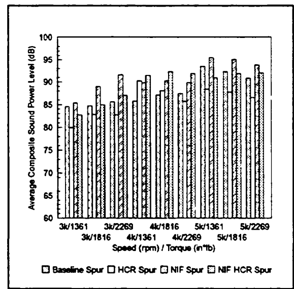
Figure 21 - Tooth Form Effect
