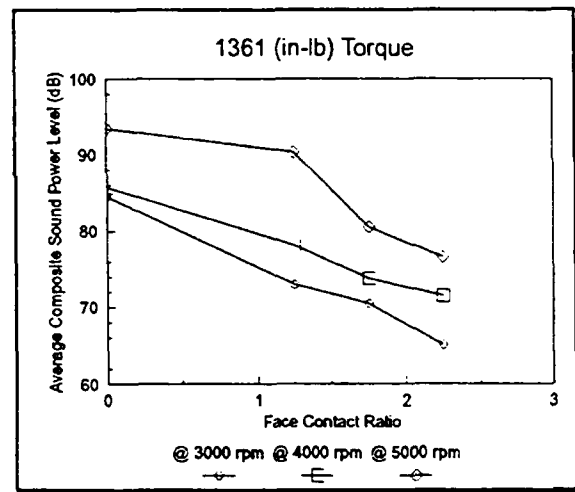
Figure 17 - Face Contact Ratio Effect Low Torque
