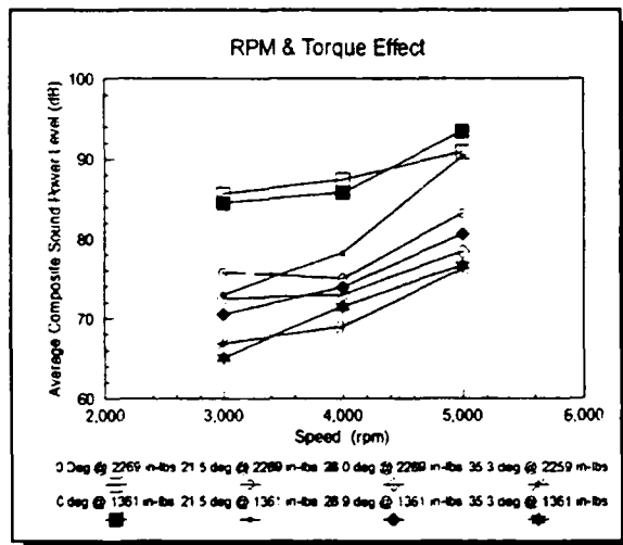
Figure 16 - Combined Speed & Torque Effects
