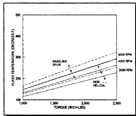
Figure 9 - Flash Temperature v Torque
