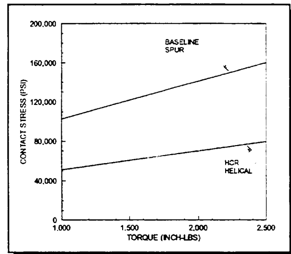
Figure 8 - Contact Stress v Torque
