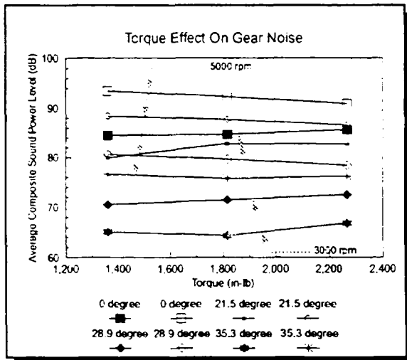
Figure 15 - Torque Effect On Gear Noise
