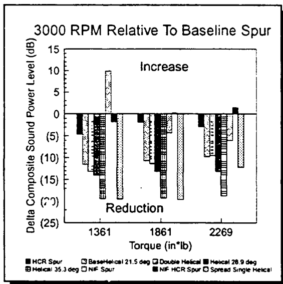
Figure 22 - 3,000 RPM Noise Summary
