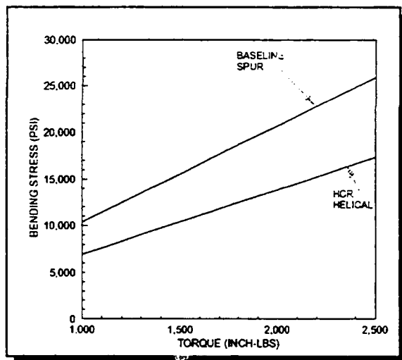
Figure 7 - Bending Stress v Torque
