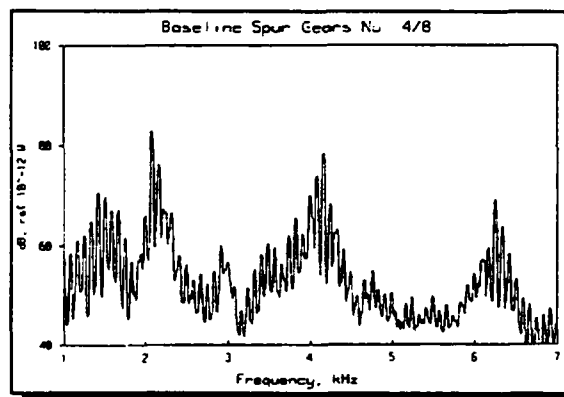
Figure 5 - Baseline Spur Spectrum
