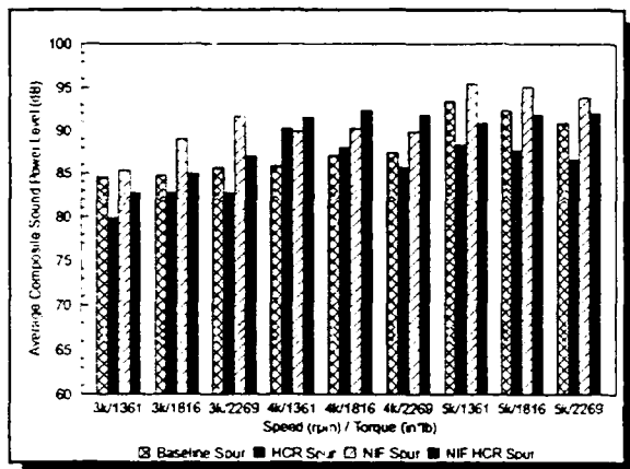
Figure 11 - Spur Gear Noise Levels
