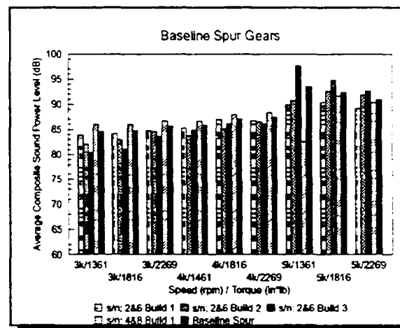
Figure 13 - Spur Gear Build Variations
