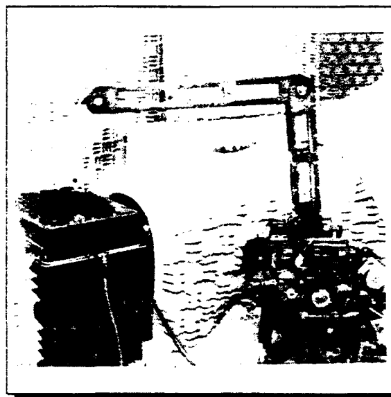
Figure 4 - Robot Noise Measurement System
