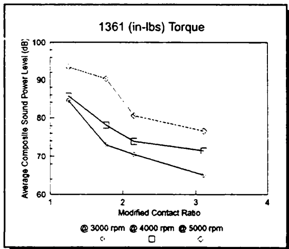
Figure 19 - Modified Contact Ratio Effect
