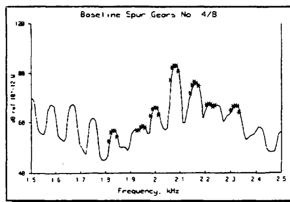
Figure 6 - Enlargement of Figure 5 (Around First Harmonic)
