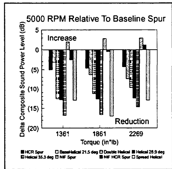
Figure 24 - 5,000 RPM Noise Summary
