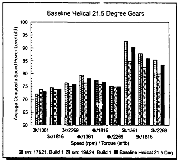
Figure 14 - Helical Gear Build Variations
