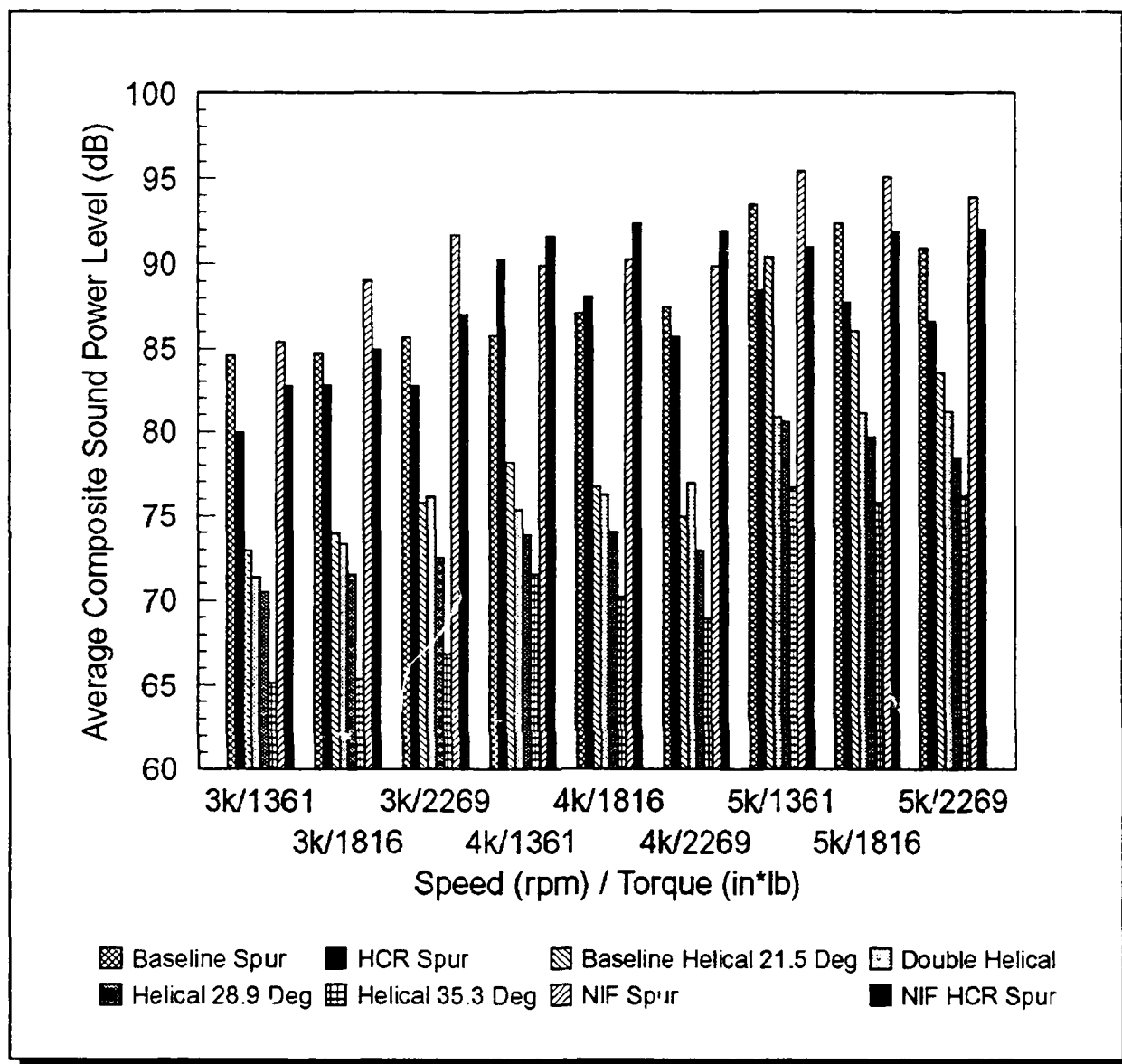
Figure 10 - Summary Of Test Results
