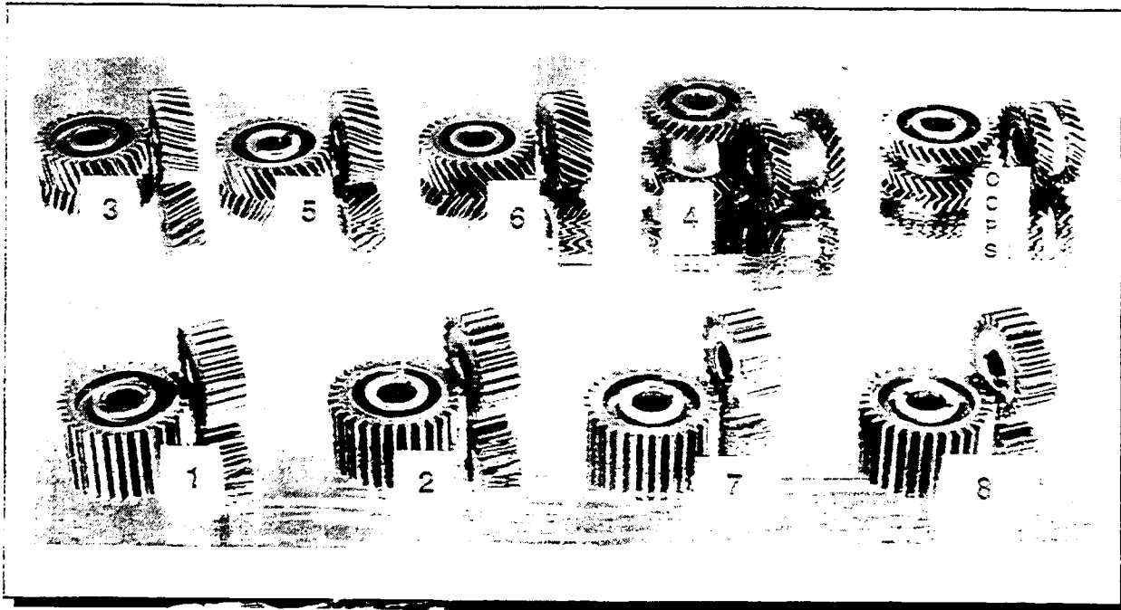
Figure 1 - Test Gears
