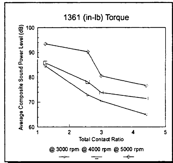
Figure 20 - Total Contact Ratio Effect
