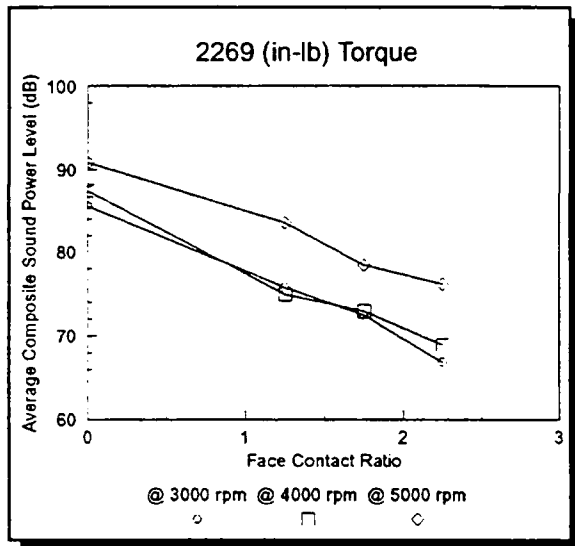
Figure 18 - Face Contact Ratio Effect High Torque
