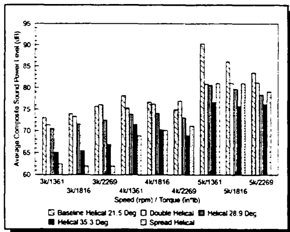
Figure 12 - Helical Gear Noise Levels
