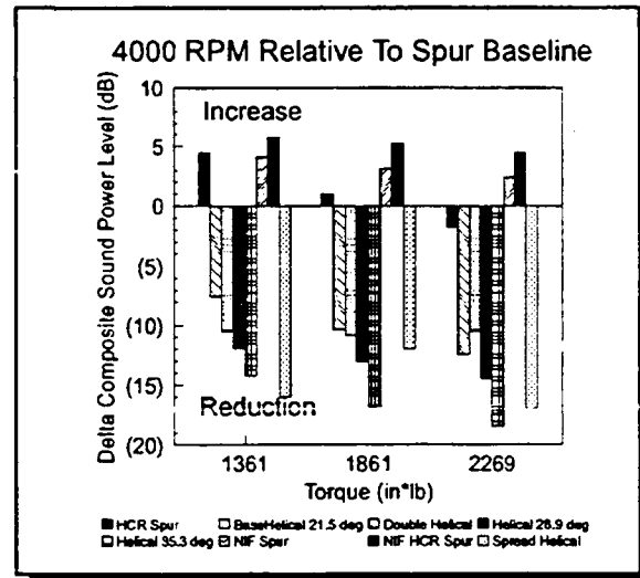
Figure 23 - 4,000 RPM Noise Summary
