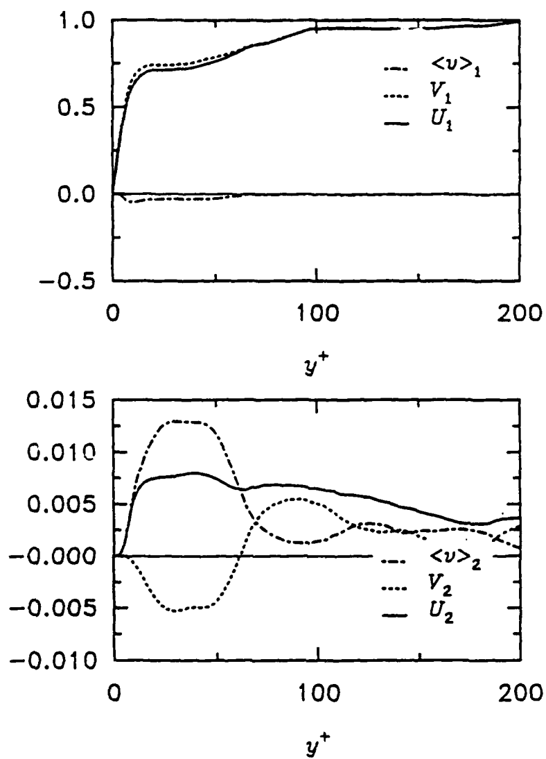
Figure 1. The Reynolds mean, Favre mean and Favre fluctuation mean velocity profiles.
