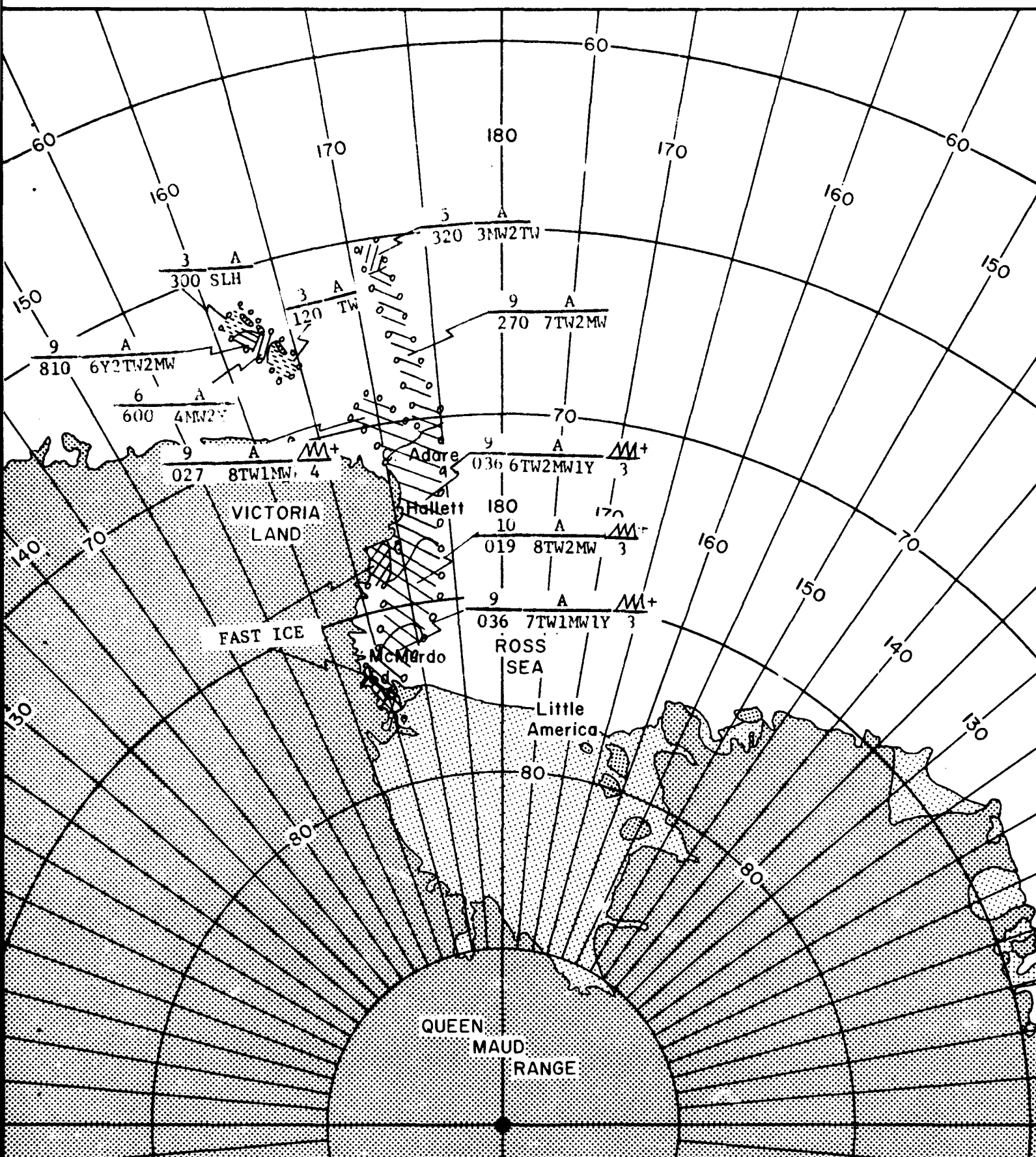
FIGURE 3 OBSERVED ICE CONDITIONS 3-8 OCTOBER 1966
