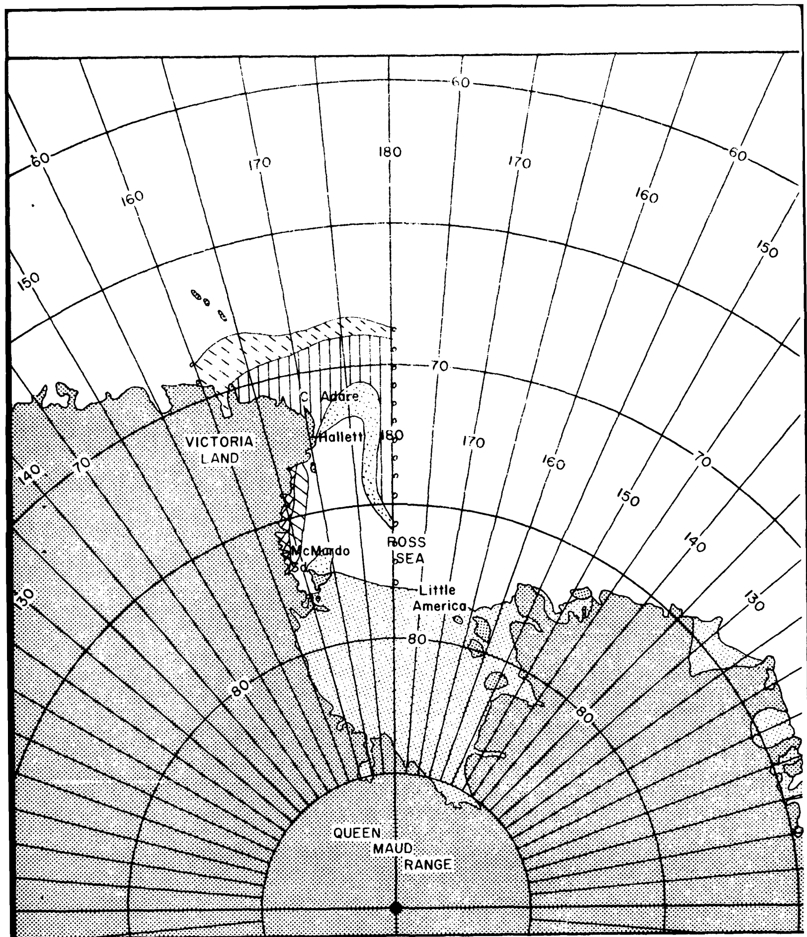
FIGURE 7 PROGNOSTIC ICE CHART MID-JANUARY 1967
