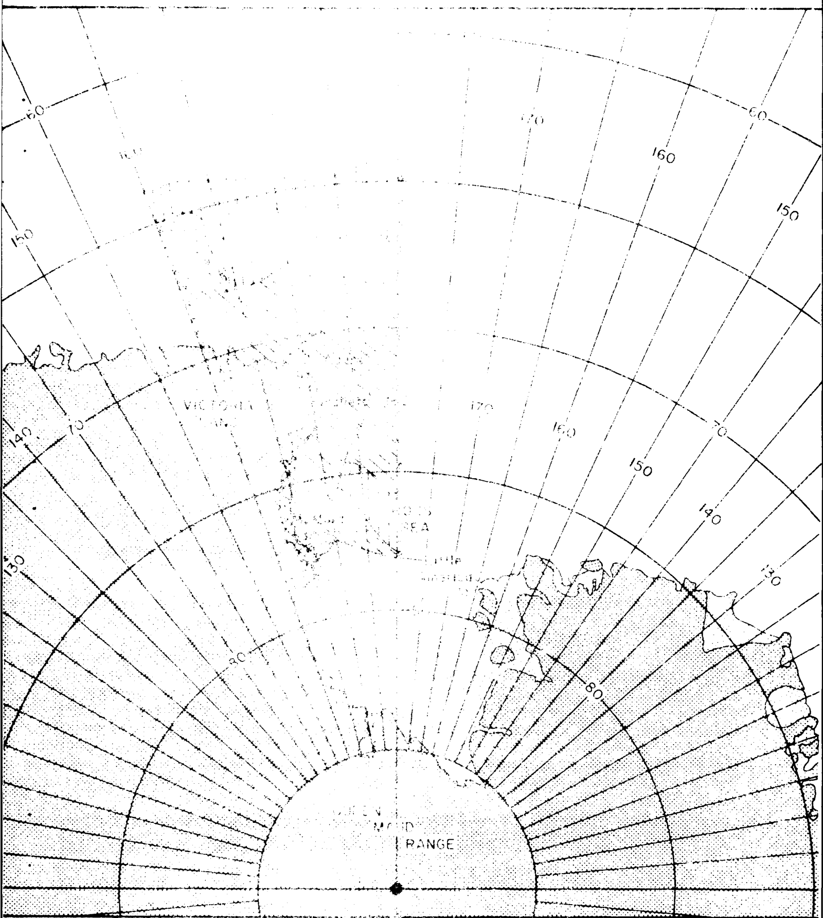
FIGURE 5 PROGNOSTIC ICE CHART MID-NOVEMBER 1966
