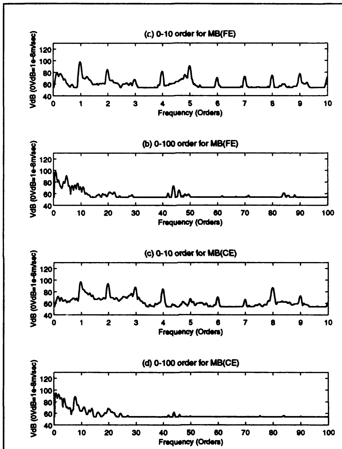
Figure 24 The Narrow Band Spectra for Type I Fire Pumps Using NAVSSES Frequency Domain Data Measured at MB(FE) and MB(CE)
