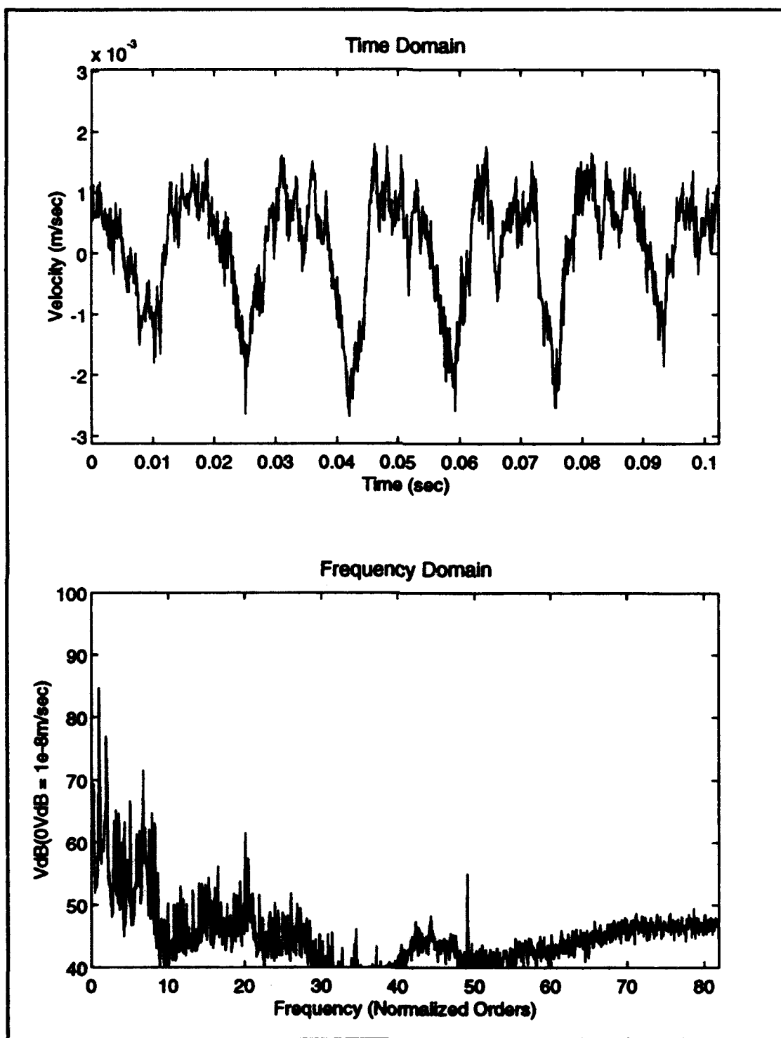
Figure 10 Typical Time Series and Frequency Spectrum of Type II Fire Pumps Measured at MB(FE)
