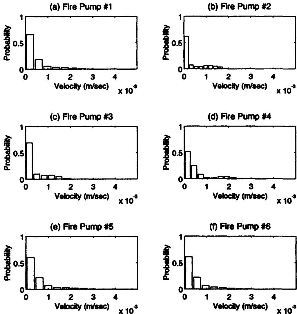
Figure 12 The Probability Distributions of Cross Peak Data for Type I (10/30/89) Fire Pumps Measured at MB(FE)
