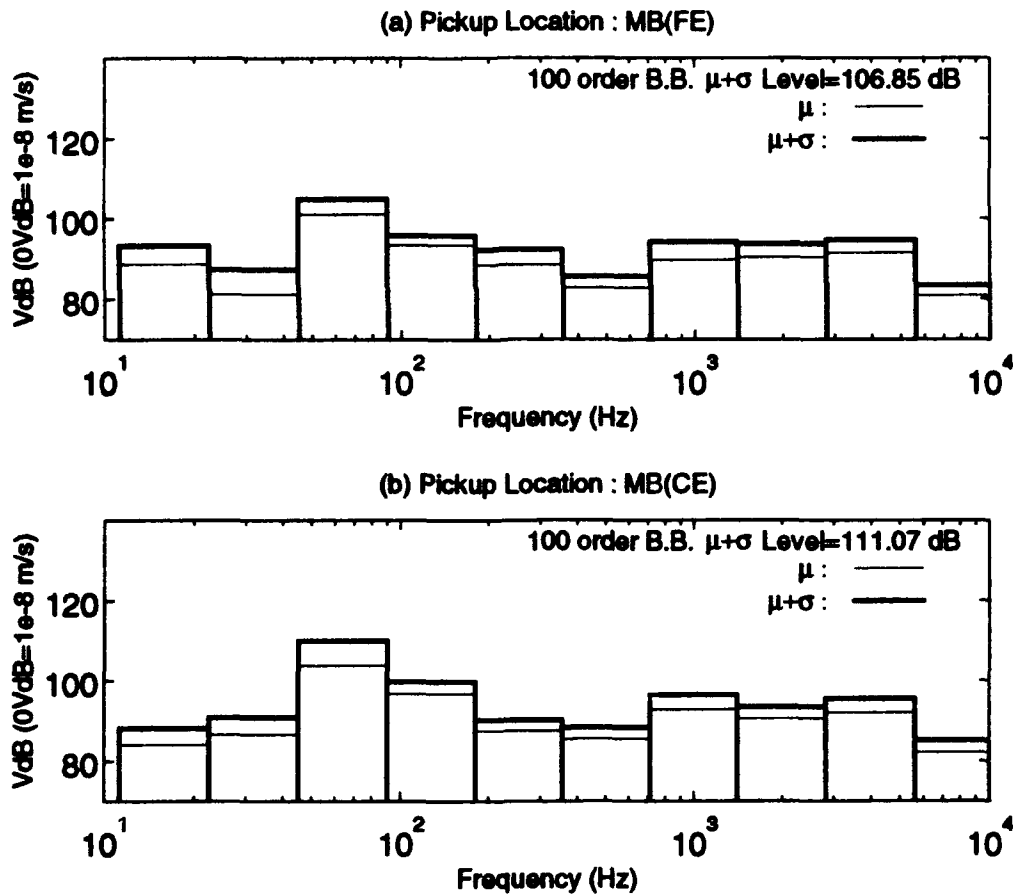
Figure 23 The Summarized 1/1 Octave Band Levels for Type I Fire Pumps Using NAVSSES Frequency Domain Data
