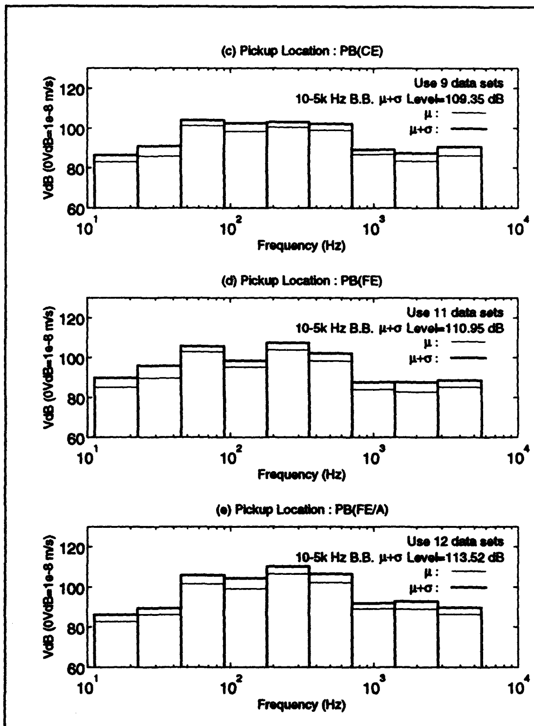
Figure 14 The Summarized 1/1 Octave Band Levels for Type I Fire Pumps (Cont.)
