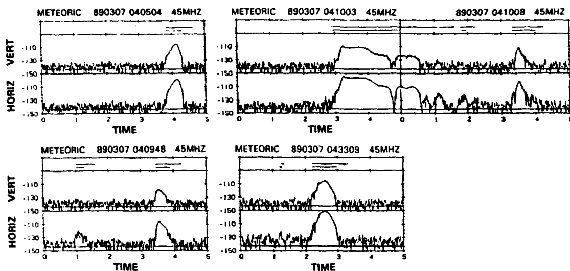
Figure 6. Examples of Returns from Overdense Trails.
