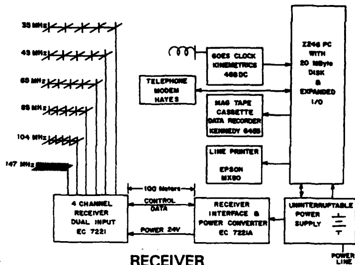
Figure 2. Block Diagrams of HLMSTB Instrumentation for the Sondrestrom AB-Thule AB Link.
