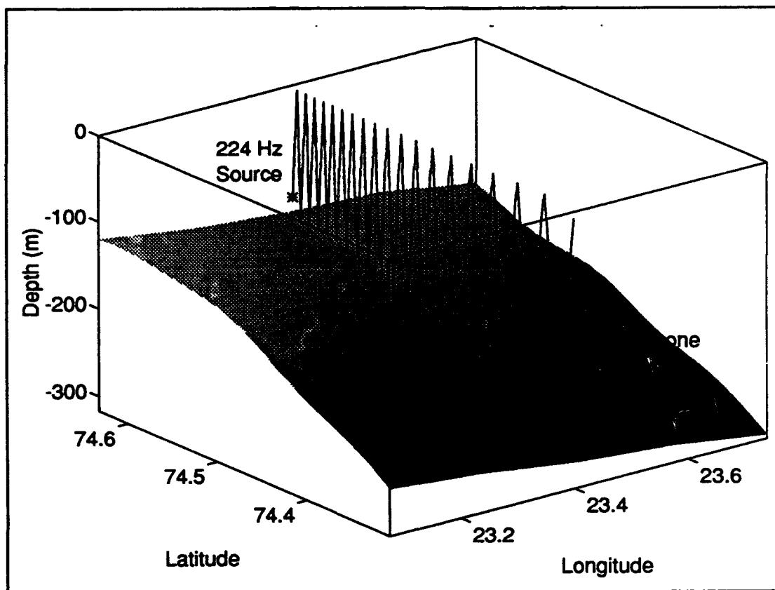
Figure 11. Three dimensional representation of the region of study. Superimposed on this figure are the locations of the 224 Hz source and the hydrophone array as well as a bottom interacting ray path.
