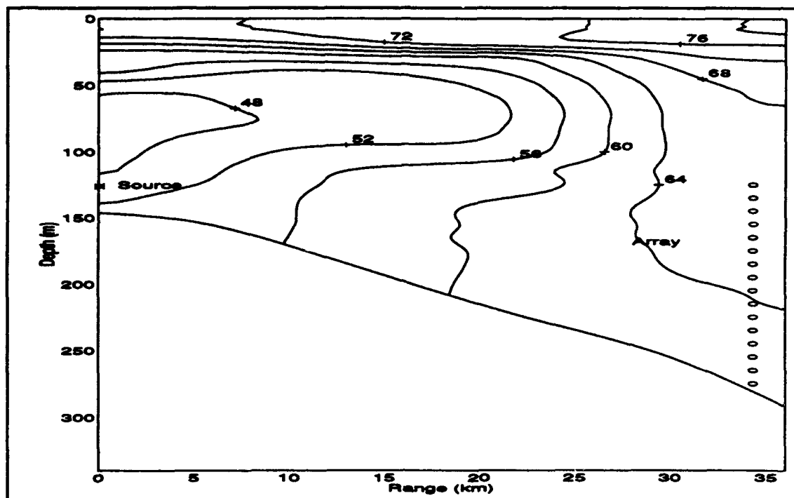
Figure 8. Sound speed contour along the line of sight between the source and receiver. (+1400 m/s)
