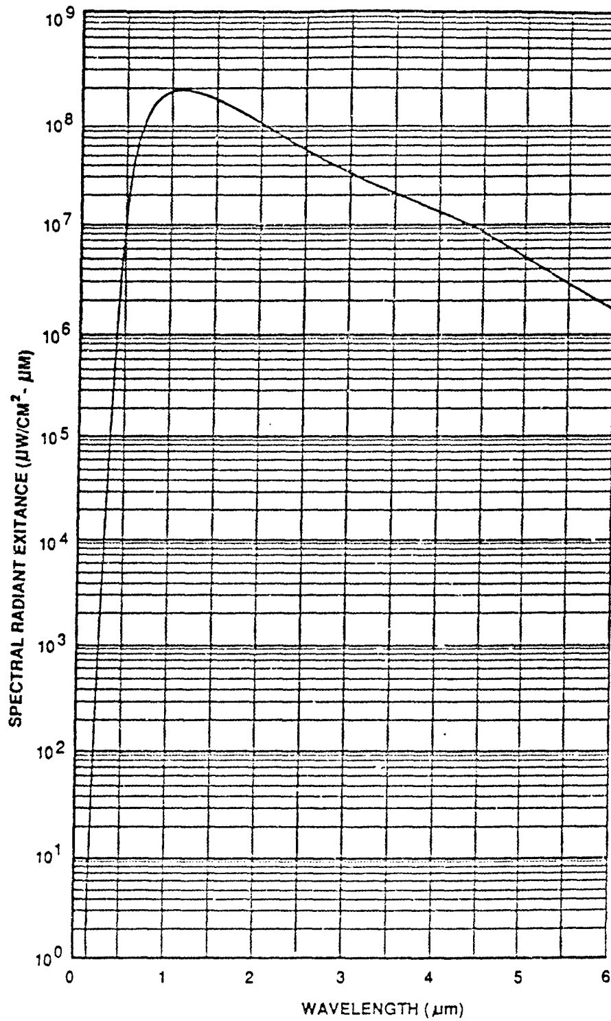
Figure 27 BLACKBODY RADIATION CURVE AT 2700°K
