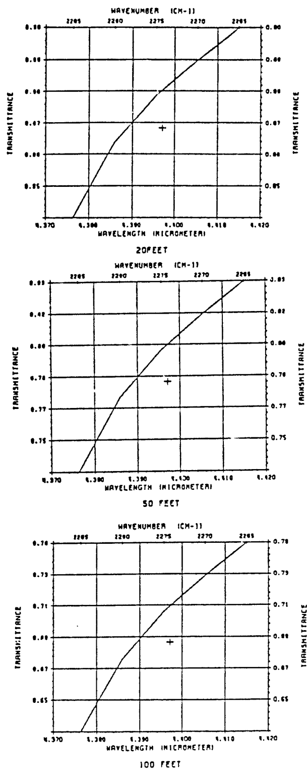
Figure 10. Atmospheric Transmittance in the IR Region of Interest over Distances of 20, 50 and 100 feet, respectively.
