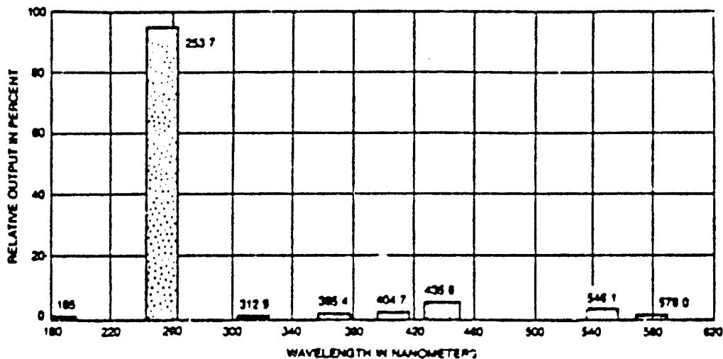
(a) Relative Spectral Distribution of Energy Emitted by Ozone-Producing Germicidal Lamps
