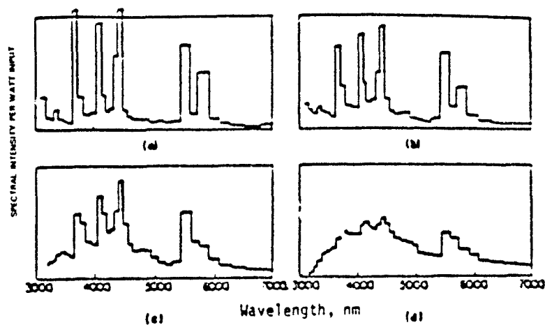
Figure 19. Emission Spectrum of High-Pressure Mercury Arc Lamps Showing Continuous Background: (a) 31 atm; (b) 75 atm; (c) 165 atm; (d) 285 atm. (Noel, 1941)
