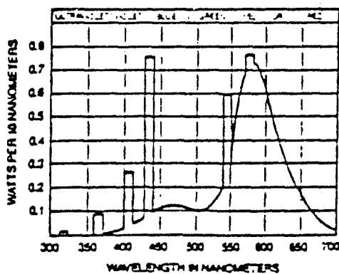
(c) Warm White F40WW
