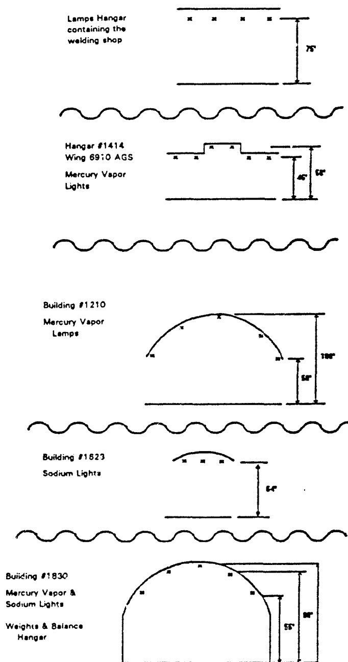
Figure 5. Typical Placement of High-intensity Discharge Lamps in AF Hangars/Facilities
