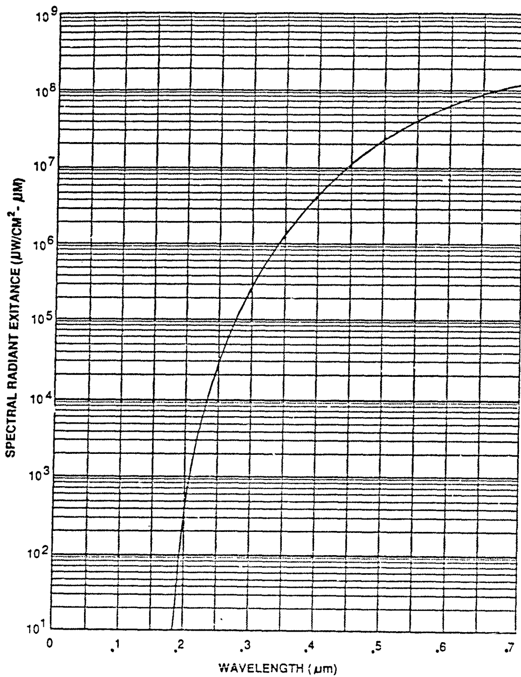
Figure 26 BLACKBODY RADIATION CURVE AT 2700°K
