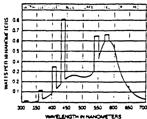
(b) Cool White F40CW
