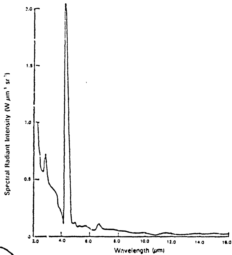
Figure 3. Far Infrared Emissions from JP-4 Burning at Sea Level
