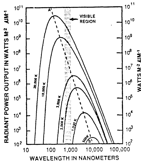
Figure 25. Blackbody Radiation Curves for Operating Temperatures between 500°K and 20,000°K Showing Wien Displacement of Peaks. Shaded Area is Region of Visible Wavelengths.
