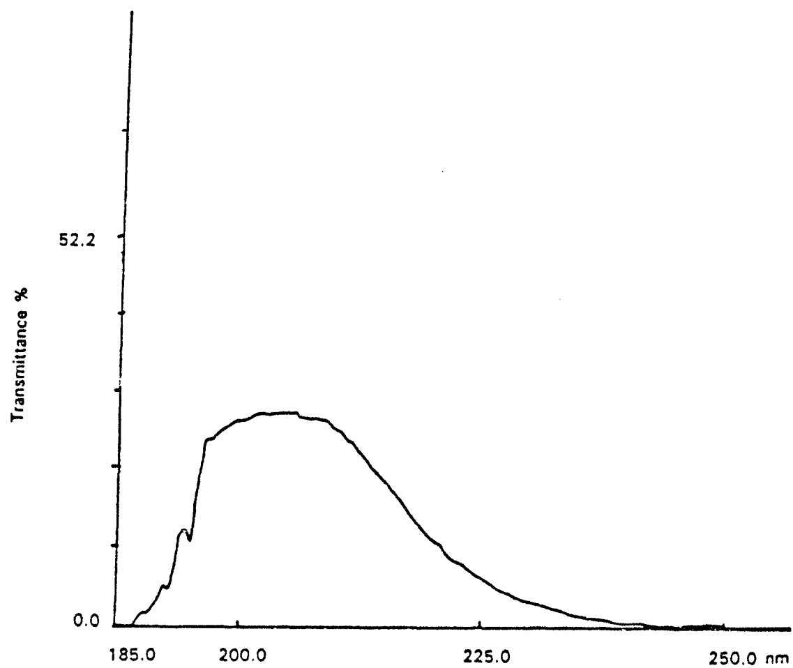
Figure 7. Transmittance of UV Filter
