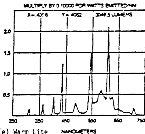
Figure 21. Spectral Output of Several Types of Fluorescent Lamps
