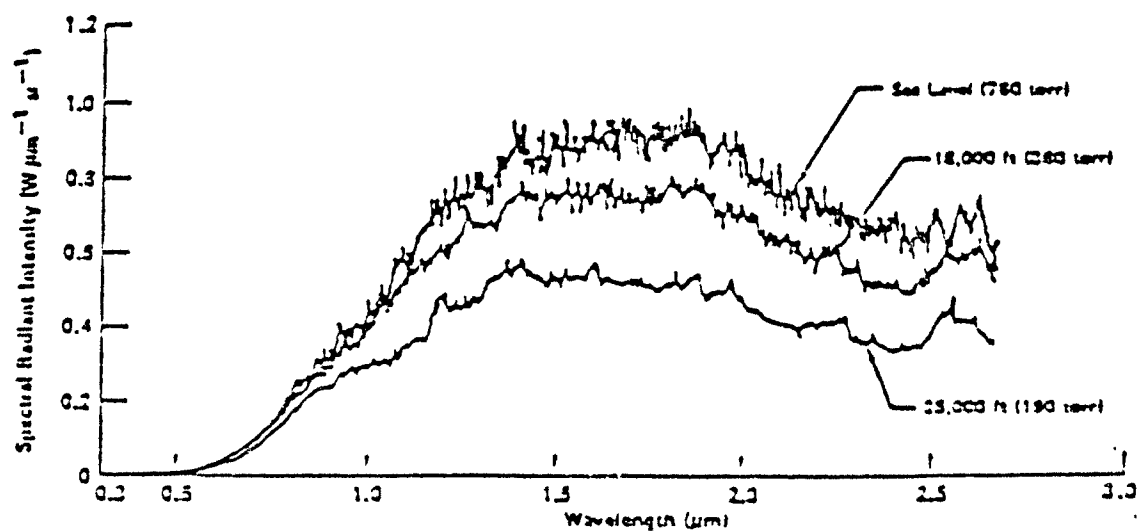
Figure 2. Visible and Near Infrared Emissions from JP-4 Burning at Various Altitudes
