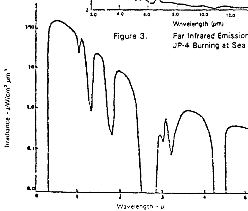
Figure 4. Spectral Irradiance vs. Wavelength for Solar Radiation
