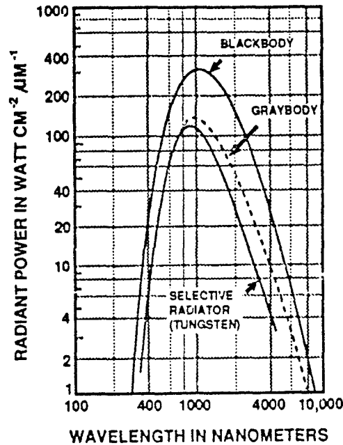
Figure 24. Radiation Curves for Blackbody, Graybody, and Selective Radiators Operating at 3000°K.
