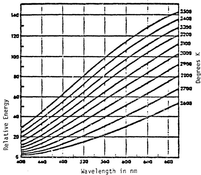
Figure 28. Spectral Power Distribution in the Visible Region from Tungsten Filaments of Equal Wattage but Different Temperatures.
