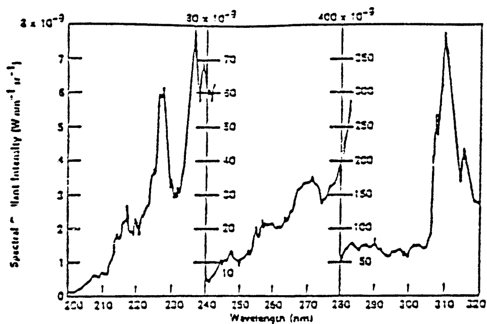
Figure 1. Spectral Radiant Intensity of JP-4 Burning at Sea Level (200-320 nm)
