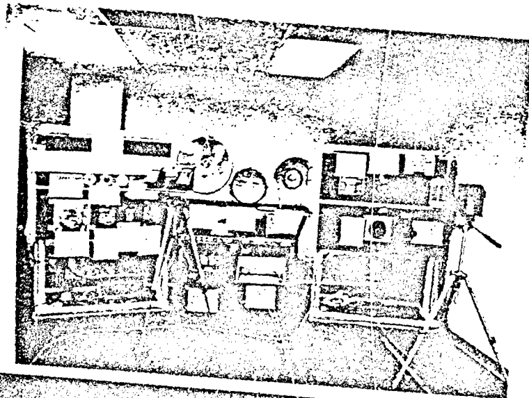
Figure 34. Lights and hot bodies used in lab measurements.
