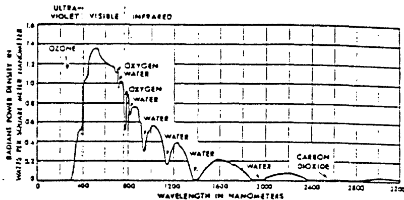
Figure 30. Spectral Distribution of Solar Radiant Power Density at Sea Level Showing Ozone, Oxygen, Water and Carbon Dioxide Absorption Bands.
