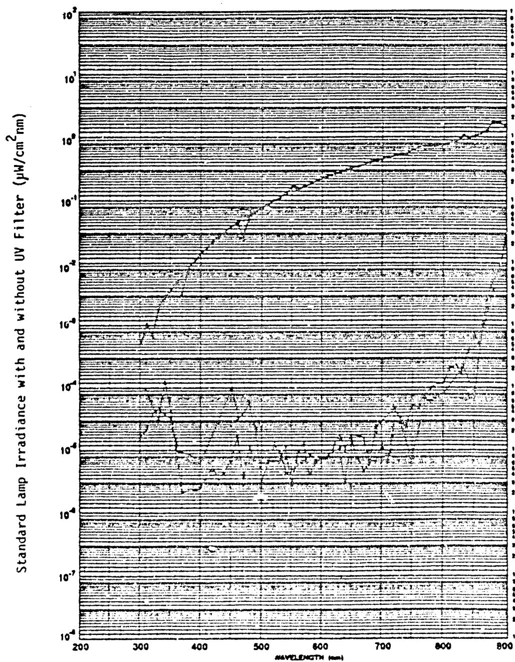
Figure 8. Comparison of UV Filter Transmittance of Standard Lamp Irradiance with No Filter Signal and Dark Current of Absolute Spectroradiometer System
