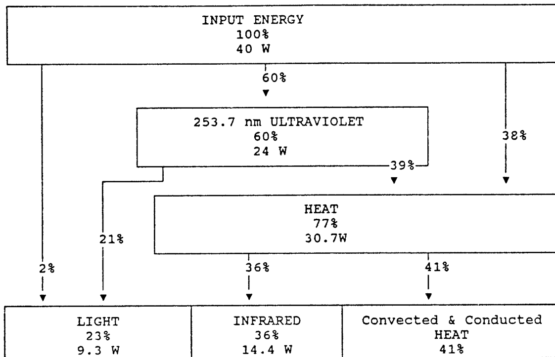
Figure 22. Energy Distribution of A Typical 40-Watt Cool White Fluorescent Lamp.
