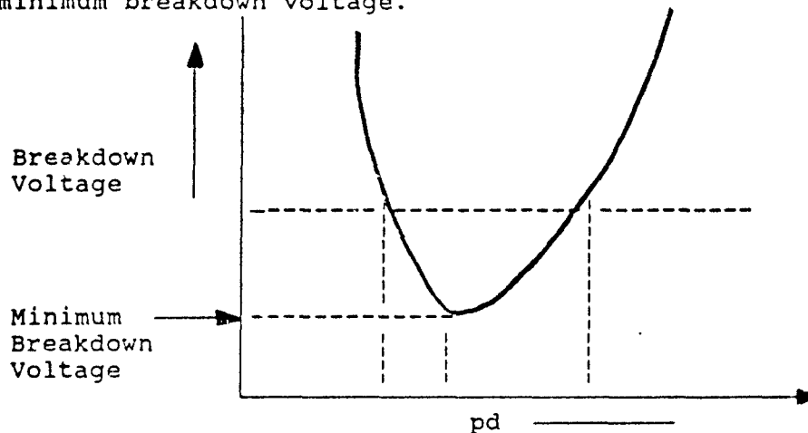
Figure 12 Paschen's Law
