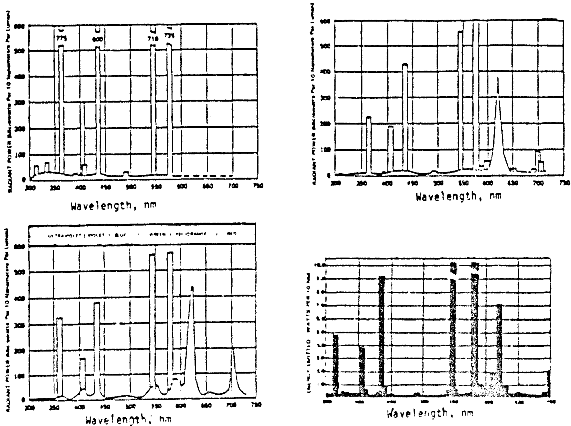
Figure 20. Spectral Output of High Pressure Mercury Lamps: (a) Clean; (b) deluxe; (c) Warm Deluxe; (d) White White Deluxe (H33GL-400 DX) as used in the Older 2-Lamp Lightall Units
