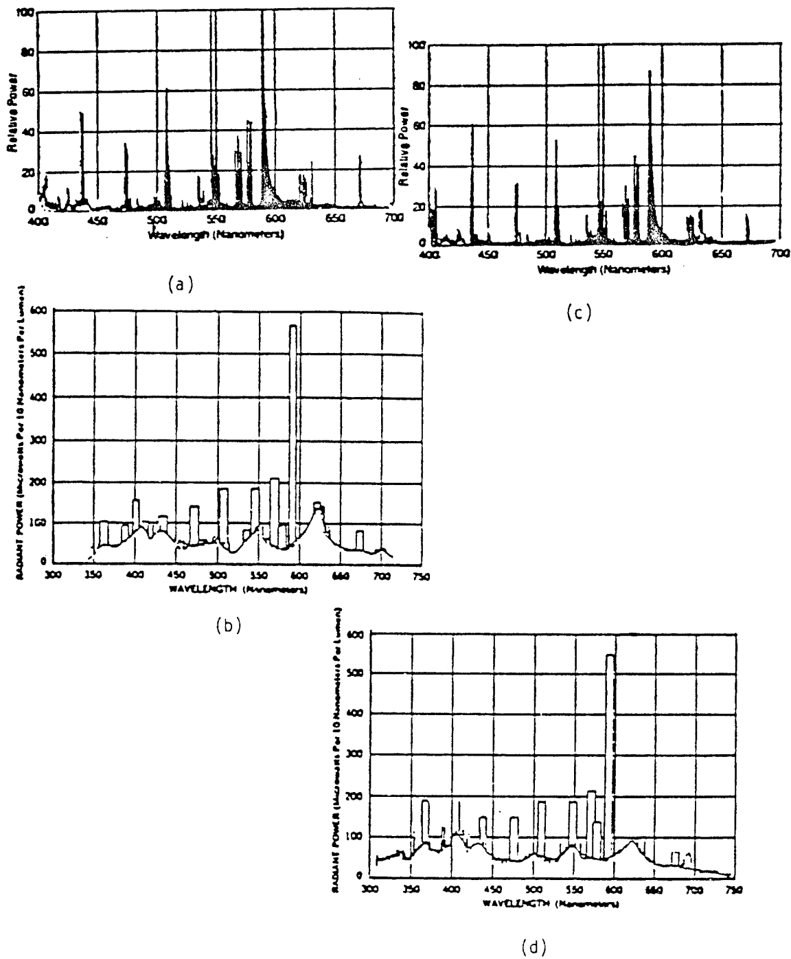
Figure 14. High Pressure Multivapor Metal Halide Lamps Spectral Output: (a) and (b): Metal Halide Lamps-Clear; (c) and (d): Metal Halide Lamps-Phosphor Coated
