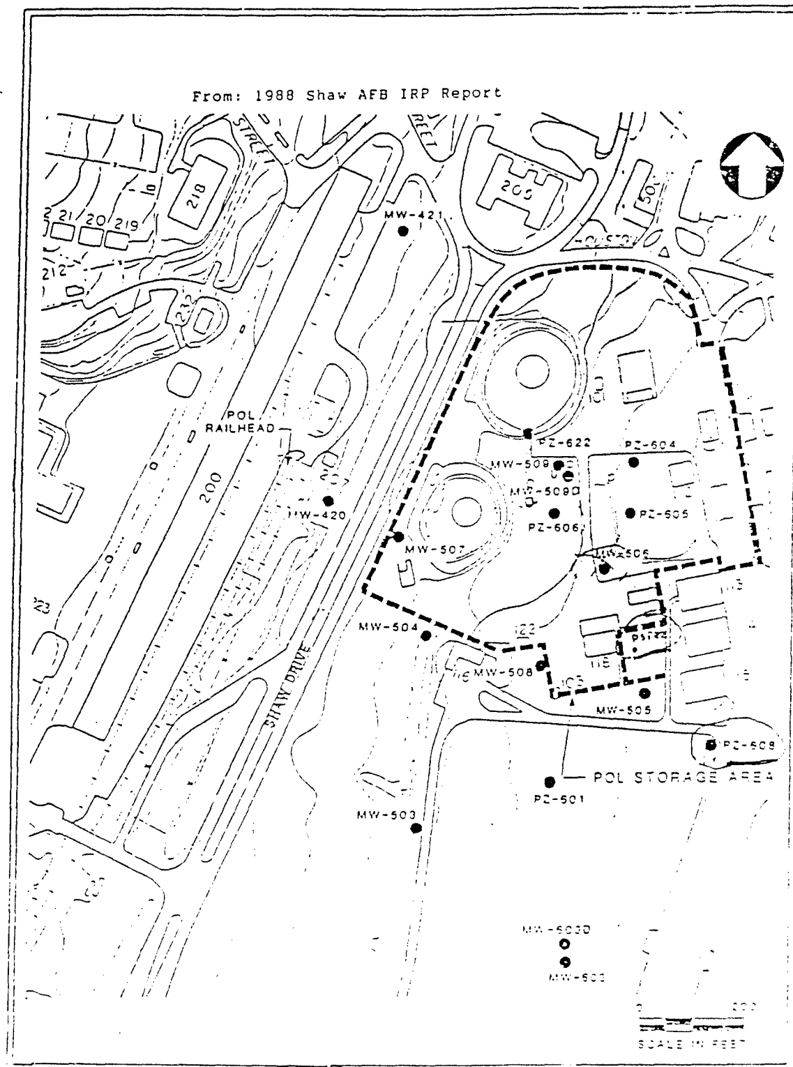
FIGURE A-2 POL STORAGE LOCATION - SHAW
