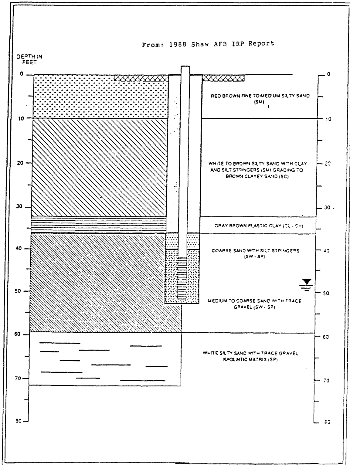
FIGURE A-10 PIEZOMETER PZ601 LOG
