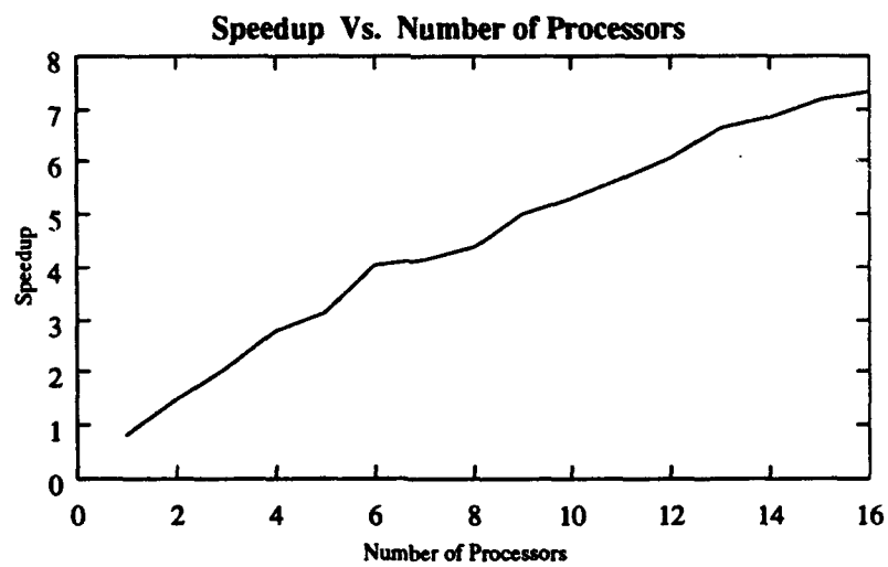
Figure 3: 1000 Point Problem
