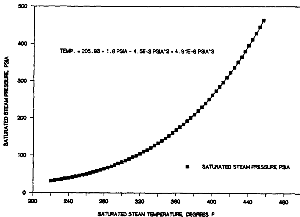
Figure 6. Saturated Steam.
