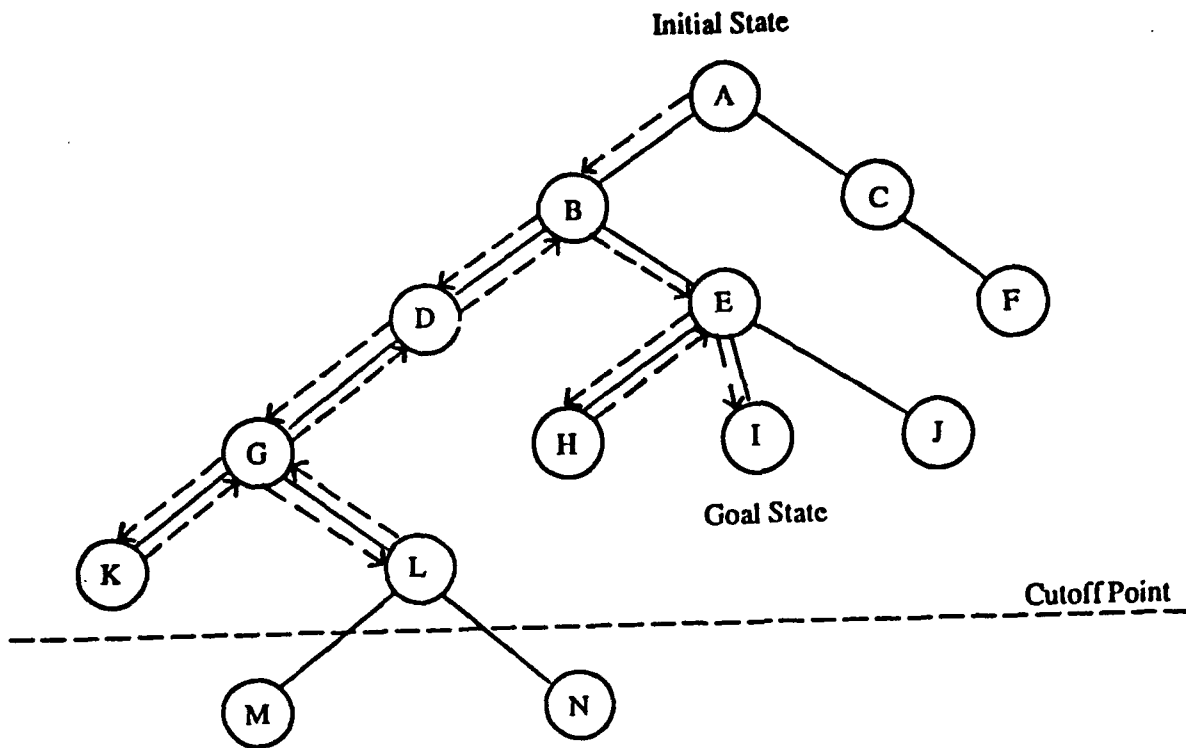
Figure 2. Depth-First Search.
