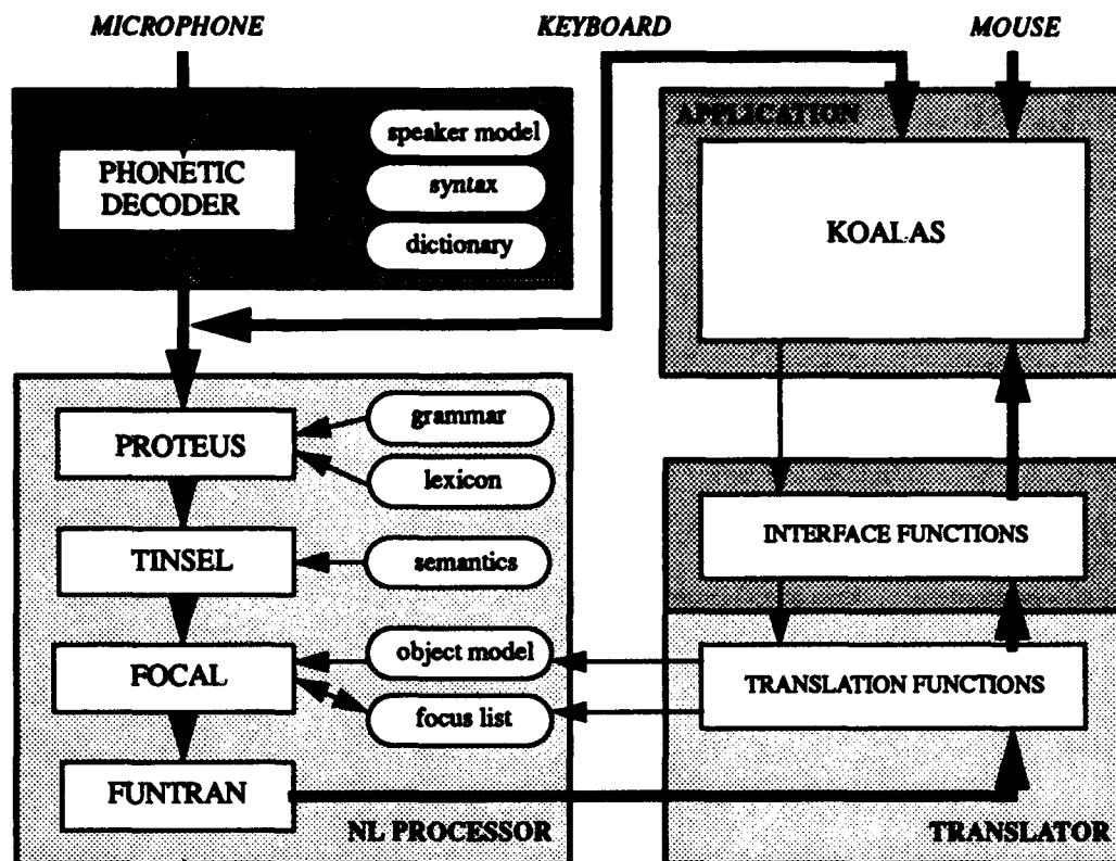
Fig. 2 - Eucalyptus architecture
