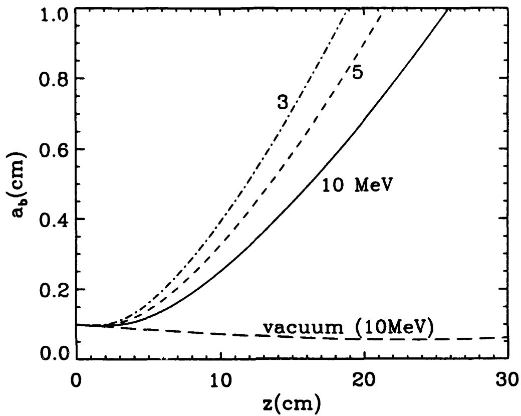
Fig. 2 - Free expansion in air and vacuum for \theta_t = 0.003 , \theta_i = 0.002 , and beam energies of 3, 5, and 10 MeV
