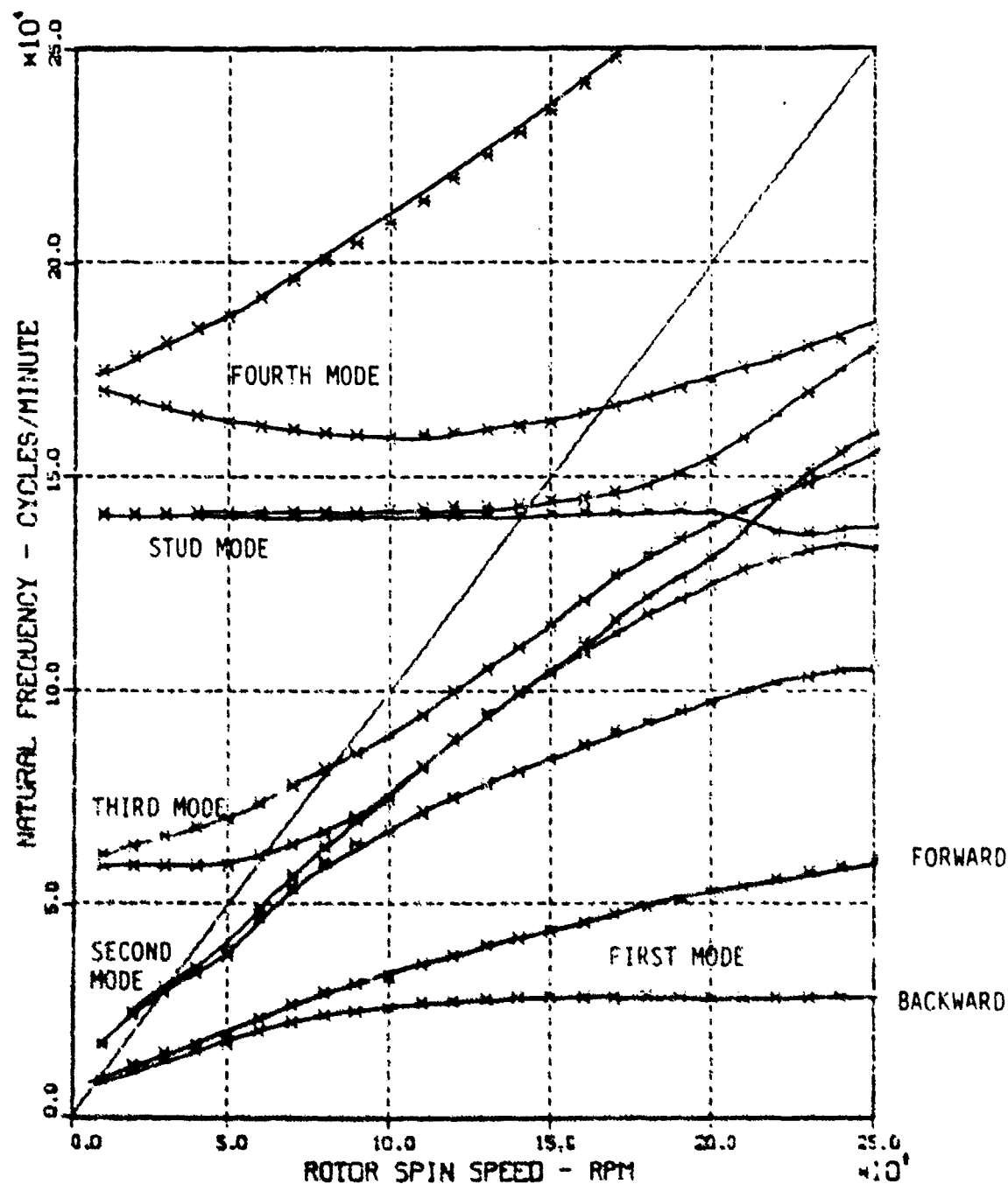
Figure B-3. Rotordynamic Critical Speed Plot
