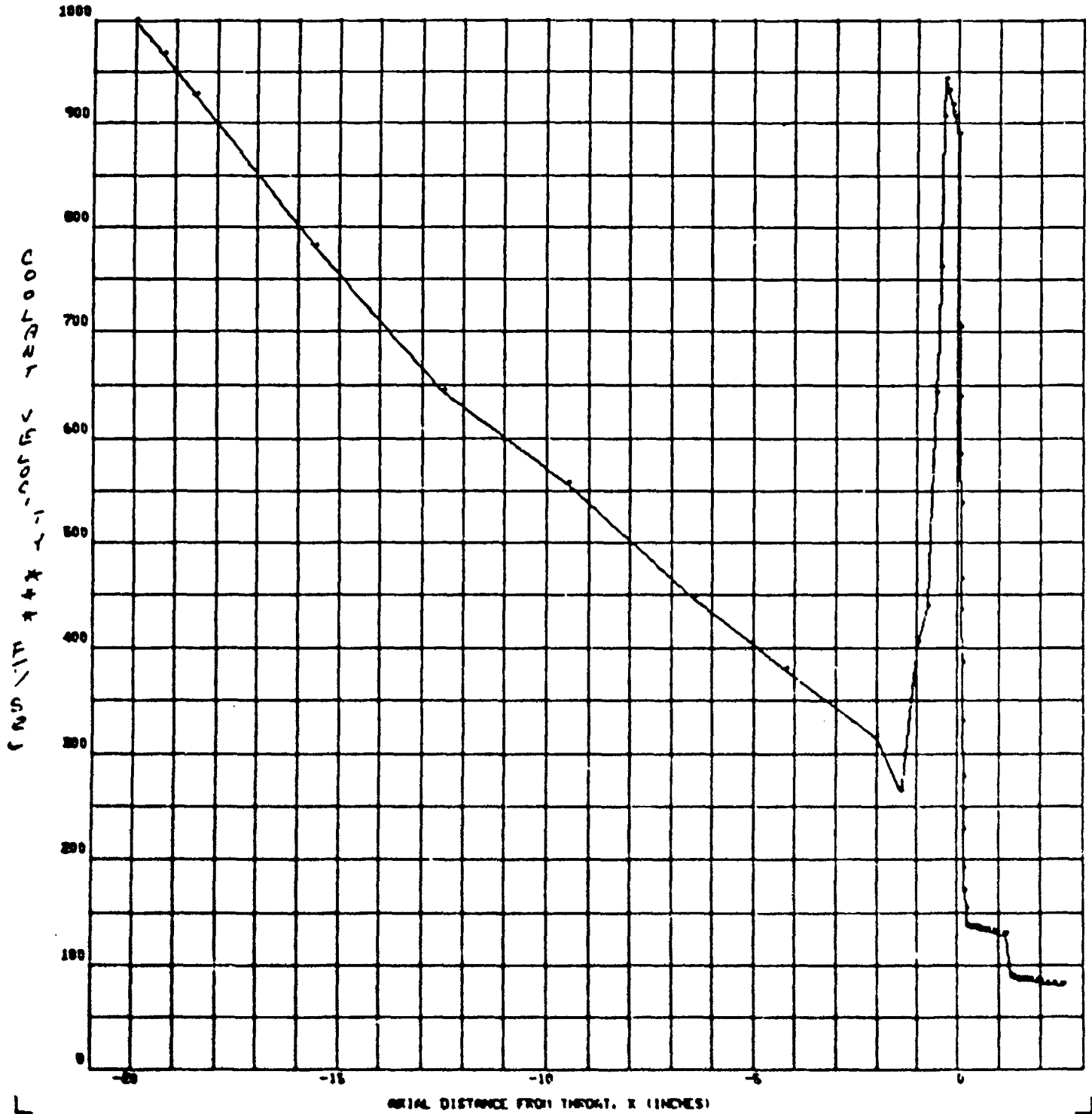
Figure 21. Coolant Velocity Profile
