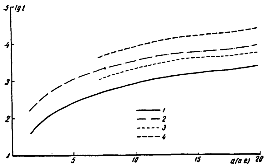
Figure 6. Lifetime of cometary nucleus of \text{C}_2\text{N}_2 ( t in years).
